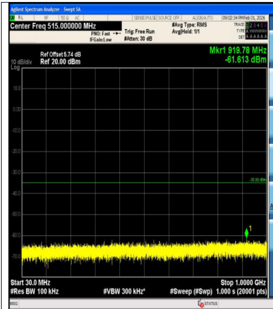
Band7-5MHz-16QAM-21425-25RB#0-3000~180 00-PASS
