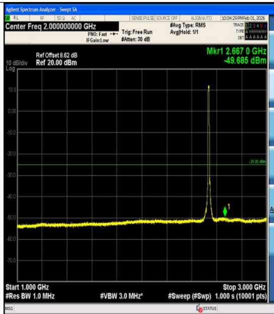
Band7-10MHz-16QAM-21100-50RB#0-18000~27000-PASS
