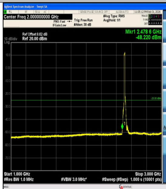
Band7-15MHz-QPSK-20825-75RB#0-18000~27 000-PASS
