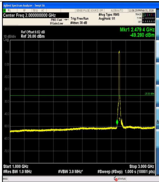
Band7-15MHz-16QAM-20825-75RB#0-18000~27000-PASS
