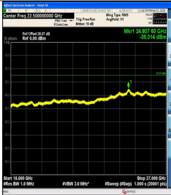
Band7-15MHz-QPSK-21100-1RB#0-0.15~30-PA SS
