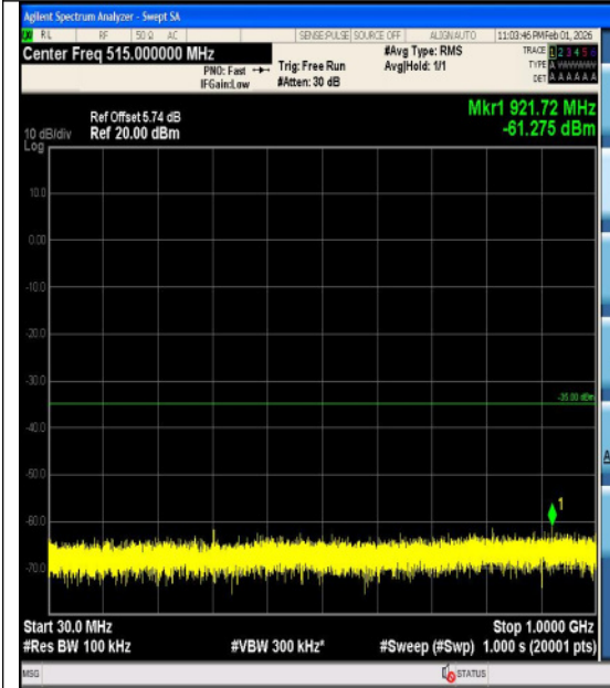
Band7-15MHz-16QAM-20825-1RB#74-3000~18000-PASS
