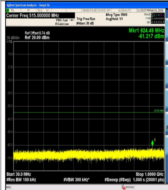
Band7-15MHz-QPSK-21375-1RB#0-3000~1800 0-PASS
