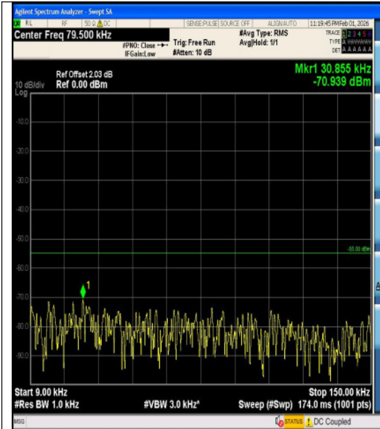
Band7-15MHz-QPSK-21375-75RB#0-30~1000-P ASS
