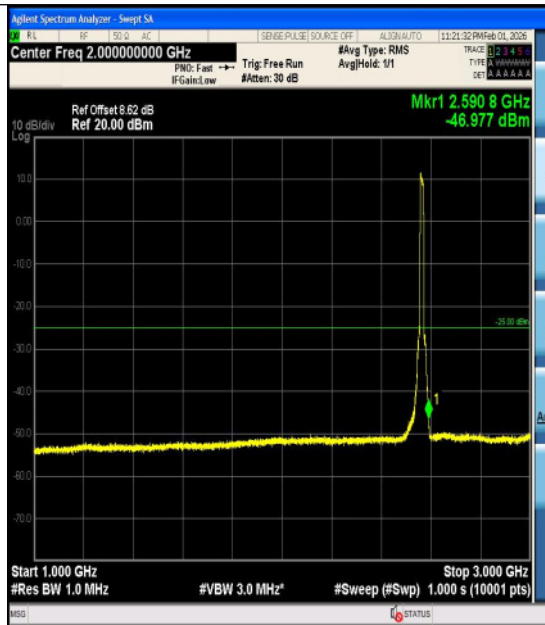
Band7-15MHz-16QAM-21375-75RB#0-18000~27000-PASS
