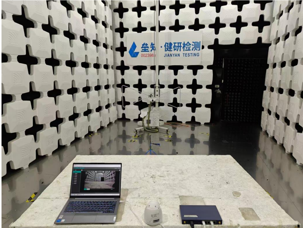
Working mode 1 (AC/DC power adapter) Radiated Spurious Emission Below 1GHz
