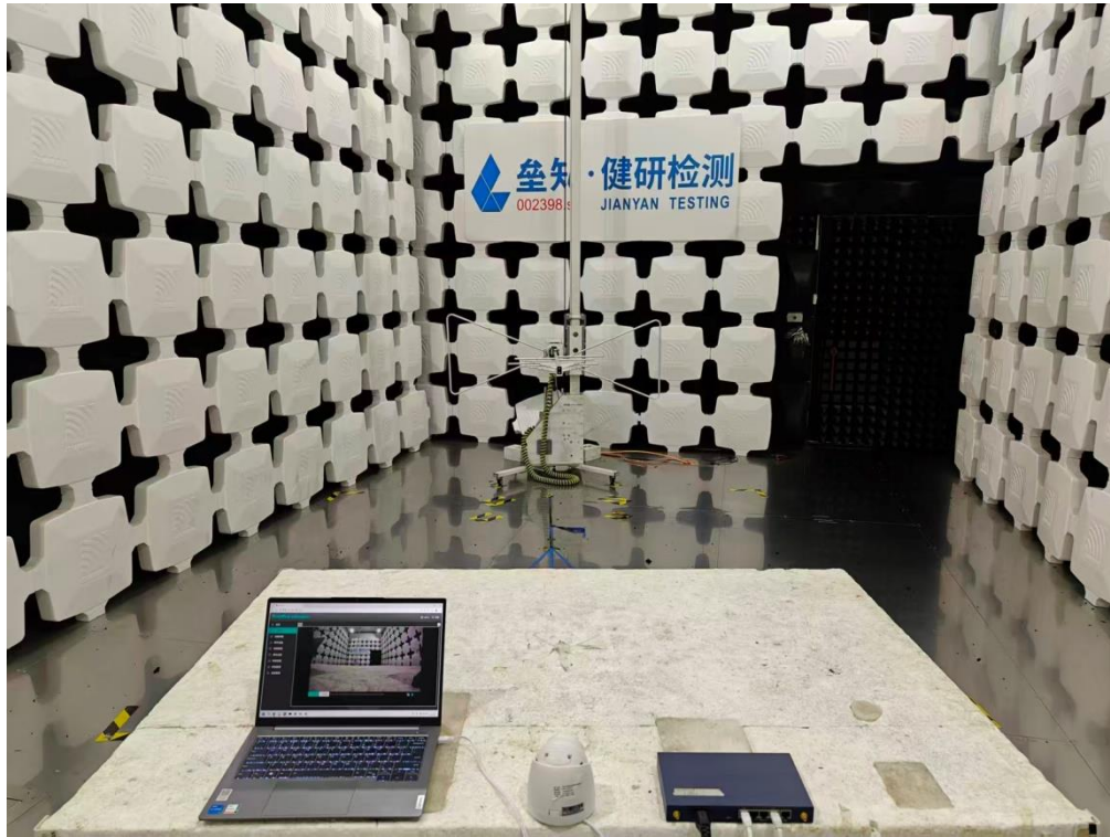
Working mode 2 (Giga PoE Injector) Radiated Spurious Emission Below 1GHz
