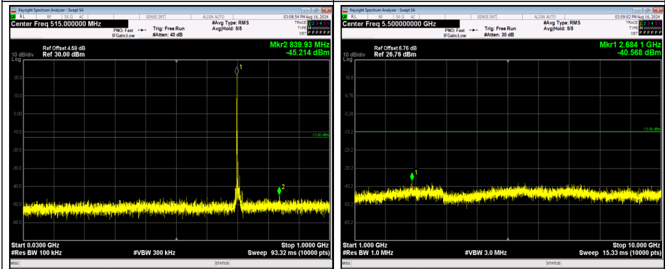
Band17-10MHz-64QAM-23800-1RB#0-Range1:30~1000MHz
