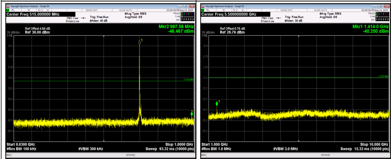
Band17-10MHz-64QAM-23800-1RB#0-Range1:30~1000MHz
