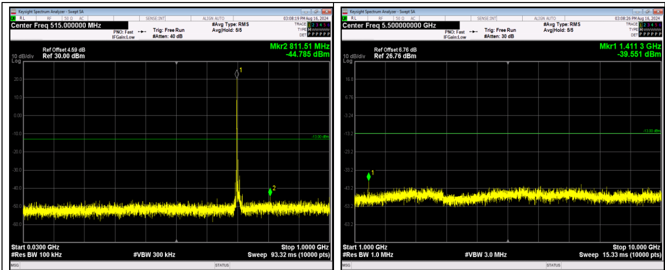
Band17-10MHz-QPSK-23800-1RB#0-Range1:30~1000MHz
