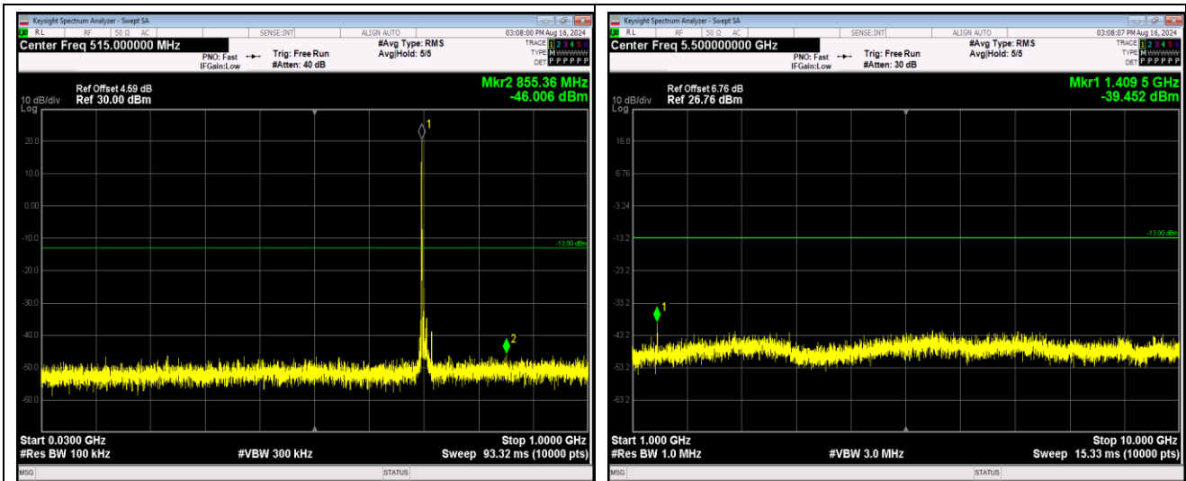
Band17-10MHz-64QAM-23790-1RB#0-Range1:30~1000MHz
