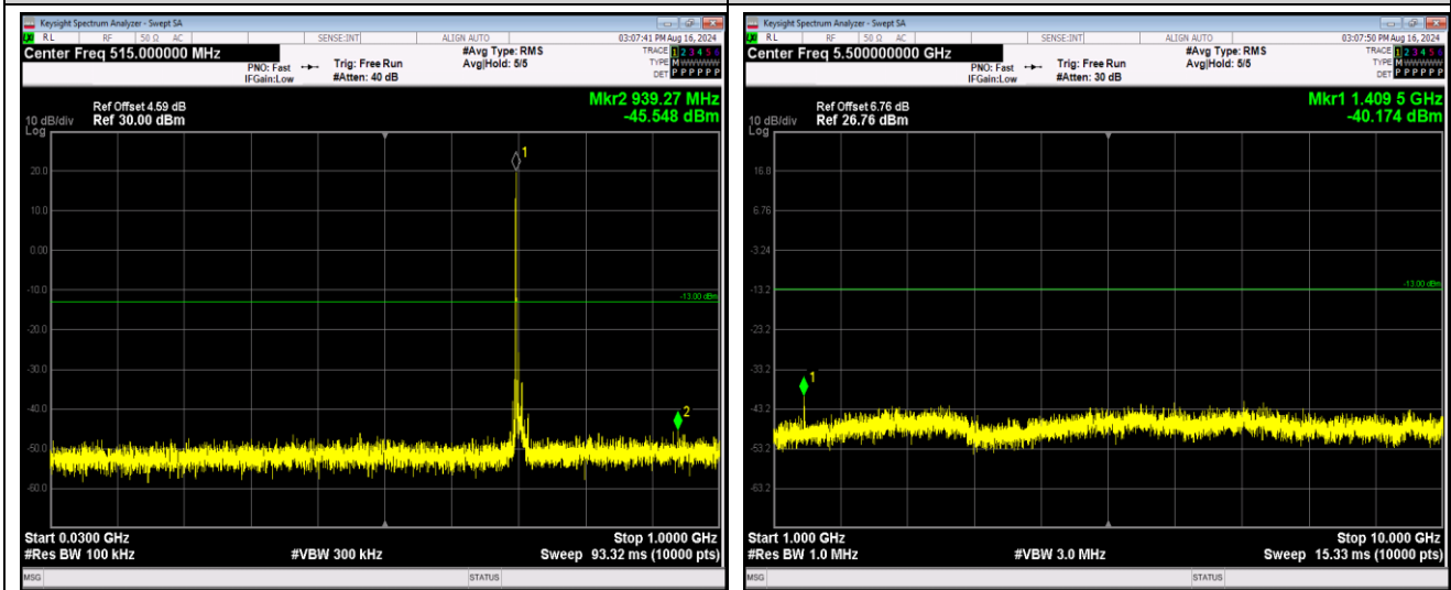
Band17-10MHz-16QAM-23780-1RB#0-Range1:30~1000MHz
