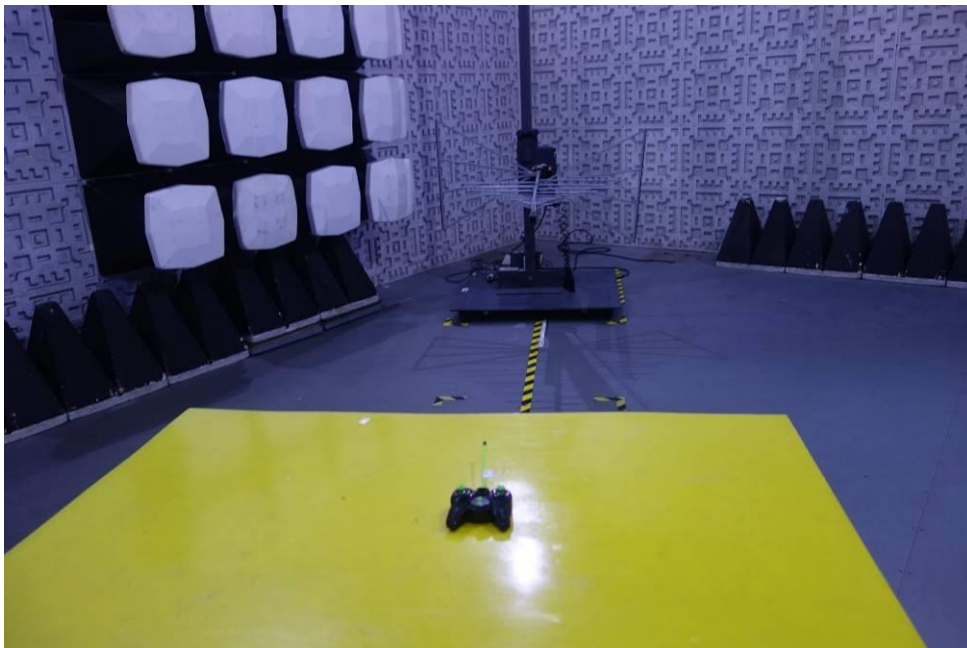
Radiated Emissions
