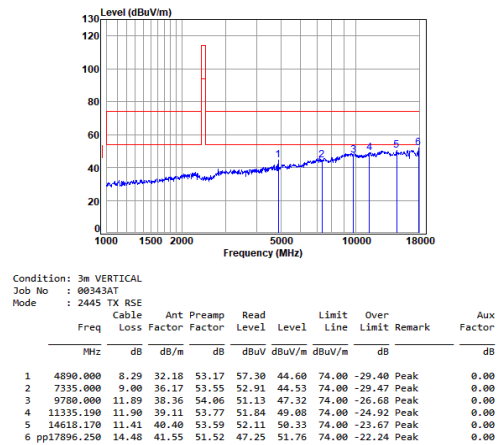
2.4G_SRD_MID_TX_Vertical
