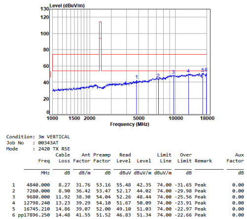
2.4G_SRD_LOW_TX_Vertical
