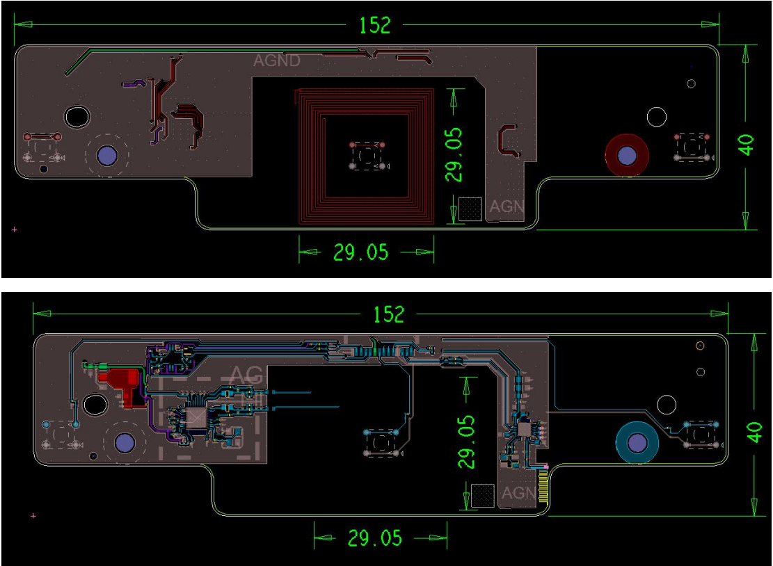
Antenna size diagram
