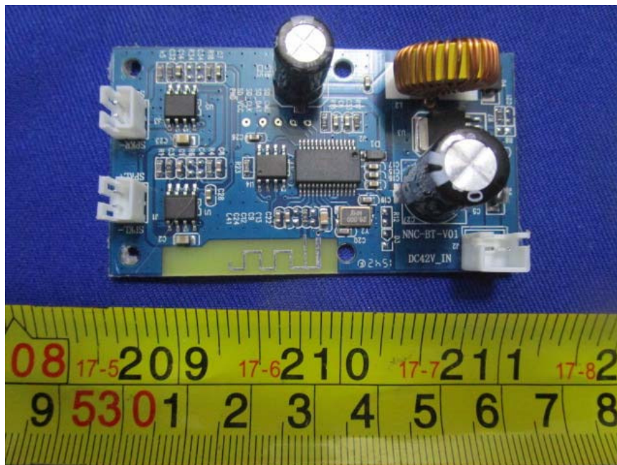
EUT –PCB Board4 Top View
