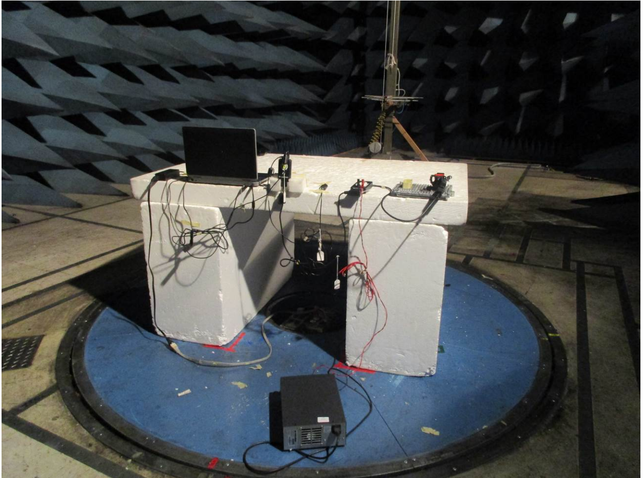
Figure 4: Radiated Emissions – Back View – below 1 GHz
