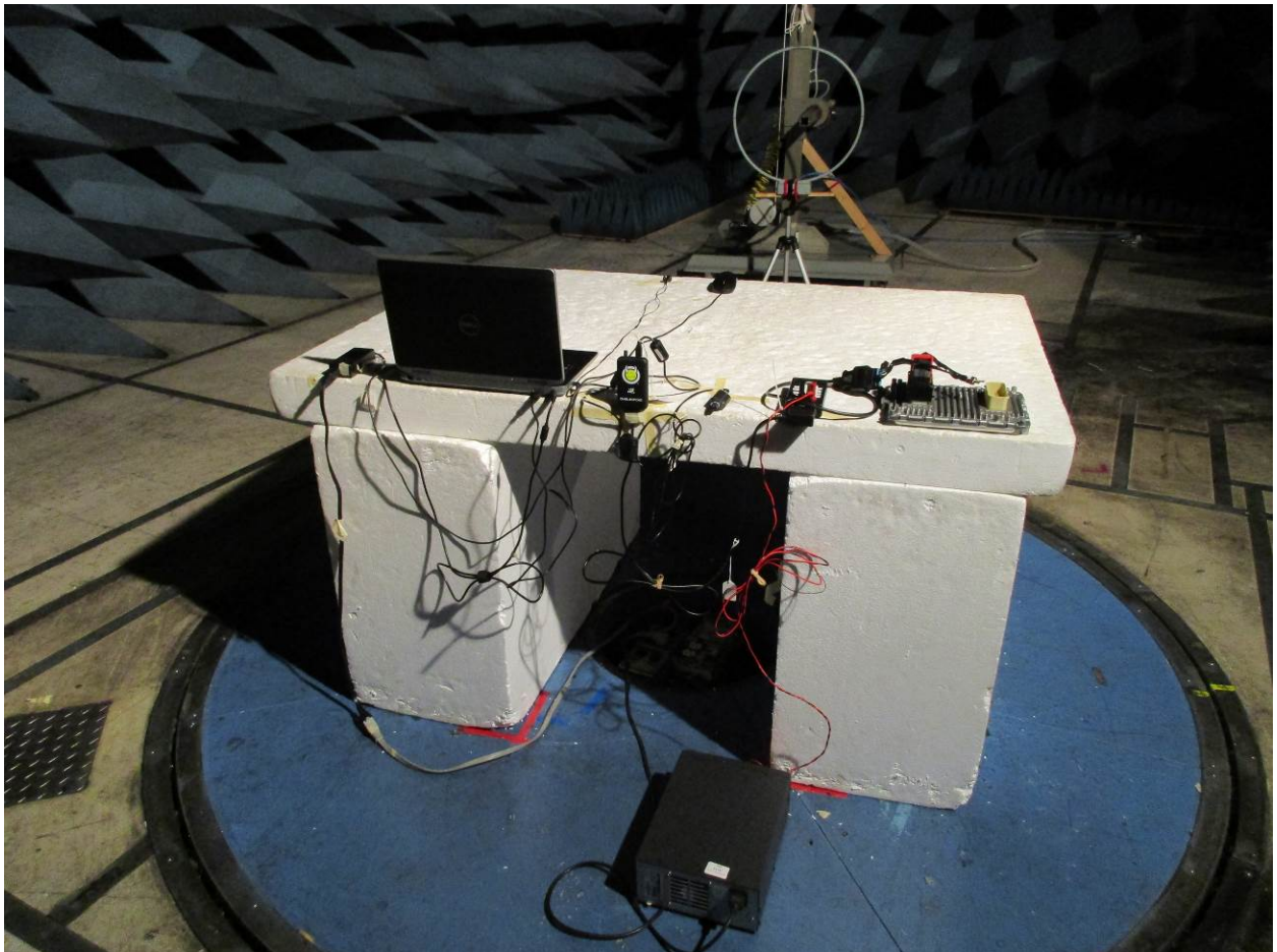
Figure 2: Radiated Emissions – Back View – below 1 GHz
