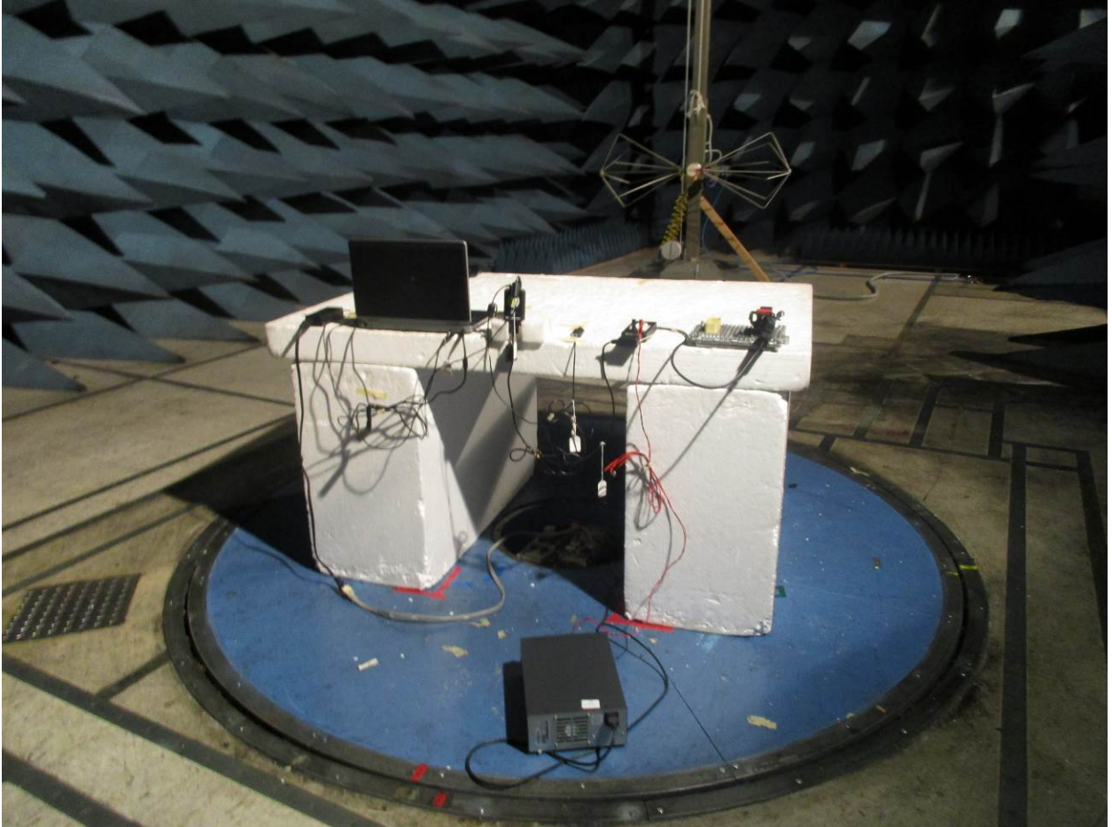
Figure 3: Radiated Emissions – Back View – below 1 GHz
