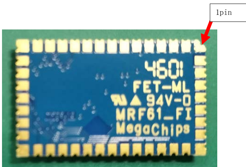
Picture 3-3 MRF61_FI_F1/TH Bottom view
