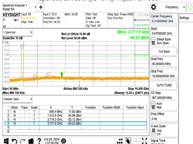
Spurious Emission_OFDM_4M_LowCH-906
