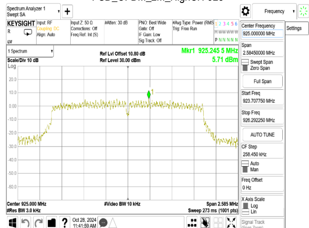
PSD_OFDM_2M_HighCH-925
