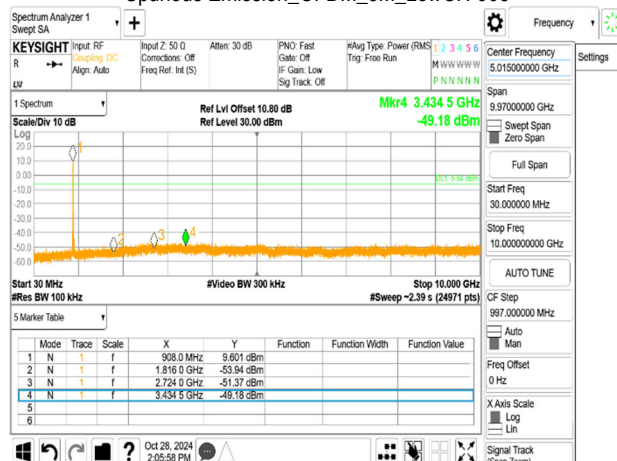
Spurious Emission_OFDM_8M_LowCH-908
