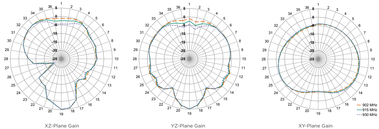
Figure 8. ANT-916-CW-RCS-ccc Radiation Patterns
