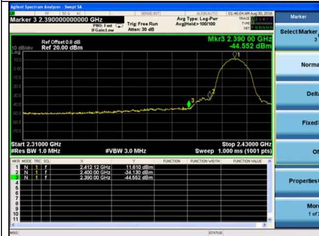
2412 MHz – Peak
