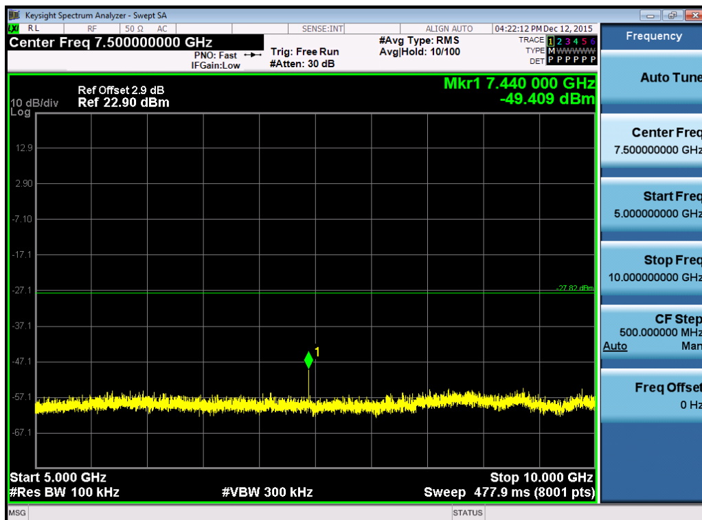
(Plot 4.6.1 C4: Channel 39: 2480MHz @ GFSK)
