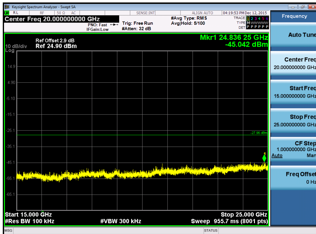
(Plot 4.6.1 A6: Channel 00: 2402MHz @ GFSK)
