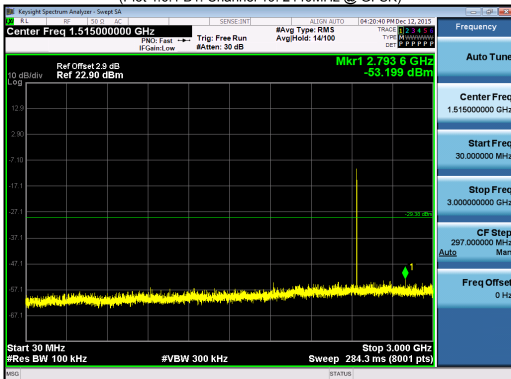
(Plot 4.6.1 B2: Channel 19: 2440MHz @ GFSK)
