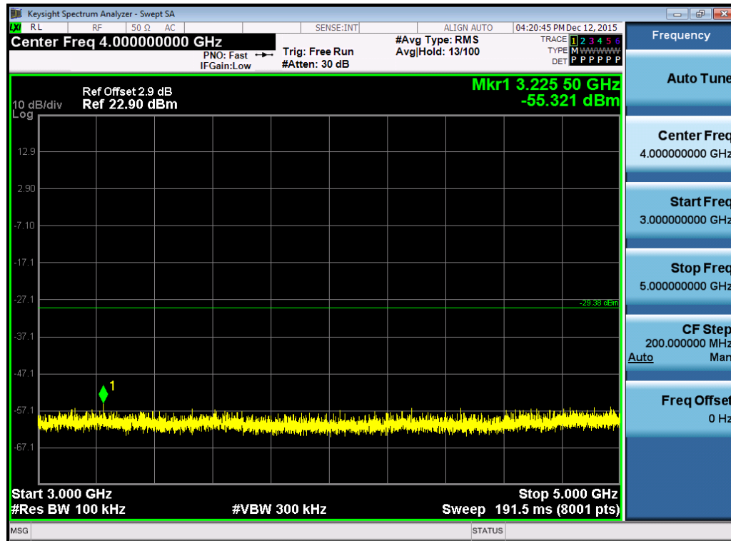
(Plot 4.6.1 B3: Channel 19: 2440MHz @ GFSK)
