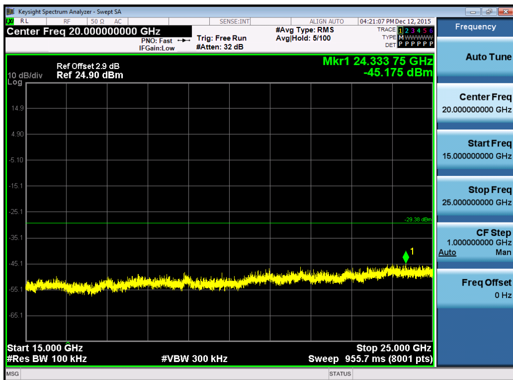
(Plot 4.6.1 B6: Channel 19: 2440MHz @ GFSK)
