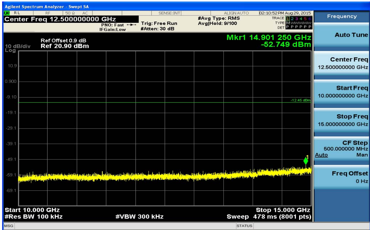
(Plot 4.6.1 A5: Channel 00: 2402MHz @ GFSK)
