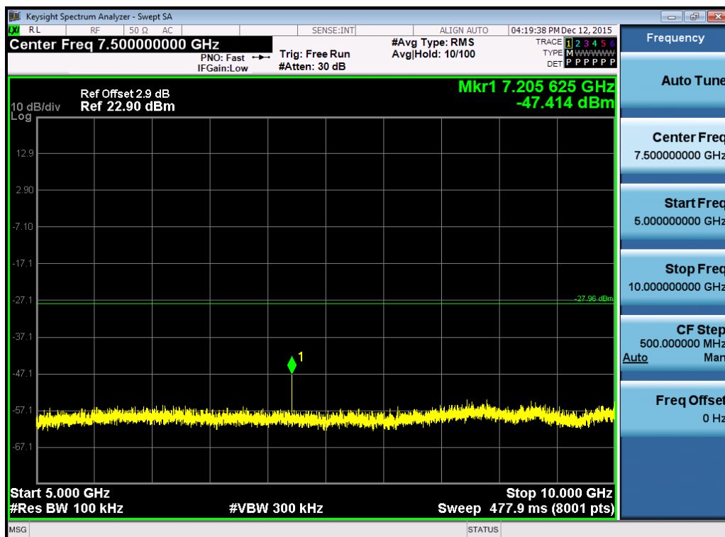
(Plot 4.6.1 A4: Channel 00: 2402MHz @ GFSK)
