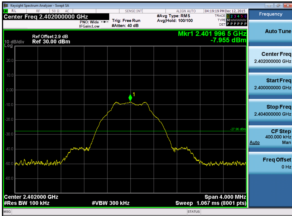
(Plot 4.6.1 A1: Channel 00: 2402MHz @ GFSK)
