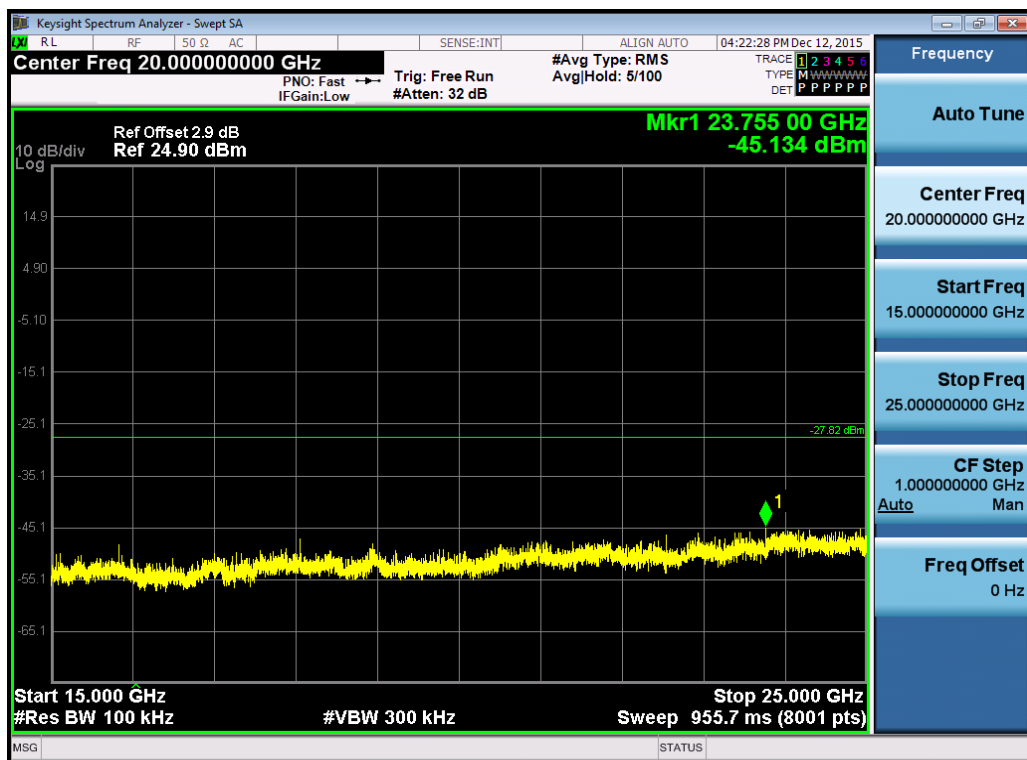
(Plot 4.6.1 C6: Channel 39: 2480MHz @ GFSK)
