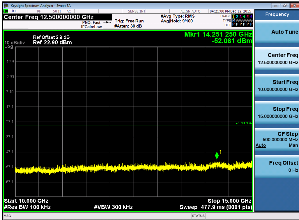
(Plot 4.6.1 B5: Channel 19: 2440MHz @ GFSK)
