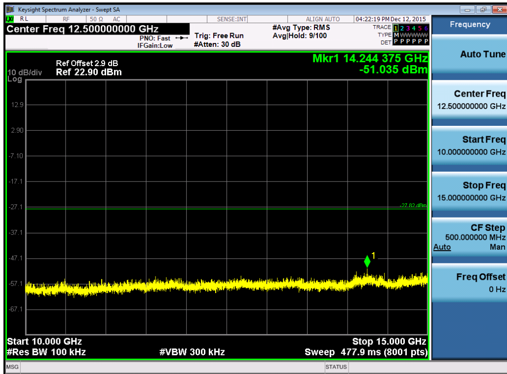
(Plot 4.6.1 C5: Channel 39: 2480MHz @ GFSK)
