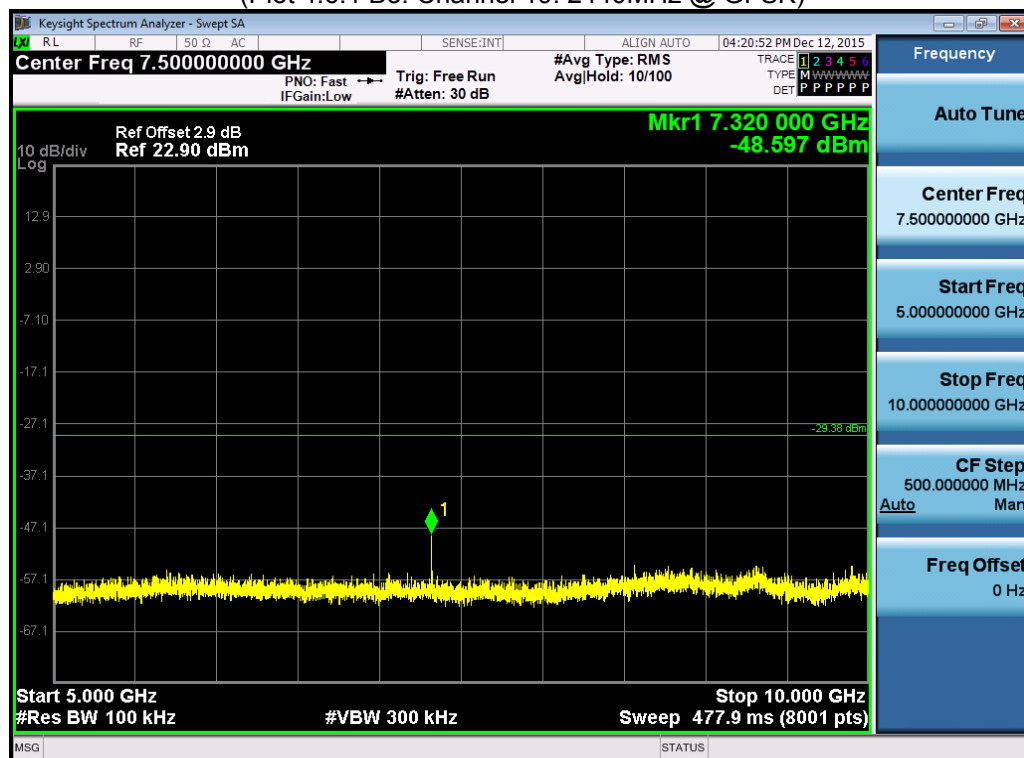
(Plot 4.6.1 B4: Channel 19: 2440MHz @ GFSK)
