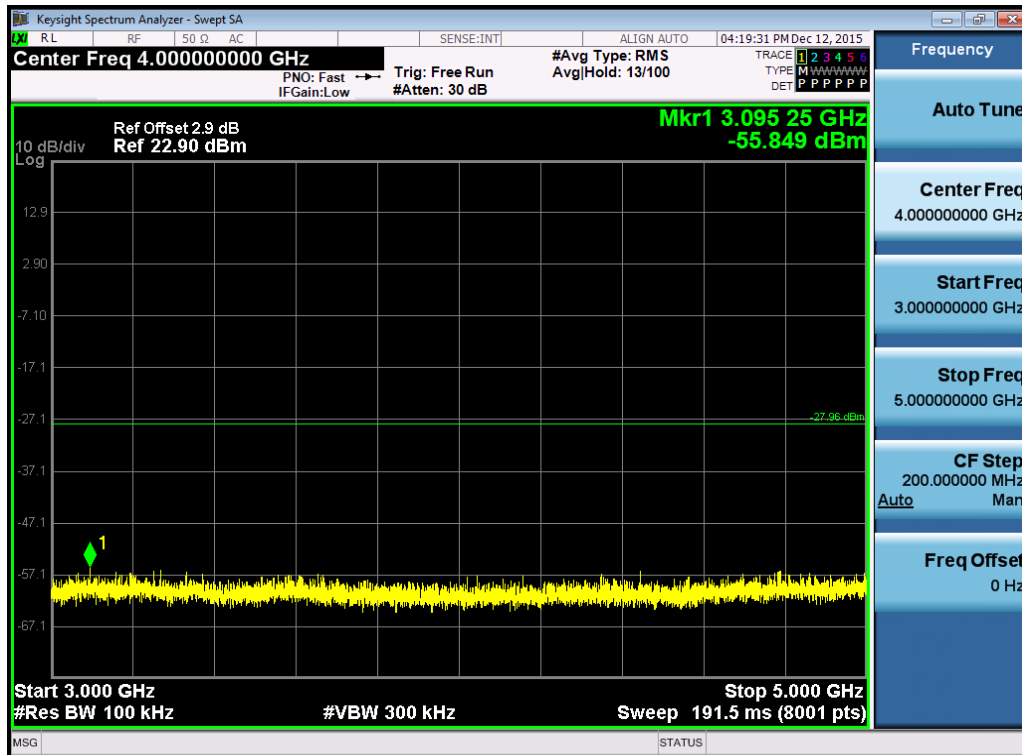
(Plot 4.6.1 A3: Channel 00: 2402MHz @ GFSK)
