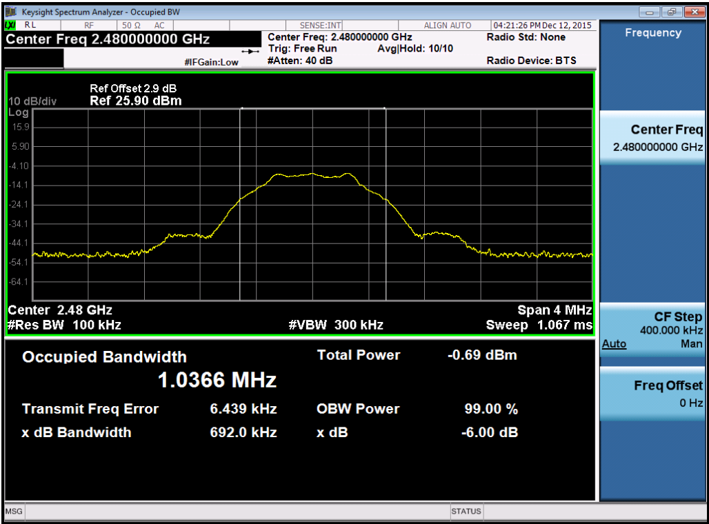
(Plot 4.7.1 C: Channel 39: 2480MHz @ GFSK)
