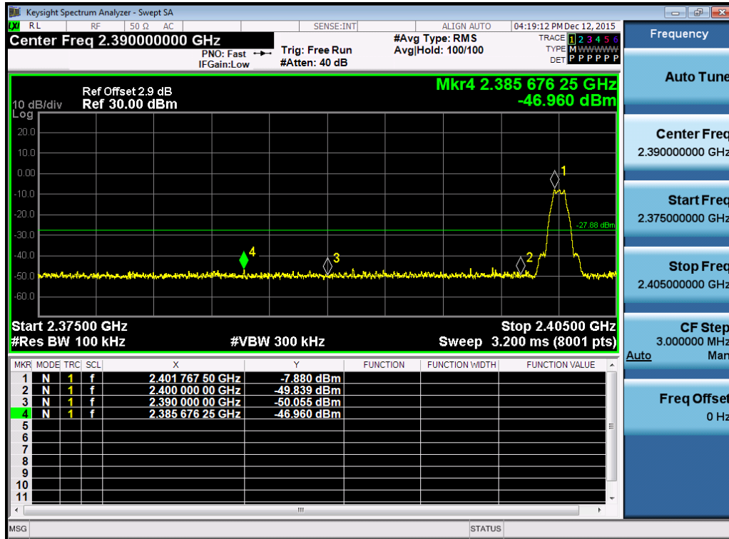
(Plot 4.5.2.1 A: Channel 00: 2402MHz @ GFSK)
