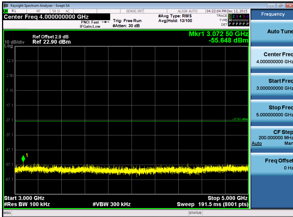
(Plot 4.6.1 C3: Channel 39: 2480MHz @ GFSK)
