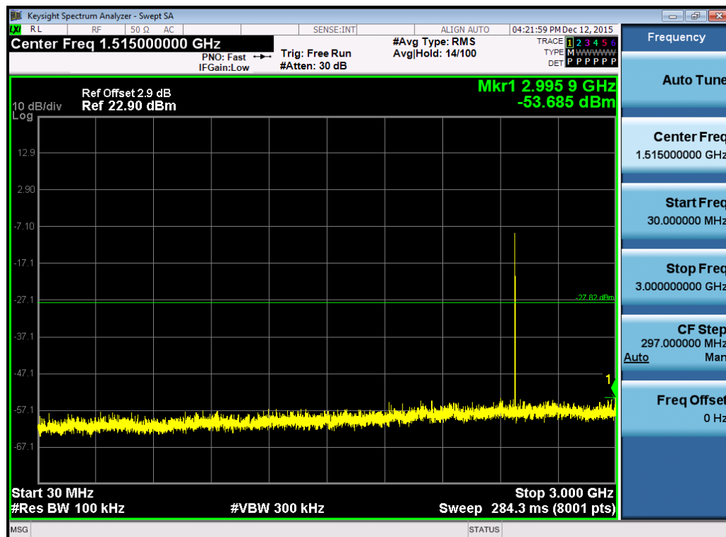
(Plot 4.6.1 C2: Channel 39: 2480MHz @ GFSK)
