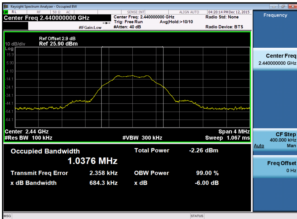
(Plot 4.7.1 B: Channel 19: 2440MHz @ GFSK)
