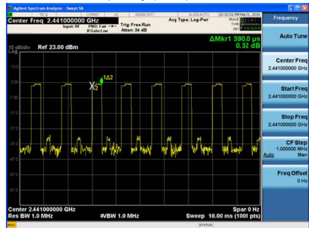
Carrier frequency (MHz): 2441, 2DH3
