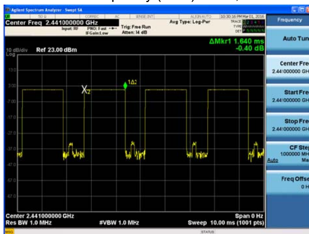
Carrier frequency (MHz): 2441, DH5
