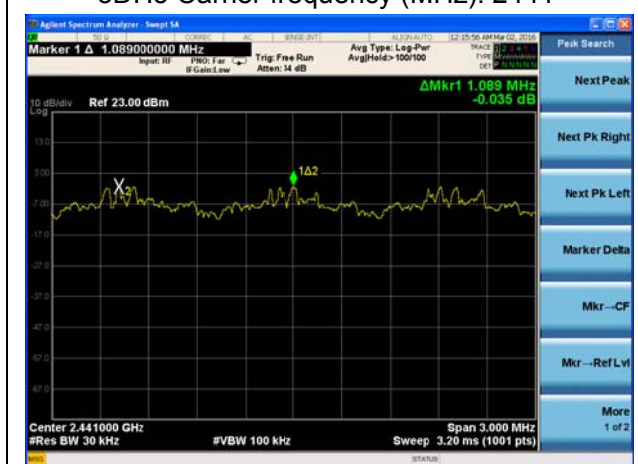
3DH5 Carrier frequency (MHz): 2441
