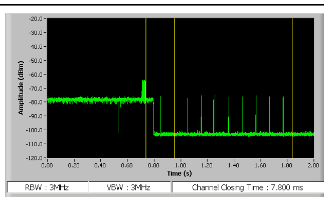
Channel Closing Time - 5500MHz (Type0)
