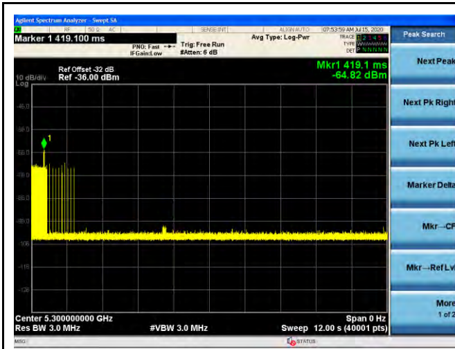
Channel Move Time - 5300MHz (Type0)
