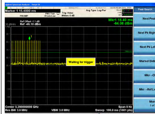
Radar Type 0 @ 5290MHz
