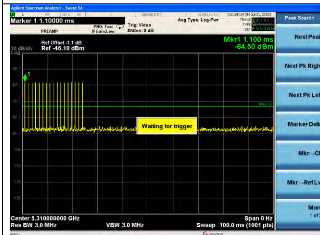
Radar Type 0 @ 5310MHz
