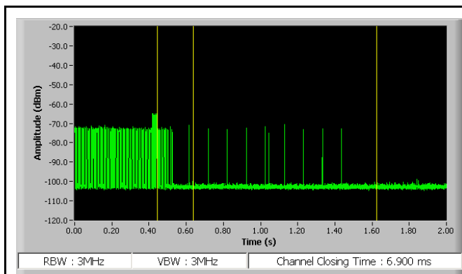
Channel Closing Time - 5300MHz (Type0)
