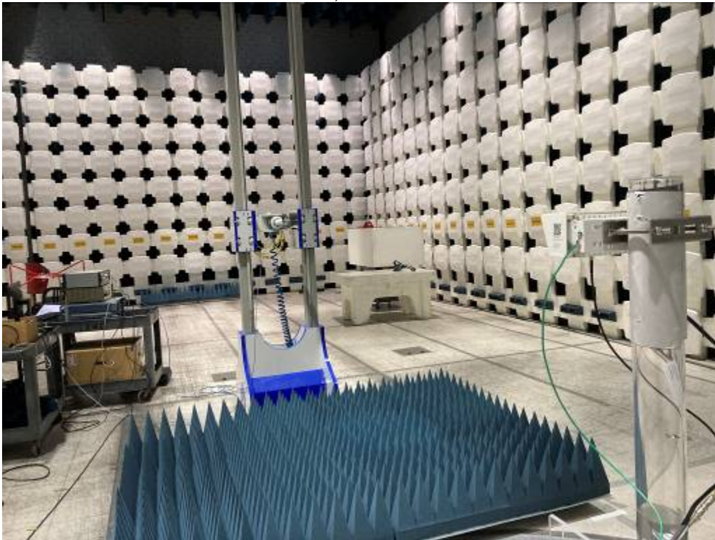
Scan, 18-26 GHz
