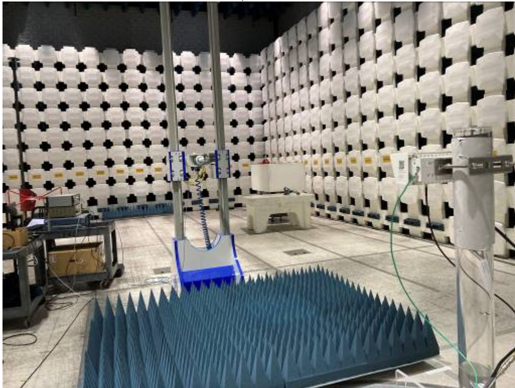
Scan, 18-40 GHz
