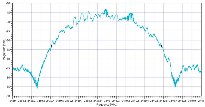
Plot_FCC Part 15.247 Bandwidth 99PCT-20dB ~ BT LE 1 Msps 20dB_21082019_164406.png
