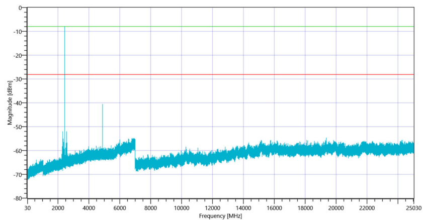
Plot_FCC Part 15.247 TX Spurious Conducted ~ BT LE 1 Msps 2440_21082019_165425.png
