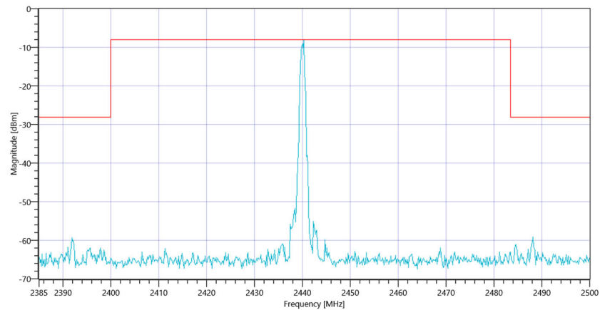
Plot_FCC Part 15.247 TX Spurious Conducted ~ BT LE 1 Msps 2440_21082019_165427.png
