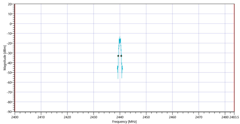
Plot_FCC Part 15.247 Bandwidth 99PCT-20dB ~ BT LE 1 Msps_21082019_164409.png
