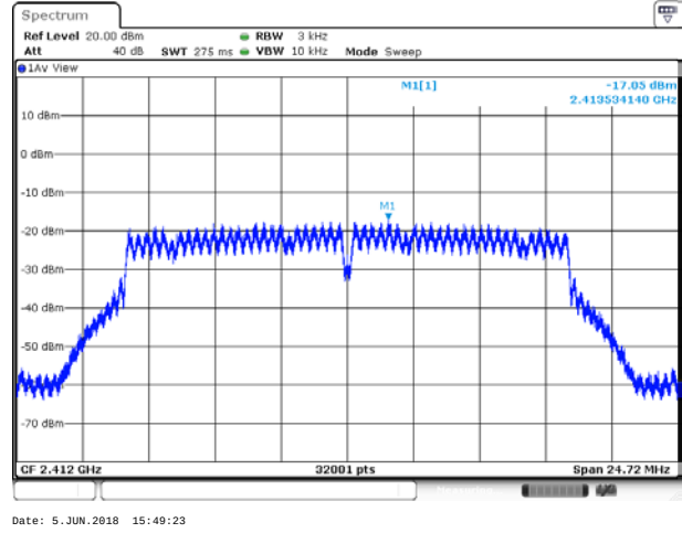
(802.11g) PSD plot on channel 1
