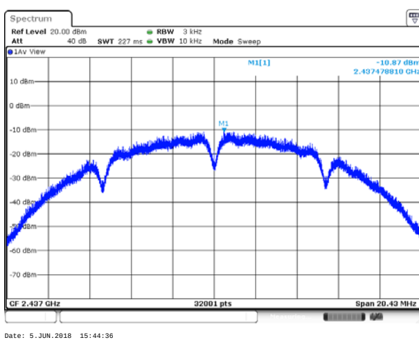
(802.11b) PSD plot on channel 6
