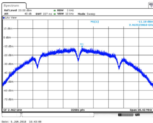
(802.11b) PSD plot on channel 11
