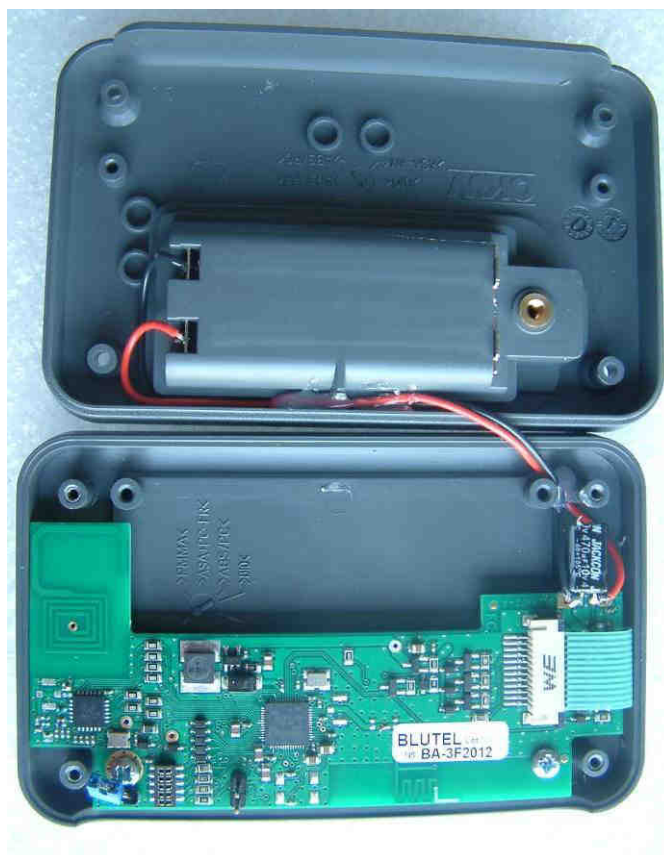
Cover Removed
