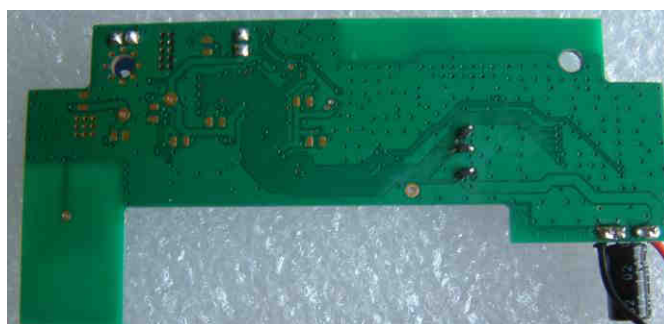
PCB view
