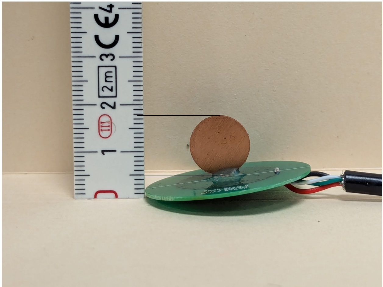
Antenna is a round disc approximately 1.3 cm in diameter
