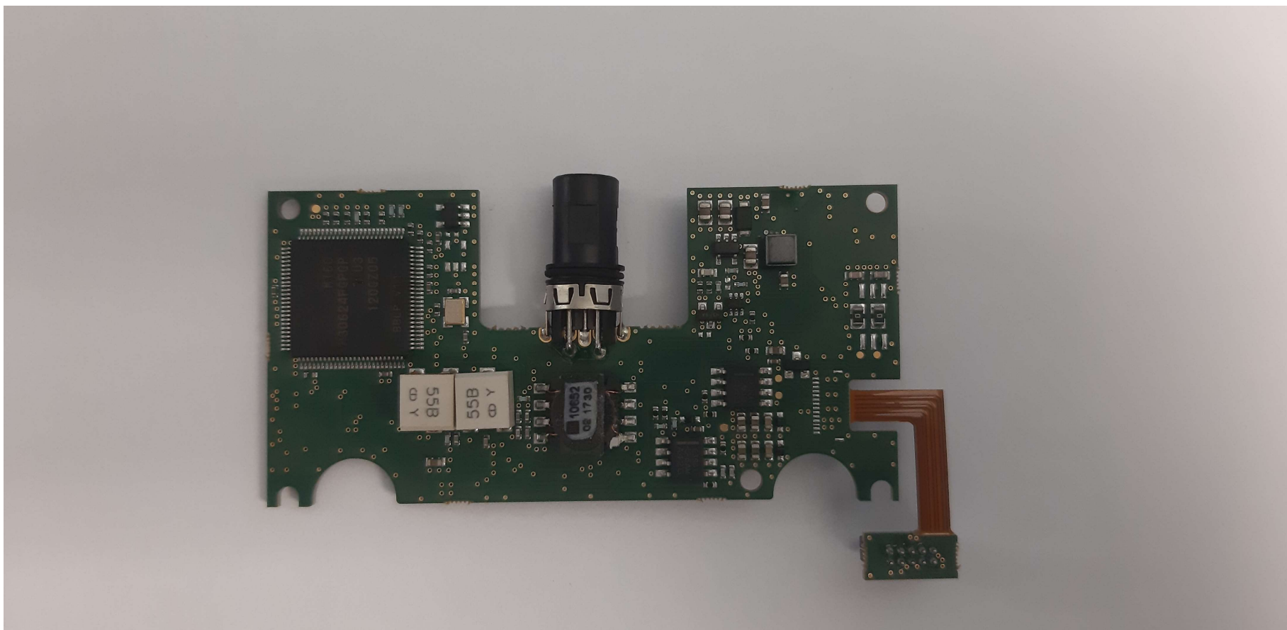
MODEL: BF-IDC02: Internal Photos (PCB Top)
