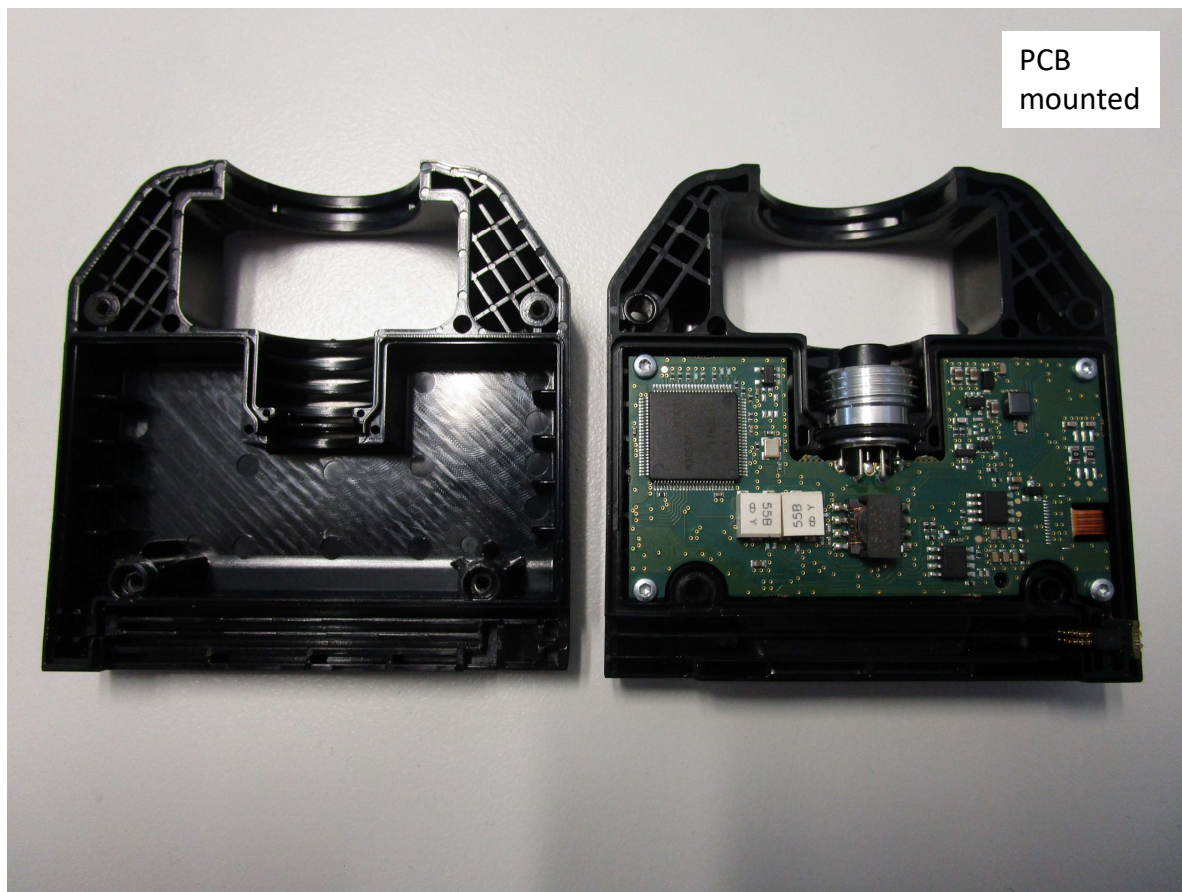
MODEL: BF-IDC02: Internal Photos (Mounting situation)
