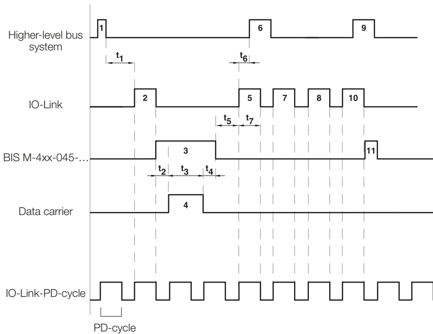
Fig. 7-4: Timing of IO-Link transmission
