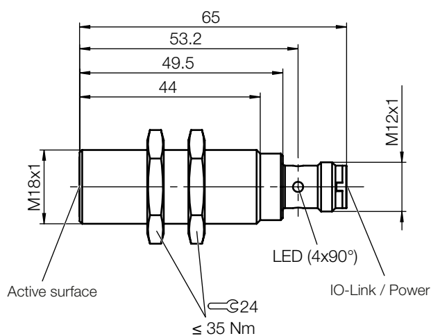
Fig. 4-3: Dimensions and design of BIS M-4A6...
