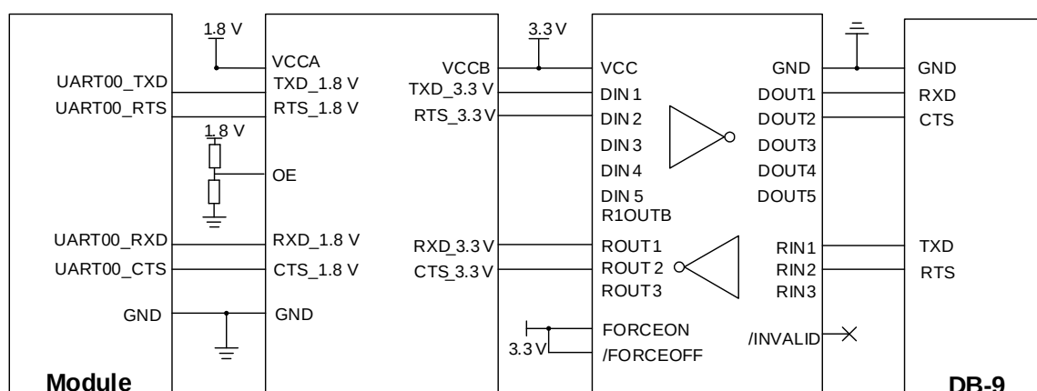
Figure 20: Reference Design of UART with RS-232 Level-shifting Chip (for UART0)
