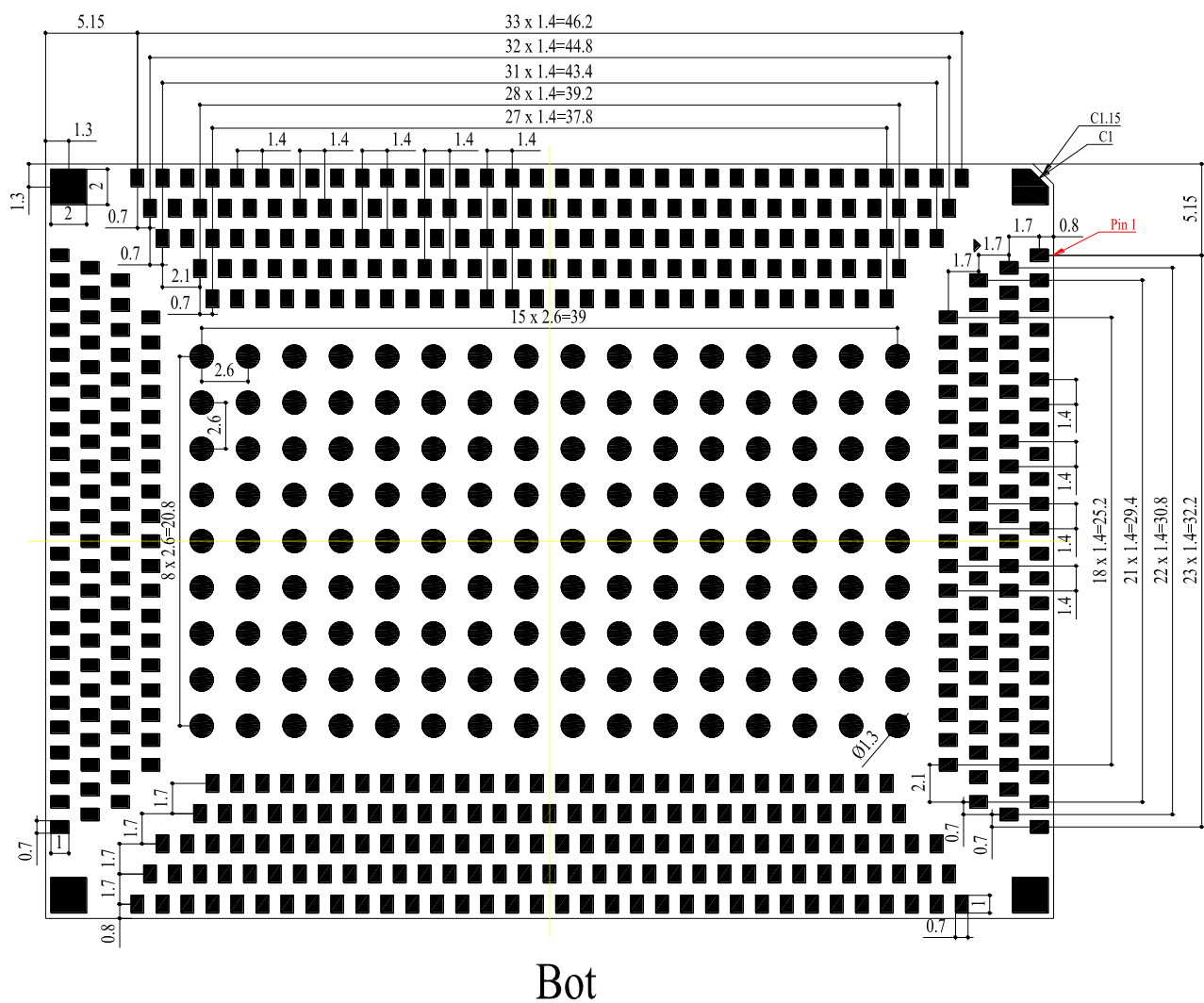
Figure 38: Module Bottom Dimensions (Bottom View)
