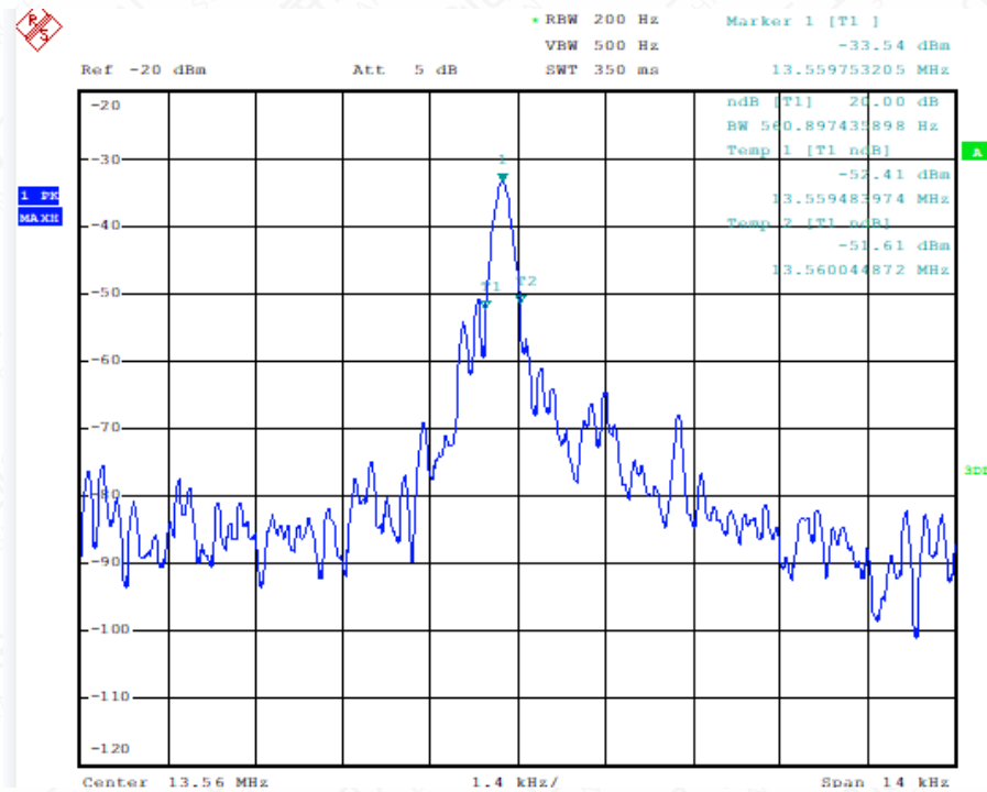
Figure A.1-1 Mode 1 20dB Bandwidth
