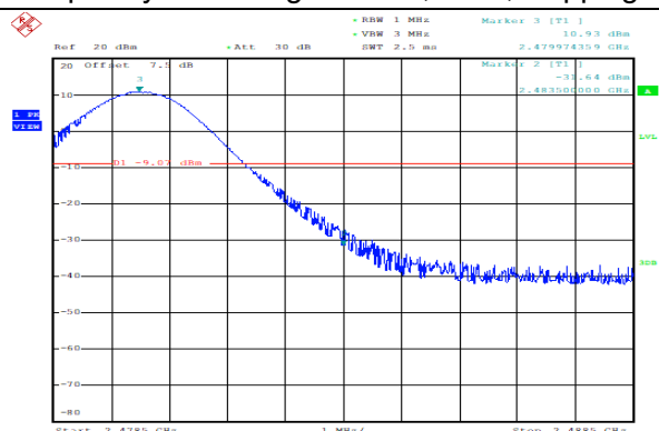
Frequency Band Edge: GFSK, Ch78, Hopping OFF
