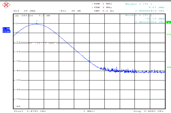
Frequency Band Edge: 8DPSK, Ch78, Hopping OFF
