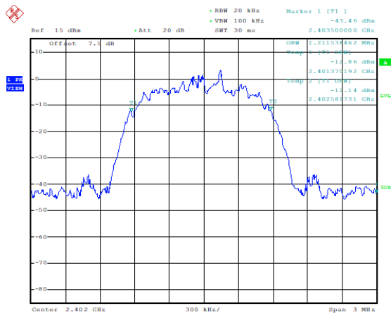
99% Bandwidth: 8DPSK, Ch0
