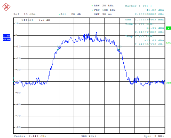
99% Bandwidth: DQPSK, Ch39
