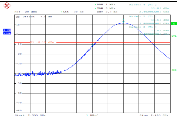
Frequency Band Edge: GFSK, Ch0, Hopping OFF
