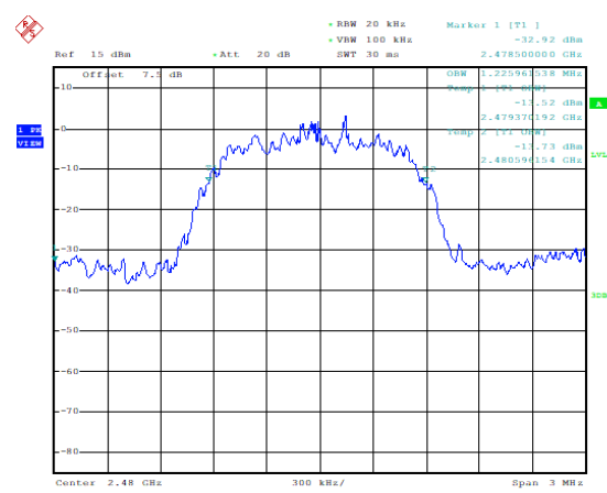
99% Bandwidth: DQPSK, Ch78
