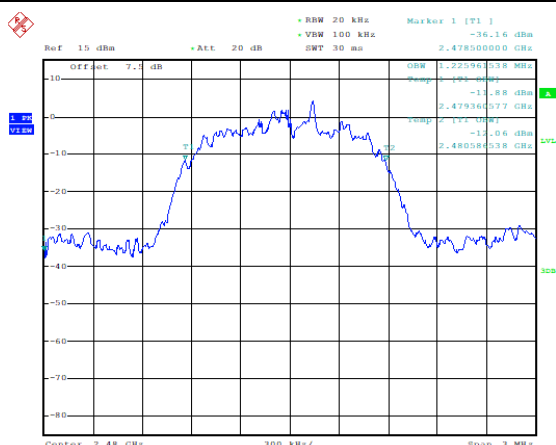
99% Bandwidth: 8DPSK, Ch78
