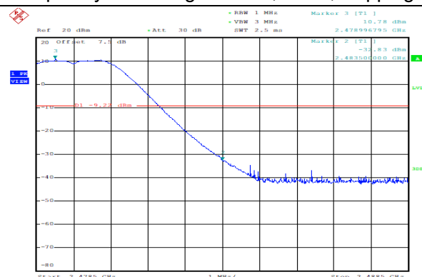
Frequency Band Edge: GFSK, Ch78, Hopping ON
