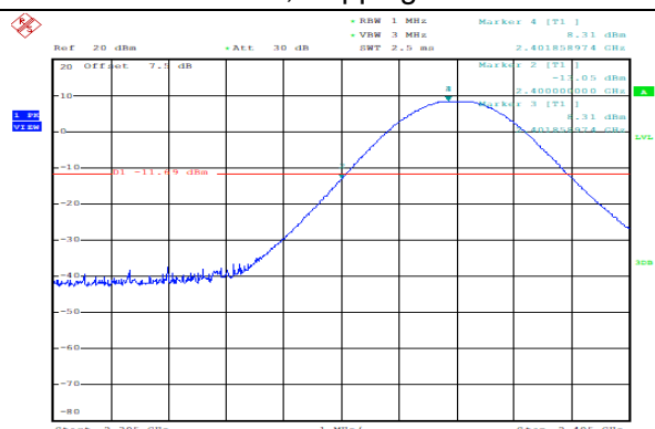
Frequency Band Edge: \pi/4 DQPSK, Ch0, Hopping OFF
