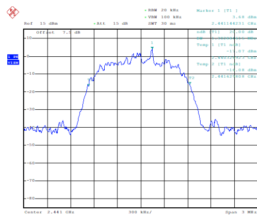
20dB Bandwidth: 8DPSK, Ch39
