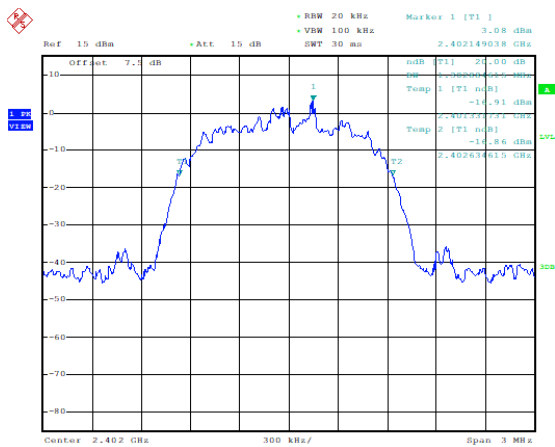
20dB Bandwidth: 8DPSK, Ch0
