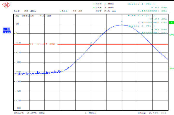
Frequency Band Edge: 8DPSK, Ch0, Hopping OFF
