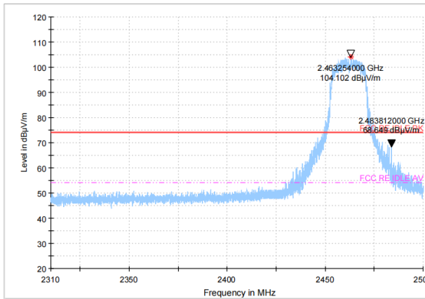
Peak detector
