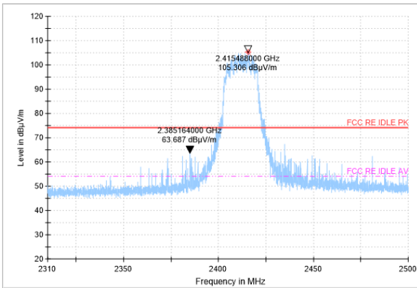
Peak detector
