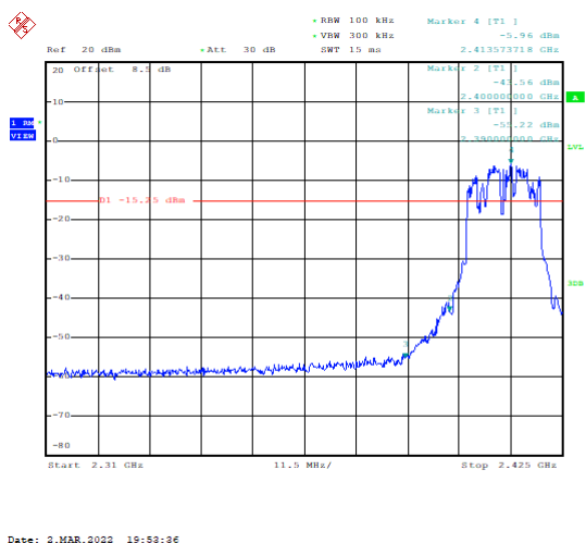
Band Edges (802.11n-20MHz, Ch1)
