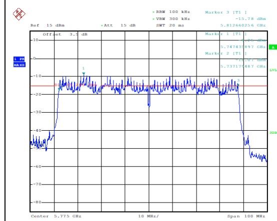
Occupied 6dB Bandwidth ( MHz) (802.11ac-VHT80), 5775MHz)
