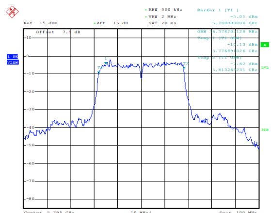
99% Occupied Bandwidth ( MHz) (802.11n-HT40), 5795MHz)
