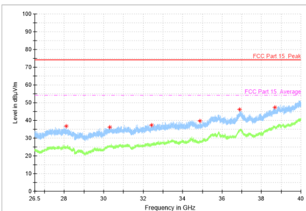
Radiated Spurious Emission (802.11n-HT40, ch151, 26.5GHz-40GHz)
