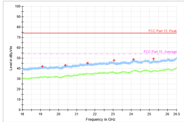
Radiated Spurious Emission (802.11n-HT40, ch151, 18GHz-26.5GHz)
