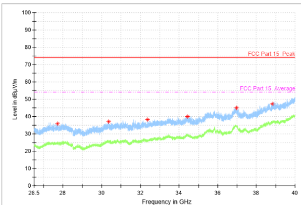
Radiated Spurious Emission (802.11n-HT20, ch165, 26.5GHz-40GHz)
