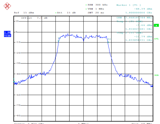
99% Occupied Bandwidth ( MHz) (802.11n-HT20), 5825MHz)
