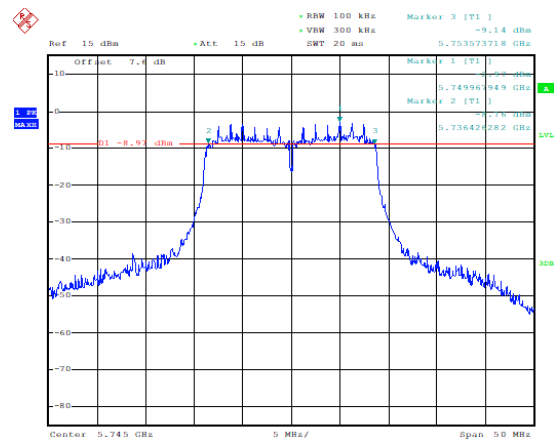
Occupied 6dB Bandwidth ( MHz) (802.11n-HT20), 5745MHz)
