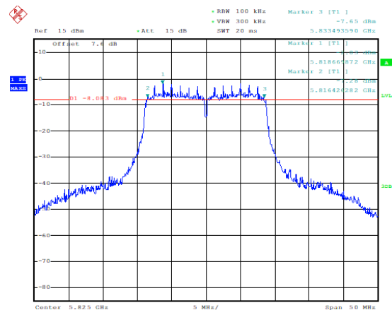
Occupied 6dB Bandwidth ( MHz) (802.11n-HT20), 5825MHz)
