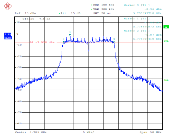
Occupied 6dB Bandwidth ( MHz) (802.11ac-VHT20, 5785MHz)
