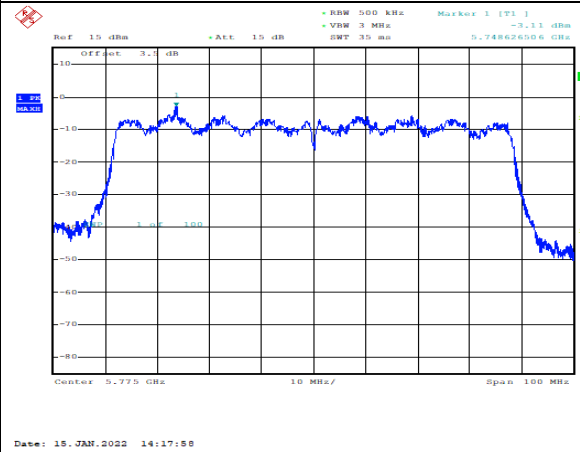
U-NII-3 Power spectral density-802.11 ac(VHT80),5775MHz,Ant1
