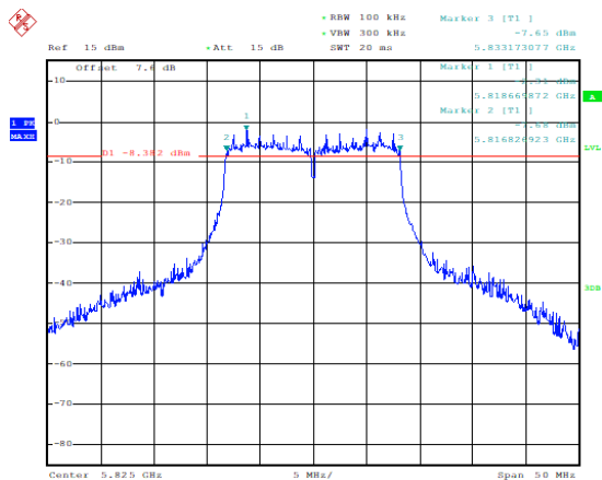
Occupied 6dB Bandwidth ( MHz) (802.11a, 5825MHz)
