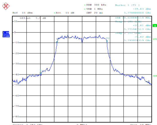
99% Occupied Bandwidth ( MHz) (802.11n-HT20, 5785MHz)
