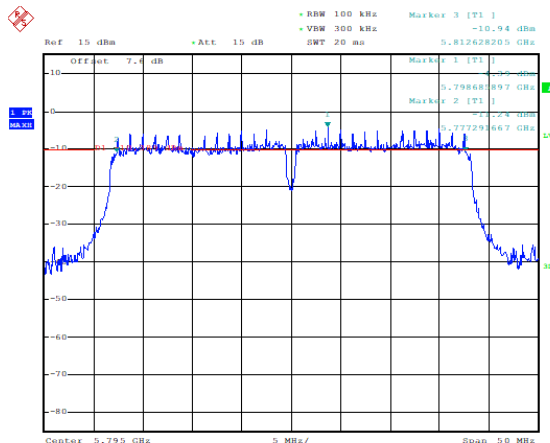
Occupied 6dB Bandwidth ( MHz) (802.11ac-VHT40), 5795MHz)
