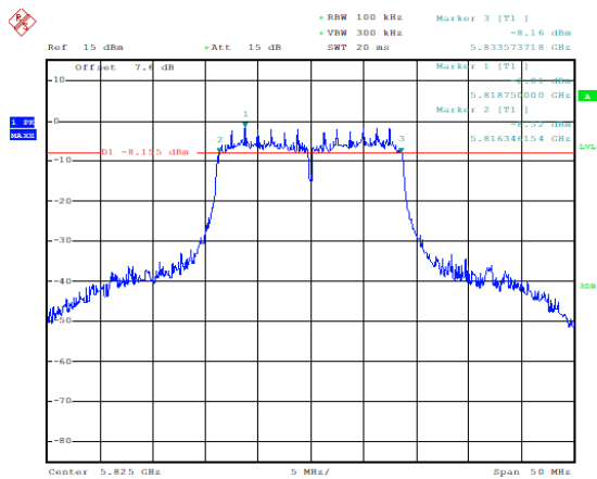
Occupied 6dB Bandwidth ( MHz) (802.11ac-VHT20, 5825MHz)
