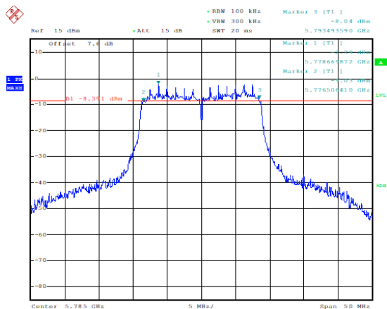
Occupied 6dB Bandwidth ( MHz) (802.11n-HT20, 5785MHz)
