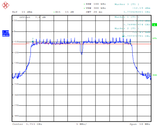
Occupied 6dB Bandwidth ( MHz) (802.11n-HT40, 5755MHz)
