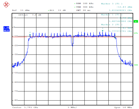
Occupied 6dB Bandwidth ( MHz) (802.11n-HT40), 5795MHz)
