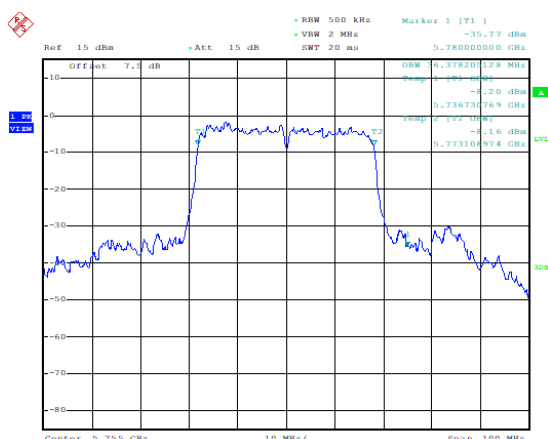
99% Occupied Bandwidth ( MHz) (802.11n-HT40, 5755MHz)
