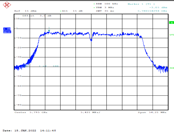
U-NII-3 Power spectral density-802.11 ac(VHT40),5795MHz,Ant1
