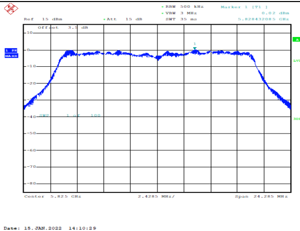
U-NII-3 Power spectral density-802.11 ac(VHT20),5825MHz,Ant1
