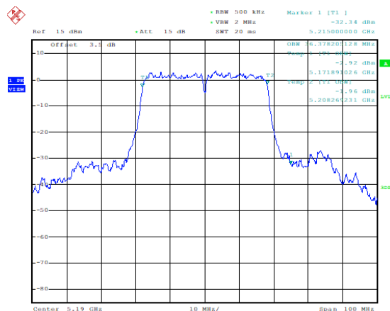
99% Occupied Bandwidth (MHz) (802.11n-HT40), 5190MHz)
