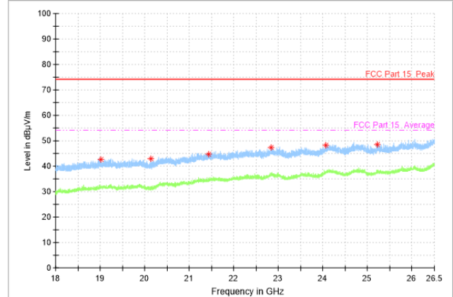
Radiated Spurious Emission (802.11ac-VHT40, ch38, 18GHz-26.5GHz)
