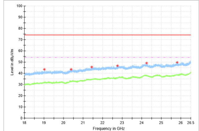
Radiated Spurious Emission (802.11ac-VHT80, ch42, 18GHz-26.5GHz)
