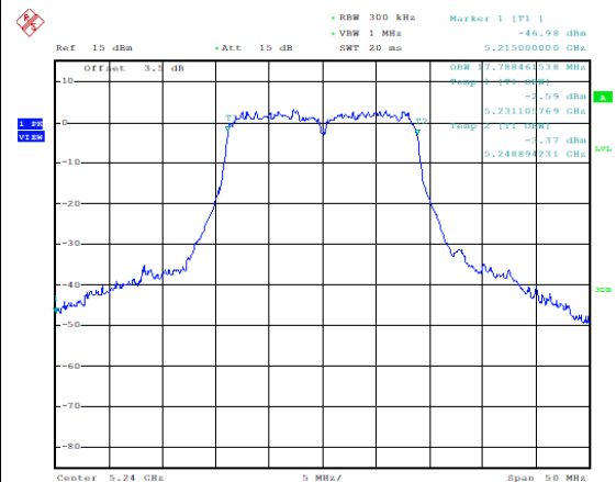
99% Occupied Bandwidth (MHz) (802.11n- HT20), 5240MHz)
