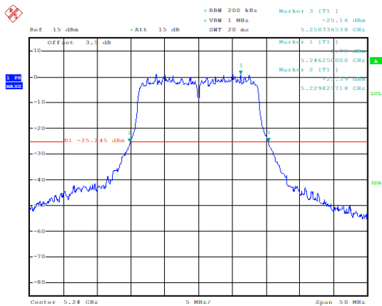
Occupied 26dB Bandwidth (MHz) (802.11ac-VHT20, 5240MHz)
