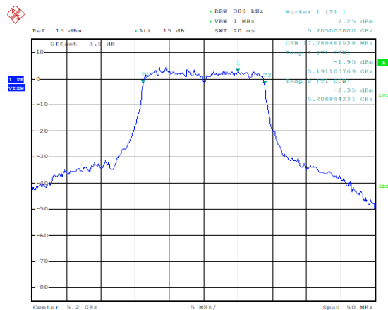
99% Occupied Bandwidth (MHz) (802.11n-HT20), 5200MHz)
