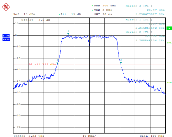
Occupied 26dB Bandwidth (MHz) (802.11ac-VHT40, 5230MHz)
