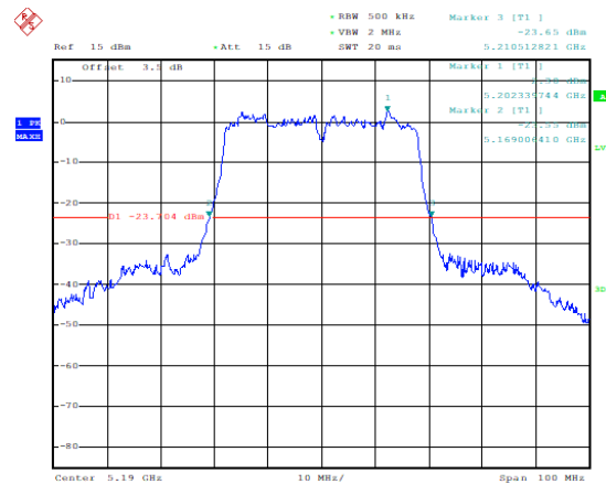
Occupied 26dB Bandwidth (MHz) (802.11ac-VHT40, 5190MHz)
