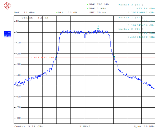
Occupied 26dB Bandwidth (MHz) (802.11n-HT20, 5180MHz)
