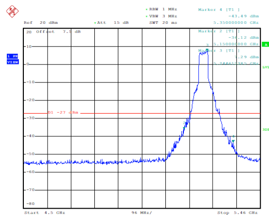
Band Edges (802.11n-HT40), 5230MHz)
