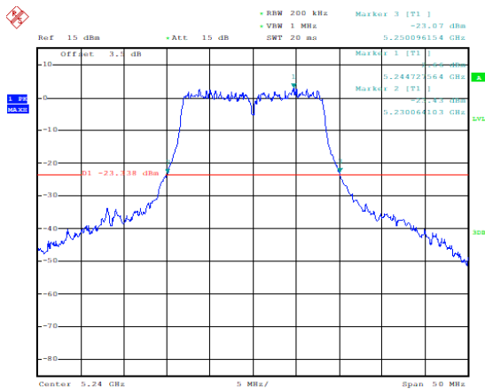
Occupied 26dB Bandwidth (MHz) (802.11a, 5240MHz)
