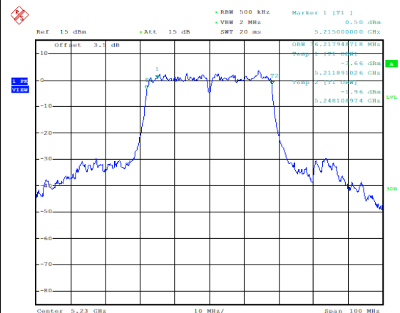
99% Occupied Bandwidth (MHz) (802.11n-HT40), 5230MHz)
