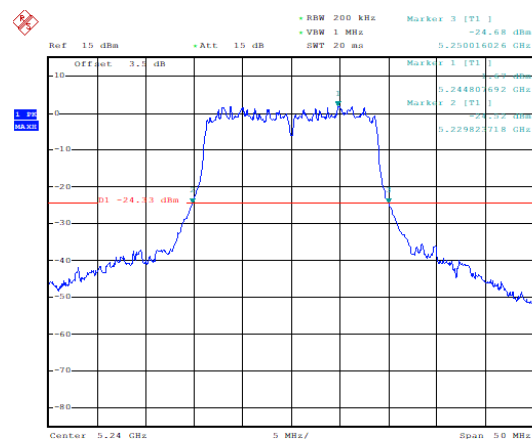
Occupied 26dB Bandwidth (MHz) (802.11n-HT20, 5240MHz)
