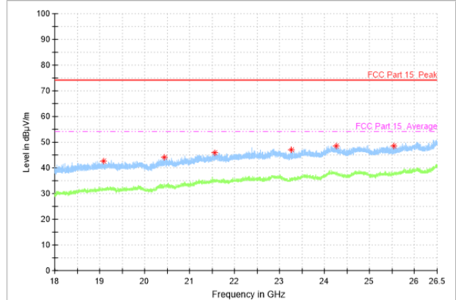
Radiated Spurious Emission (802.11n-HT20, ch48, 18GHz-26.5GHz)
