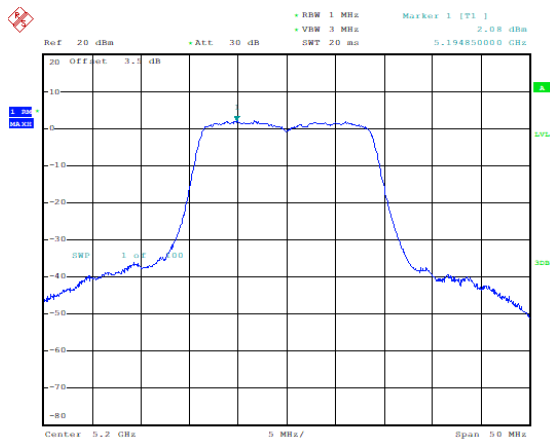
Power Spectral Density(dBm/MHz) (802.11n-HT20, 5200MHz)
