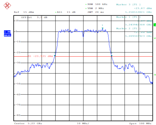
Occupied 26dB Bandwidth (MHz) (802.11n-HT40, 5230MHz)
