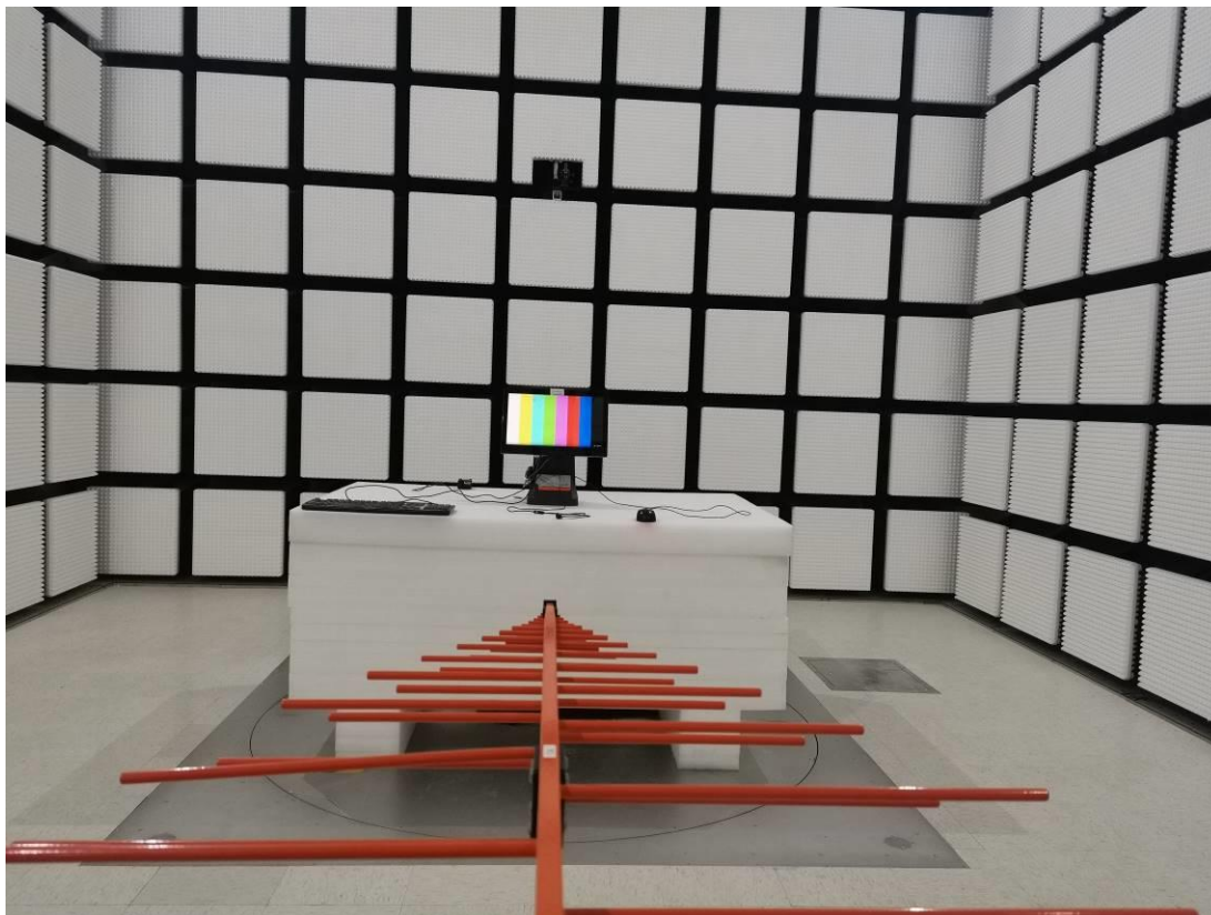
Radiated Emission Above View L1583
