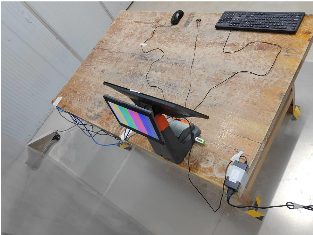
Conducted Emissions Side View L1582
