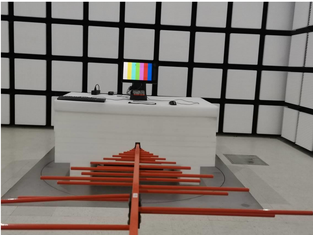
Radiated Emission Below 1GHz View L1581
