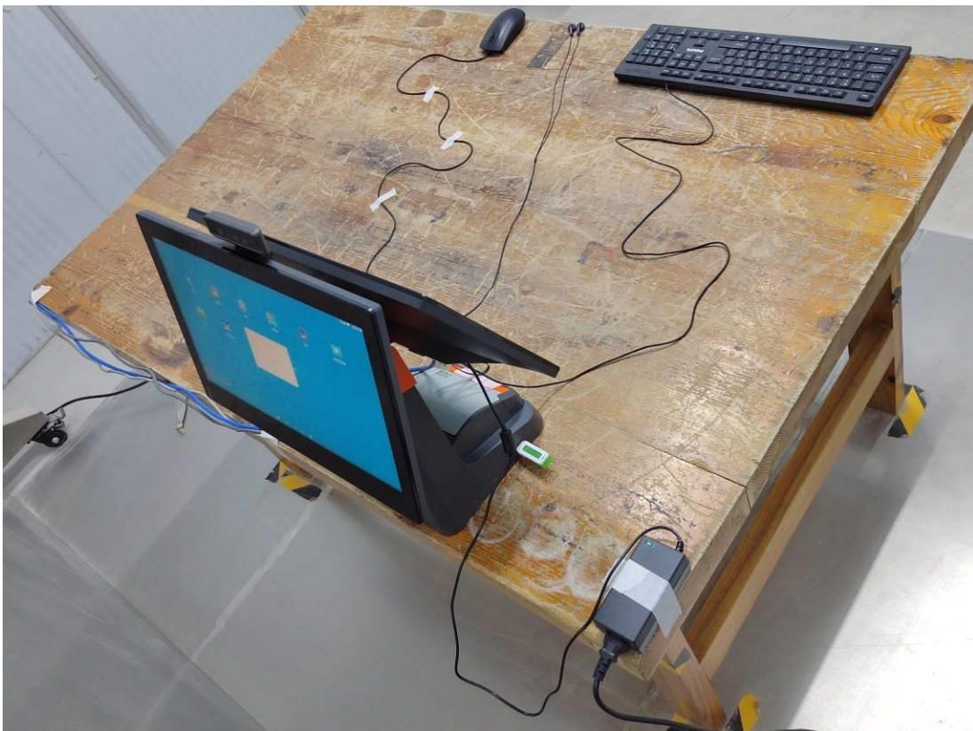
Conducted Emissions Side View L1583
