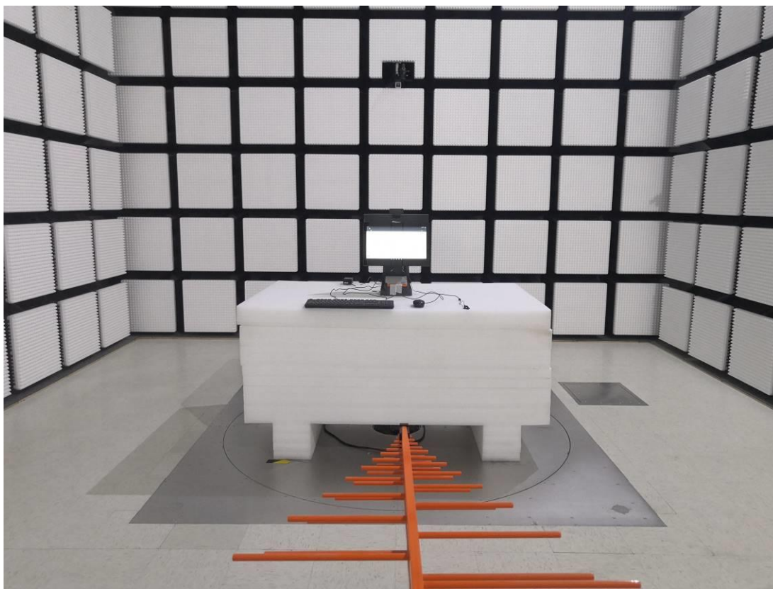
Radiated Emission Above 1GHz View L1583
