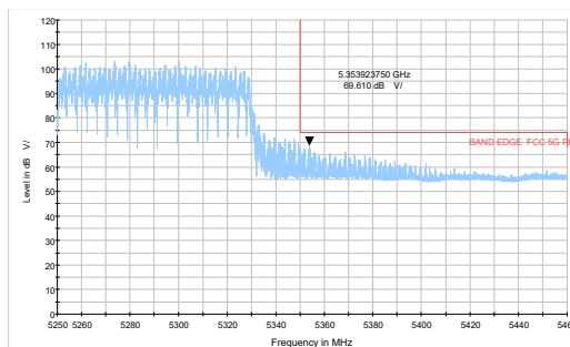
802.11ax HE80 –Channel 58: Peak + Average
