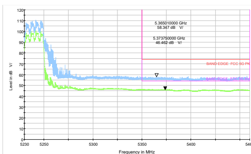
802.11ax HE20 -Channel 64: Peak + Average
