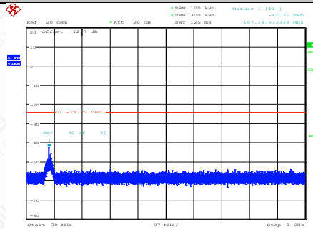
11N40SISO-Ant1-2422-30~1000-PASS
