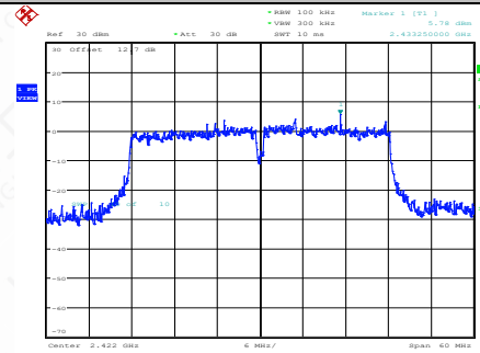
11N40SISO-Ant1-2422-0~Reference-PASS
