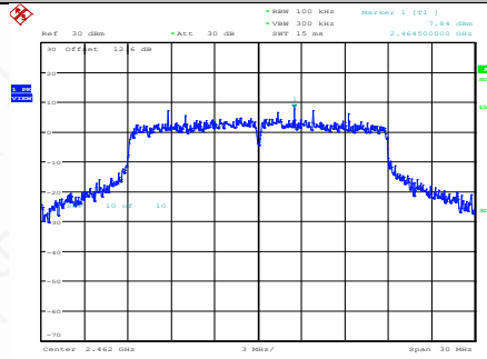
11N20SISO-Ant1-2462-0~Reference-PASS
