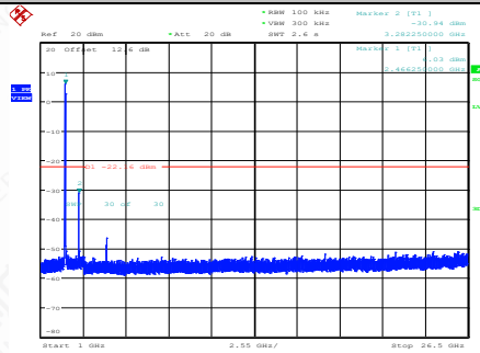
11N20SISO-Ant1-2462-1000~26500-PASS
