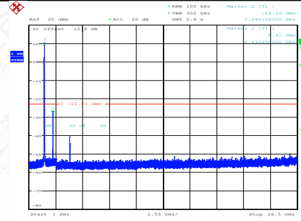
11N20SISO-Ant1-2437-1000~26500-PASS
