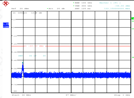
11N20SISO-Ant1-2437-30~1000-PASS
