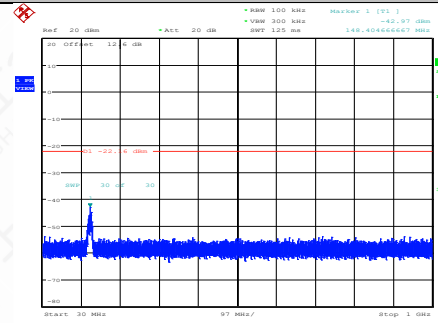
11N20SISO-Ant1-2462-30~1000-PASS
