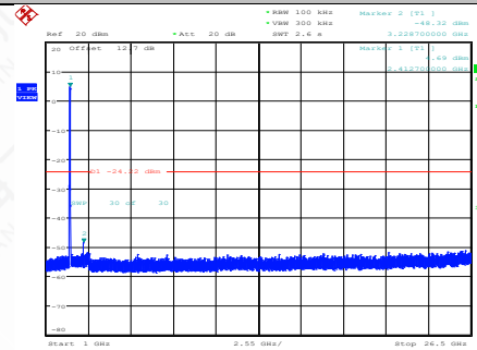
11N40SISO-Ant1-2422-1000~26500-PASS
