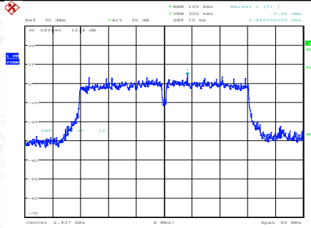
11N40SISO-Ant1-2437-0~Reference-PASS
