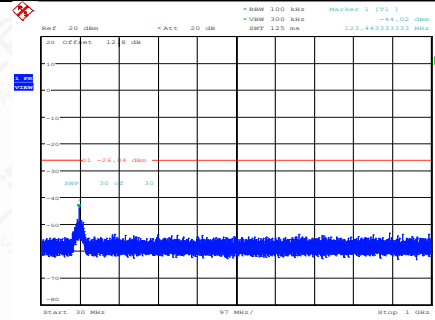
11N40SISO-Ant1-2437-30~1000-PASS
