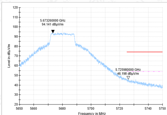
Bandedge-11A-CH136-AV
