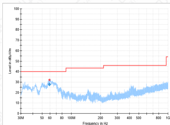
RSE-11N(40M)-CH62-30MHz-1GHz
