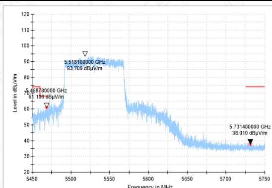
Bandedge-11AC(80M)-CH106-PK
