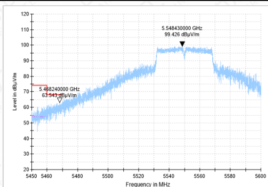
BANDEDGE-11AC(40M)-CH110-PK
