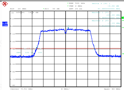
11AC40SISO-Ant1-5510
