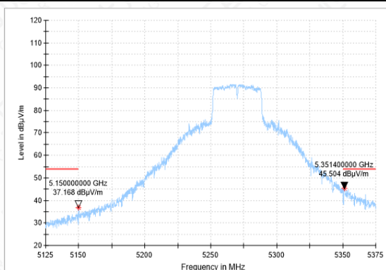
Bandedge-11AC(40M)-CH54-AV
