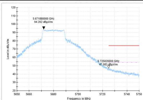
Bandedge-11N(20M)-CH136-AV
