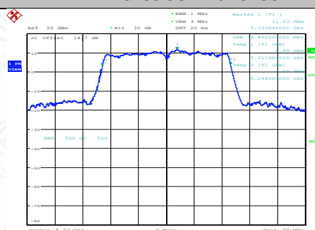
11AC40SISO-Ant1-5230
