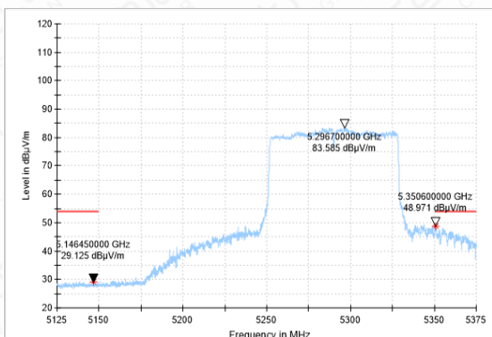
Bandedge-11AC(80M)-CH58-AV
