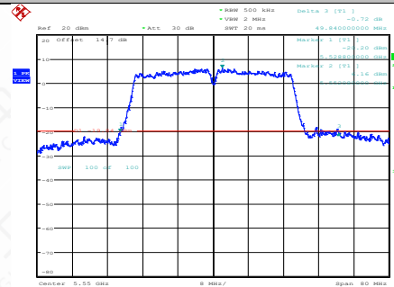
11AC40SISO-Ant1-5550
