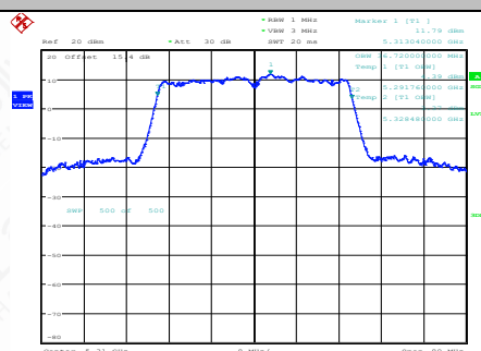
11AC40SISO-Ant1-5310
