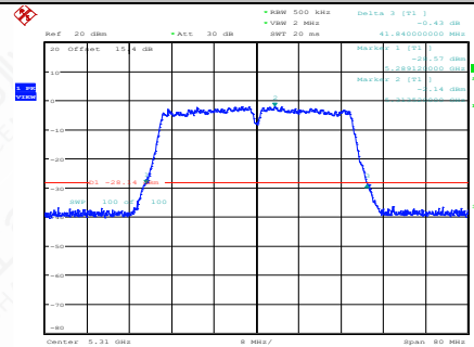
11AC40SISO-Ant1-5310
