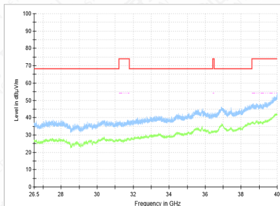
RSE-11A-CH64-26.5GHz-40GHz
