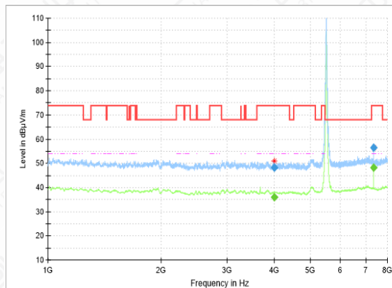
RSE-11A-CH100-1GHz-8GHz
