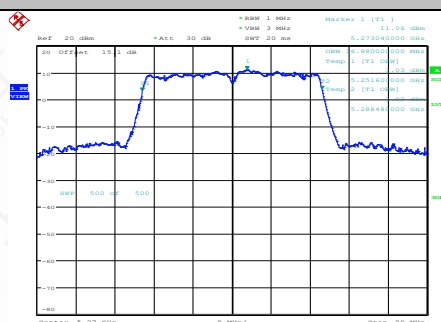
11AC40SISO-Ant1-5270
