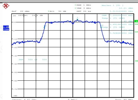
11AC40SISO-Ant1-5510
