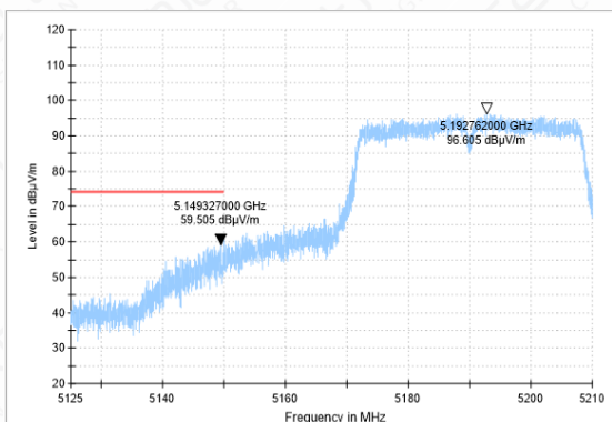
Bandedge-11AC(40M)-CH38-PK
