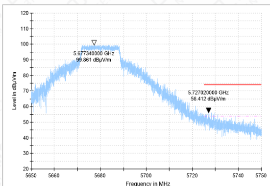
Bandedge-11A-CH136-PK
