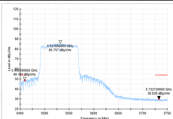
Bandedge-11AC(80M)-CH106-AV
