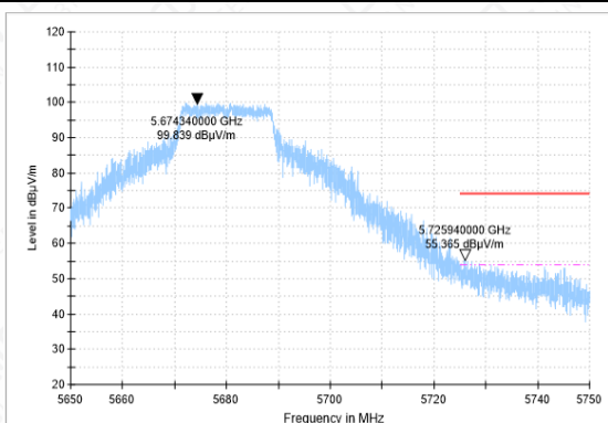
Bandedge-11AC(20M)-CH136-PK
