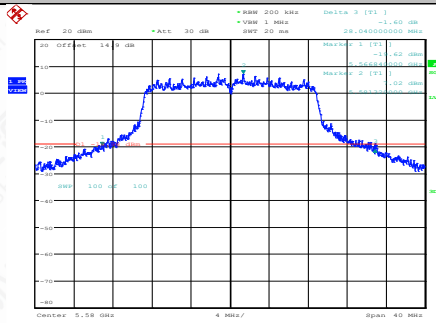
11AC20SISO-Ant1-5580
