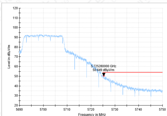
Bandedge-11A-CH140-AV
