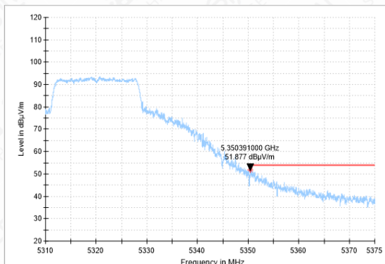
Bandedge-11A-CH64-AV
