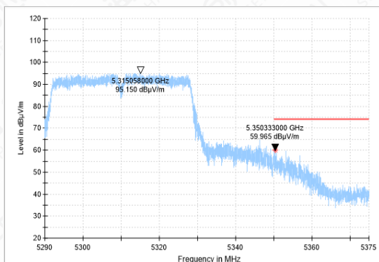
Bandedge-11AC(40M)-CH62-PK
