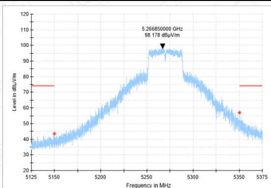
Bandedge-11AC(40M)-CH54-PK
