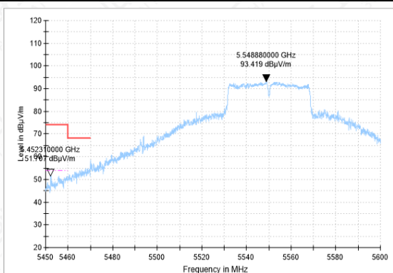
BANDEDGE-11AC(40M)-CH110-AV
