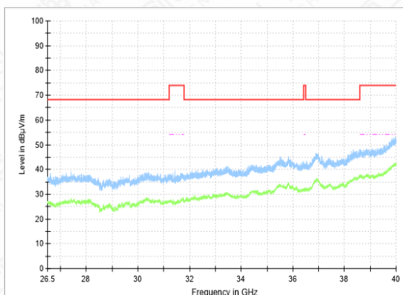
RSE-11N(40M)-CH38-26.5GHz-40GHz
