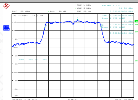
11AC40SISO-Ant1-5550
