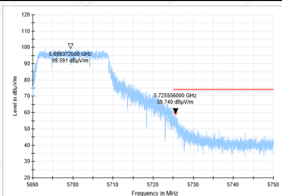
Bandedge-11AC(20M)-CH140-PK
