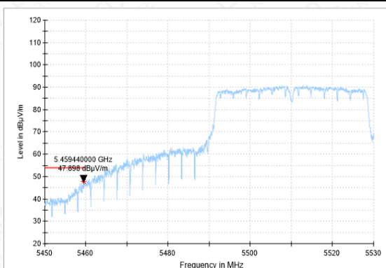
Bandedge-11AC(40M)-CH102-AV
