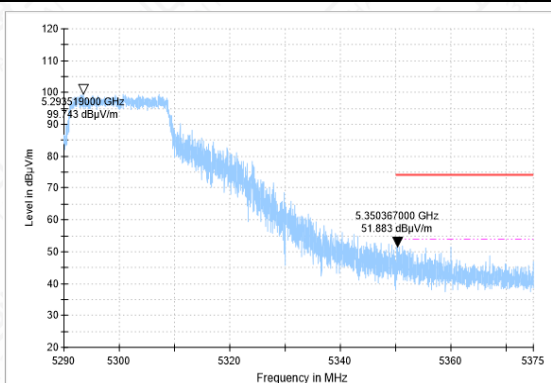
Bandedge-11N(20M)-CH60-PK
