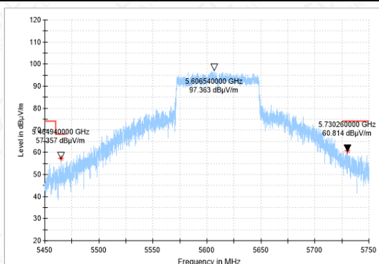
Bandedge-11AC(80M)-CH122-PK
