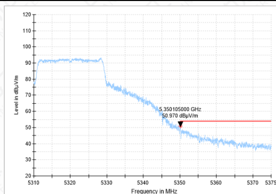
Bandedge-11N(20M)-CH64-AV
