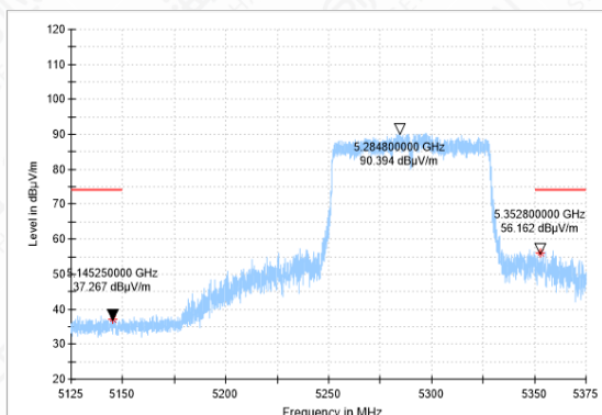
Bandedge-11AC(80M)-CH58-PK
