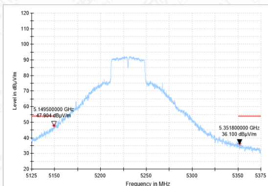
Bandedge-11AC(40M)-CH46-AV
