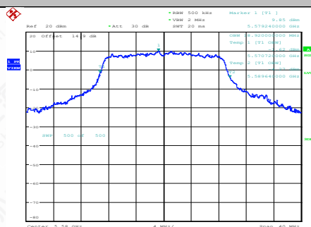
11AC20SISO-Ant1-5580
