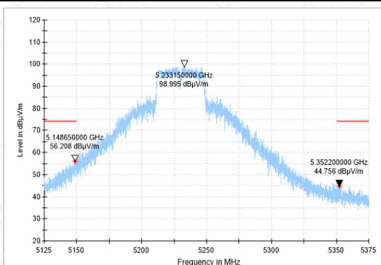
Bandedge-11AC(40M)-CH46-PK
