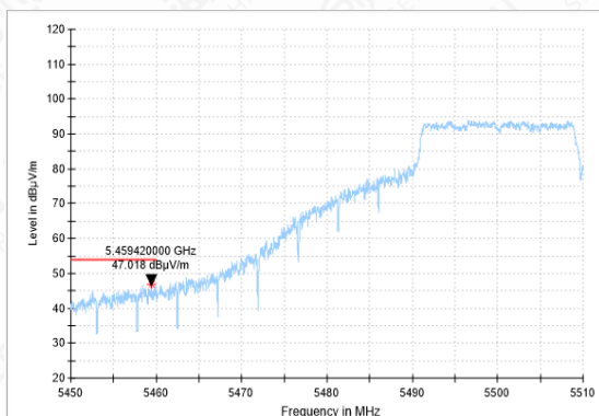
Bandedge-11N(20M)-CH100-AV
