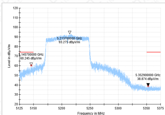
Bandedge-11AC(80M)-CH42-PK
