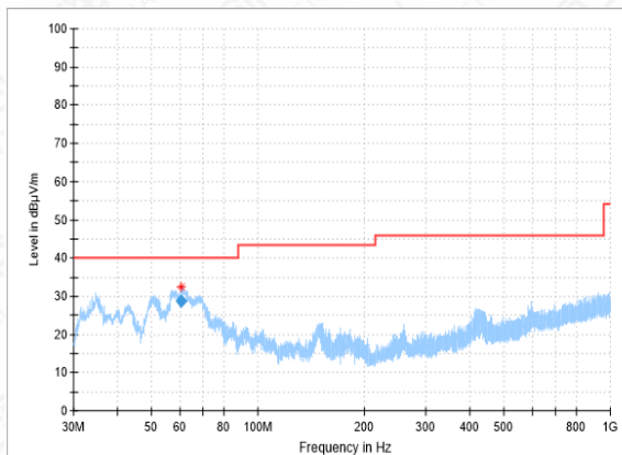
RSE-11A-CH100-30MHz-1GHz
