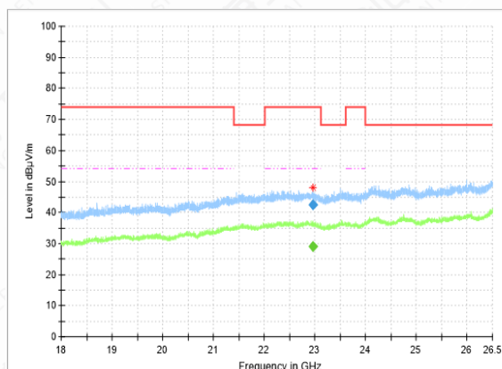
RSE-11N(40M)-CH38-18GHz-26.5GHz
