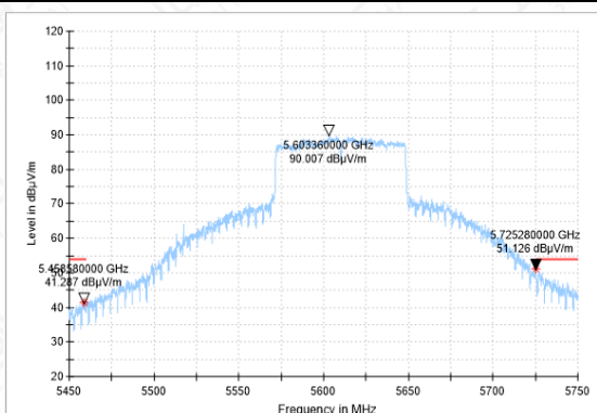
Bandedge-11AC(80M)-CH122-AV
