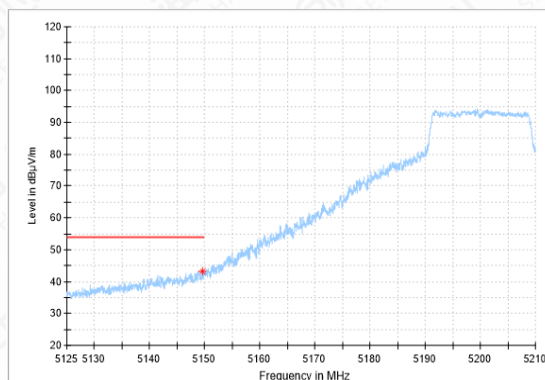
Bandedge-11N(20M)-CH40-AV
