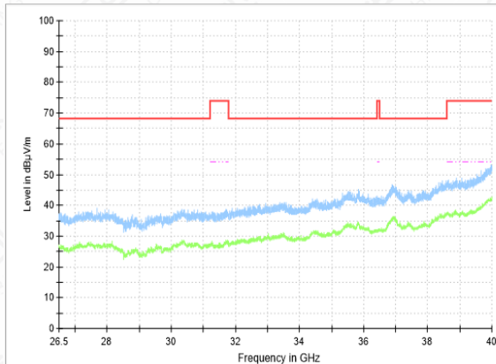
RSE-11A-CH100-26.5GHz-40GHz
