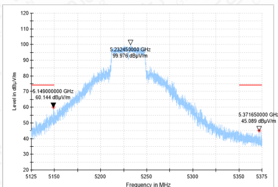
Bandedge-11N(40M)-CH46-PK
