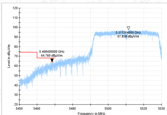
Bandedge-11N(40M)-CH102-PK
