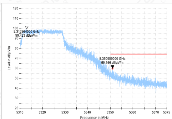
Bandedge-11N(20M)-CH64-PK
