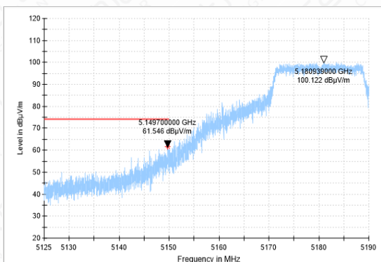
Bandedge-11N(20M)-CH36-PK
