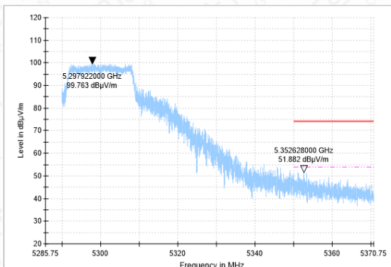
Bandedge-11A-CH60-PK
