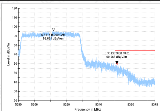
Bandedge-11N(40M)-CH62-PK
