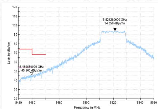
Bandedge-11AC(20M)-CH104-AV
