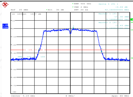
11AC40SISO-Ant1-5190
