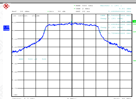
11AC20SISO-Ant1-5700
