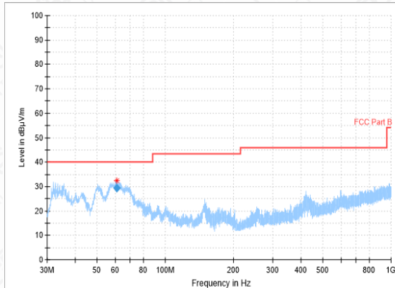
RSE-11N-CH36-30MHz-1GHz
