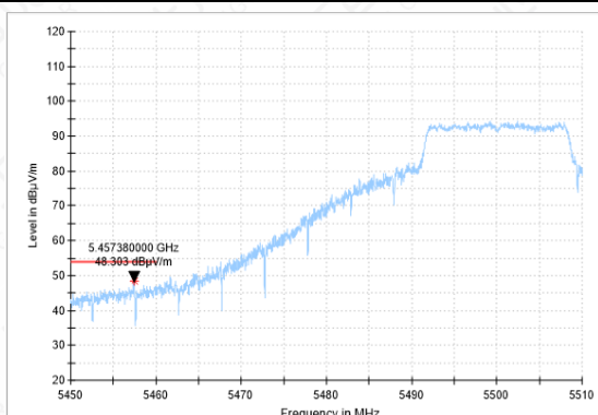
Bandedge-11A-CH100-AV
