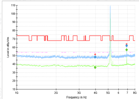
RSE-11N-CH36-1GHz-8GHz
