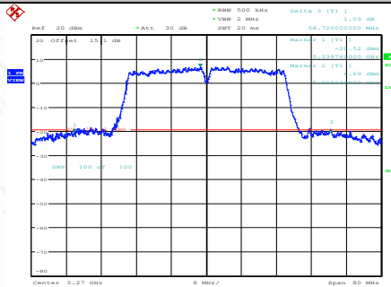
11AC40SISO-Ant1-5270
