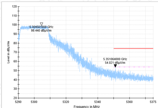
Bandedge-11AC(20M)-CH64-PK
