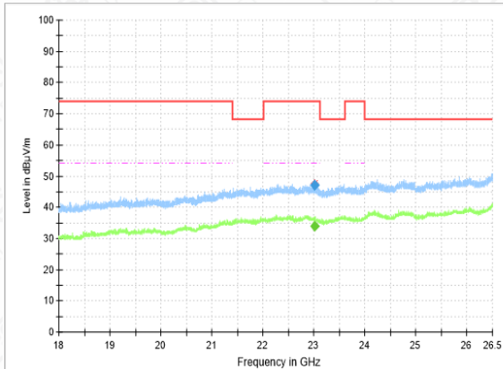
RSE-11N-CH165-18GHz-26.5GHz
