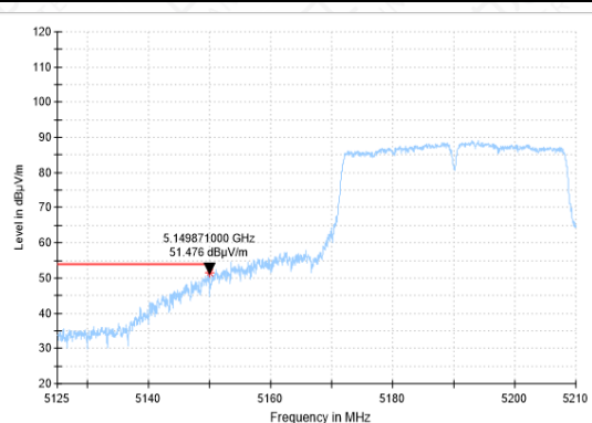
Bandedge-11AC(40M)-CH38-AV
