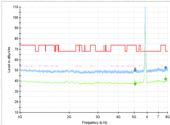
RSE-11N-CH165-1GHz-8GHz
