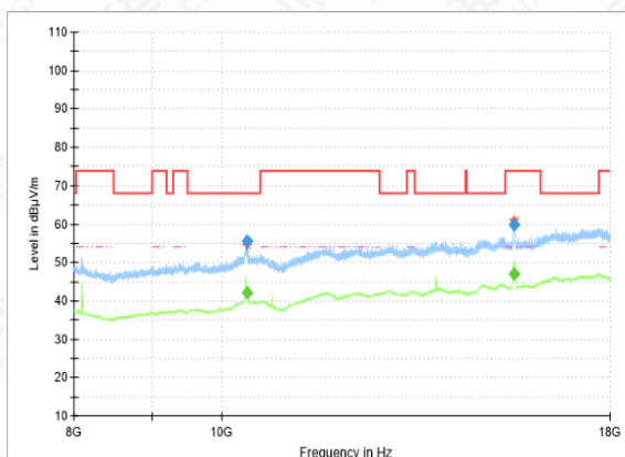
RSE-11N(40M)-CH38-8GHz-18GHz
