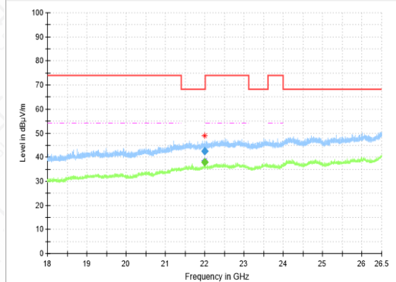
RSE-11A-CH100-18GHz-26.5GHz
