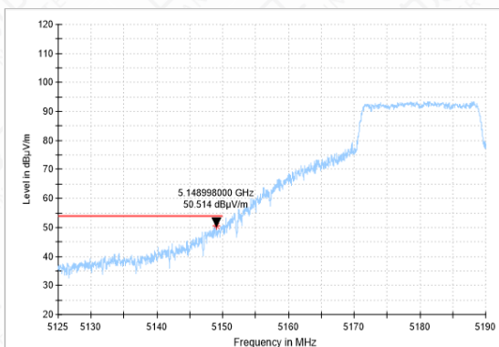
Bandedge-11N(20M)-CH36-AV
