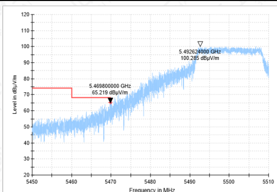
Bandedge-11A-CH100-PK
