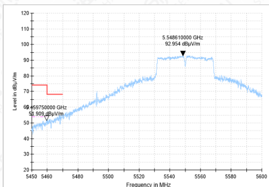
Bandedge-11N(40M)-CH110-AV
