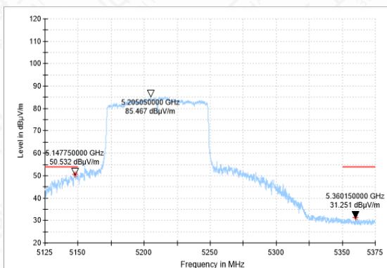
Bandedge-11AC(80M)-CH42-AV
