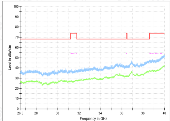
RSE-11N-CH165-26.5GHz-40GHz
