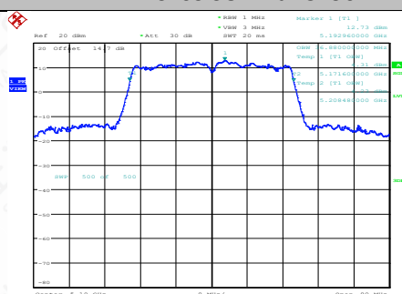
11AC40SISO-Ant1-5190
