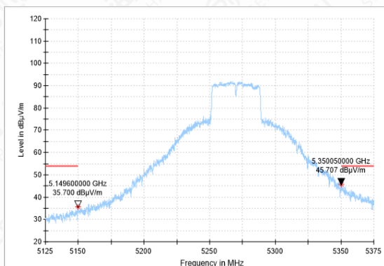
Bandedge-11N(40M)-CH54-AV
