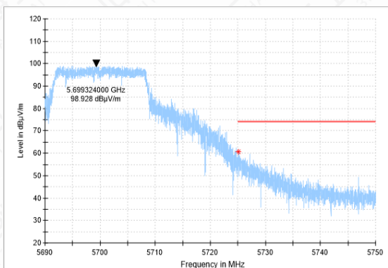
Bandedge-11A-CH140-PK
