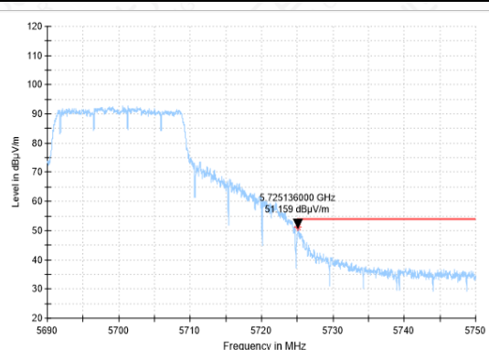
Bandedge-11AC(20M)-CH140-AV
