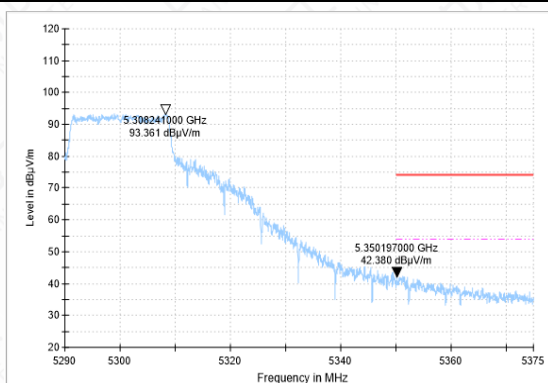
Bandedge-11AC(20M)-CH60-AV
