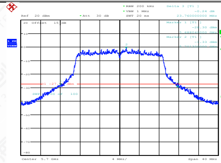
11AC20SISO-Ant1-5700
