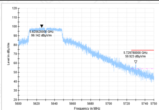
Bandedge-11N(40M)-CH126-PK
