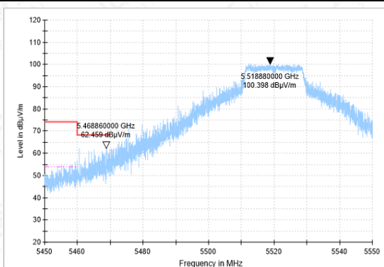
Bandedge-11N(20M)-CH104-PK
