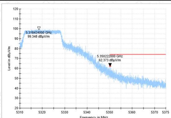
Bandedge-11A-CH64-PK
