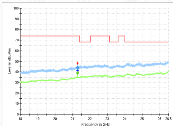
RSE-11A-CH64-18GHz-26.5GHz
