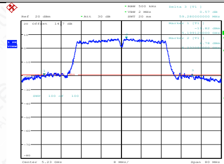
11AC40SISO-Ant1-5230
