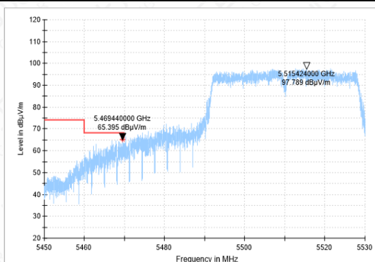
Bandedge-11AC(40M)-CH102-PK
