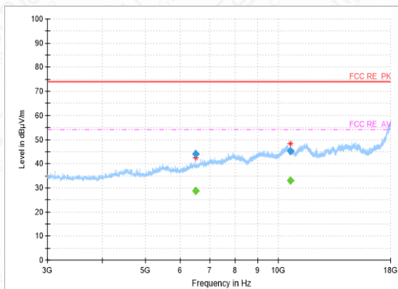
RSE-2DH5-CH39-3GHz-18GHz
