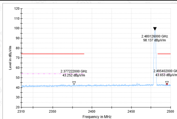
Bandedge-3DH5-CH78-AV
