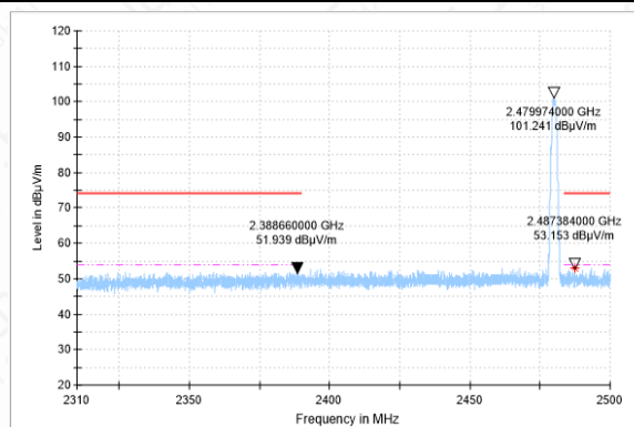
Bandedge-3DH5-CH78-PK
