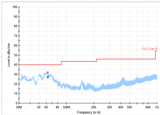
RSE-3DH5-CH0-30MHz-1GHz
