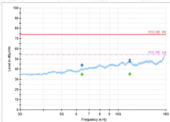
RSE-3DH5-CH0-3GHz-18GHz
