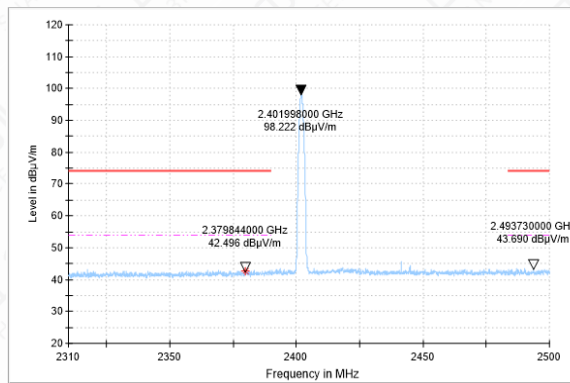
Bandedge-3DH5-CH0-AV
