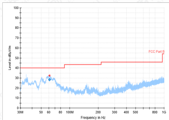
RSE-3DH5-CH39-30MHz-1GHz
