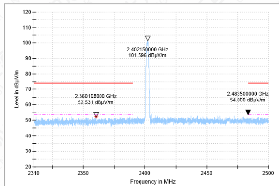
Bandedge-3DH5-CH0-PK
