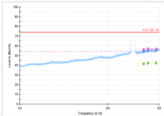
RSE-2DH5-CH39-1GHz-3GHz
