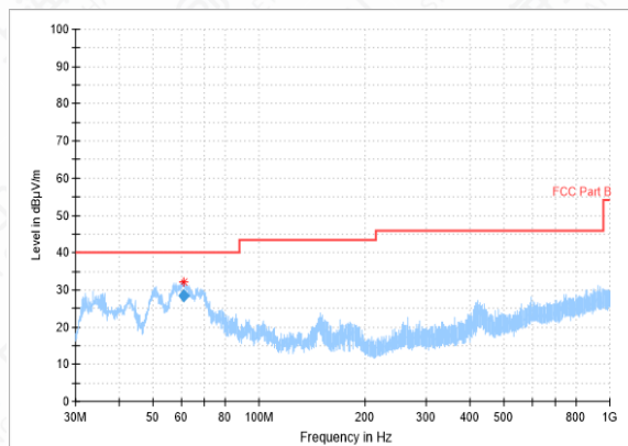
RSE-2DH5-CH0-30MHz-1GHz
