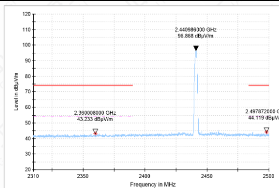
Bandedge-3DH5-CH39-AV
