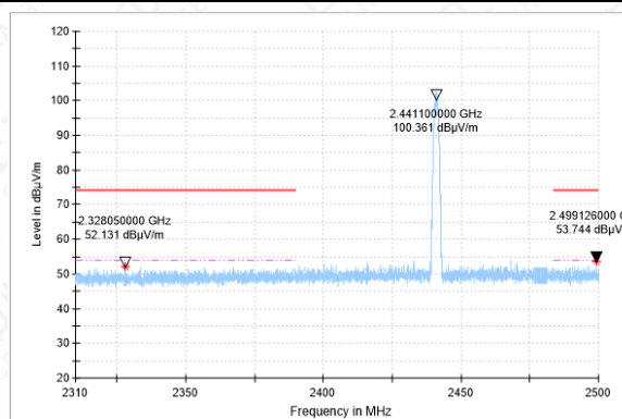
Bandedge-3DH5-CH39-PK
