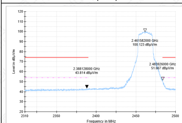
BANEDGE-11N(20M)-CH11-AV
