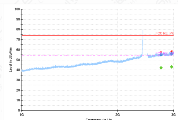
RSE-11B-CH1-1GHz-3GHz
