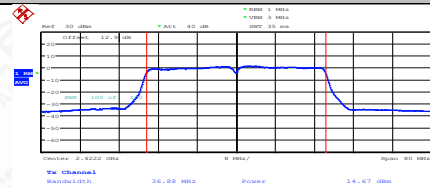
11N40SISO-Ant1-2422-PASS
