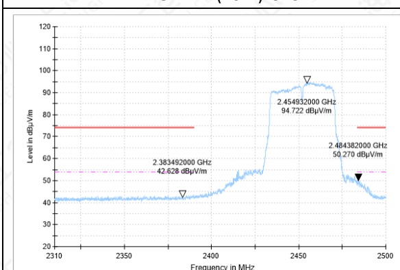
BANEDGE-11N(40M)-CH9-AV
