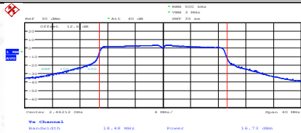
11N20SISO-Ant1-2462-PASS
