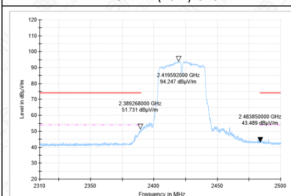
BANEDGE-11N(40M)-CH3-AV
