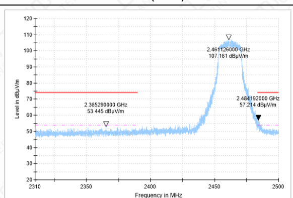
BANEDGE-11N(20M)-CH11-PK
