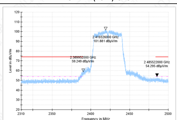
BANEDGE-11N(40M)-CH3-PK
