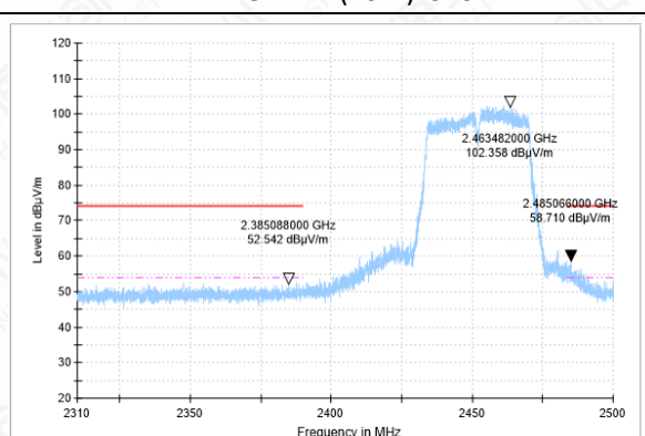
BANEDGE-11N(40M)-CH9-PK
