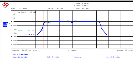
11N40SISO-Ant1-2437-PASS
