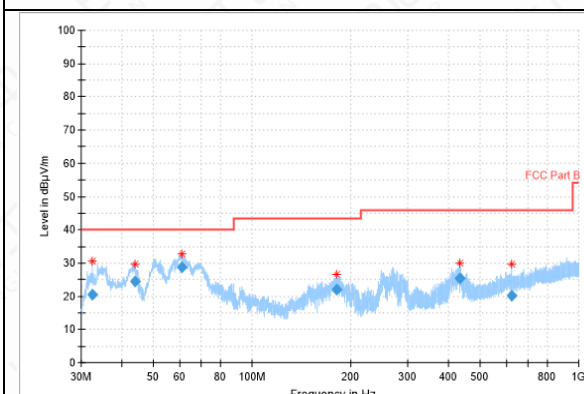
RSE-11B-CH1-30MHz-1GHz
