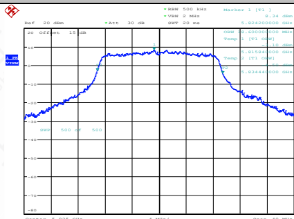
11AC20SISO-Ant1-5825
