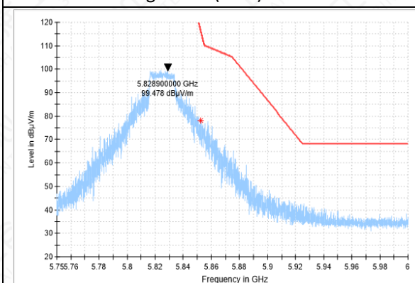
Bandedge-11AC(20M)-CH165-PK
