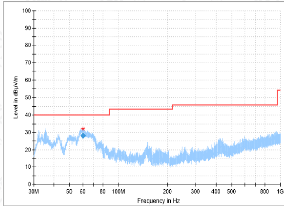
RSE-11AC(40M)-CH151-30MHz-1GHz
