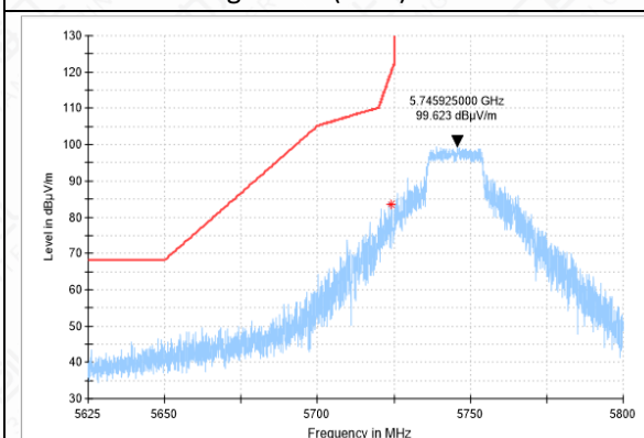
Bandedge-11AC(20M)-CH149-PK
