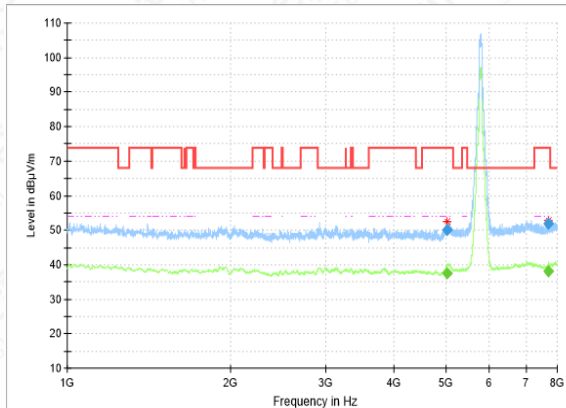
RSE-11AC(80M)-CH155-1GHz-8GHz
