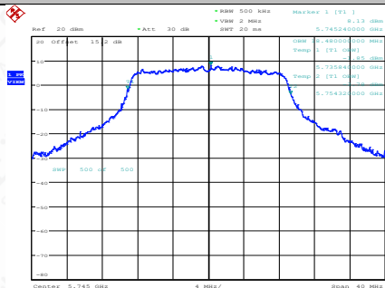
11AC20SISO-Ant1-5745
