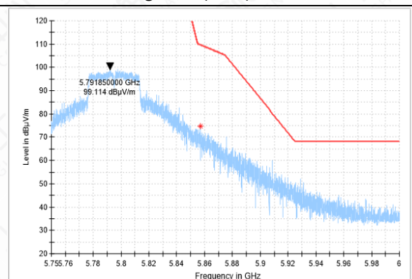
Bandedge-11N(40M)-CH159-PK
