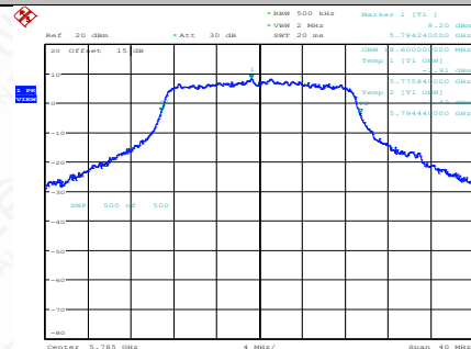
11AC20SISO-Ant1-5785
