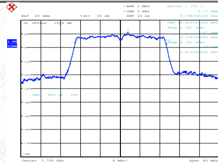
11N40SISO-Ant1-5795
