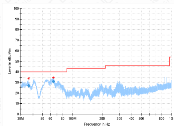
RSE-11AC(80M)-CH155-30MHz-1GHz
