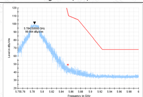
Bandedge-11AC(20M)-CH157-PK
