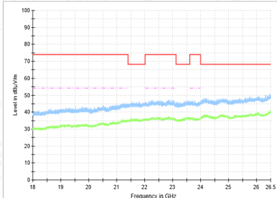
RSE-11AC(80M)-CH155-18GHz-26.5GHz
