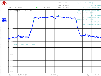
11N40SISO-Ant1-5755
