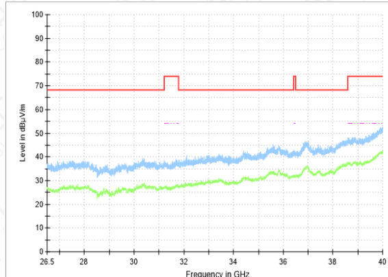
RSE-11AC(80M)-CH155-26.5GHz-40GHz
