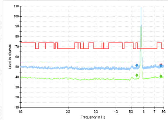
RSE-11AC(40M)-CH151-1GHz-8GHz
