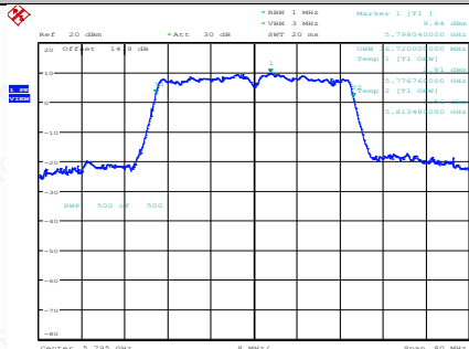
11AC40SISO-Ant1-5795
