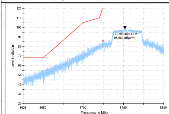
Bandedge-11N(40M)-CH151-PK
