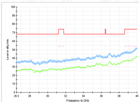
RSE-11AC(40M)-CH151-26.5GHz-40GHz
