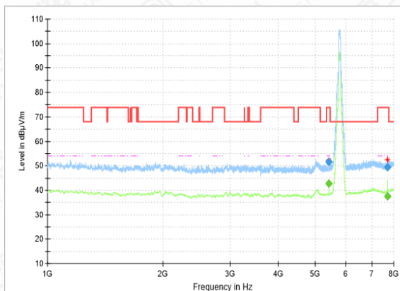
RSE-11AC(80M)-CH155-1GHz-8GHz
