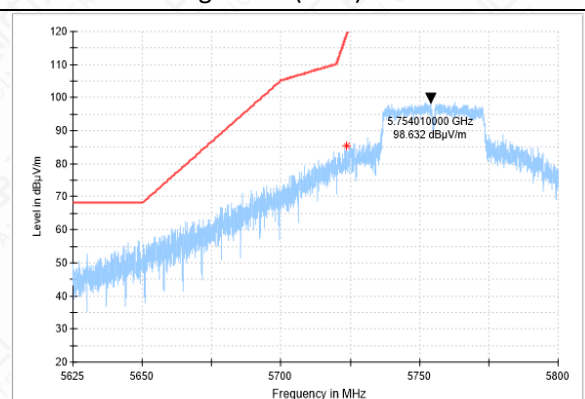
Bandedge-11AC(40M)-CH151-PK
