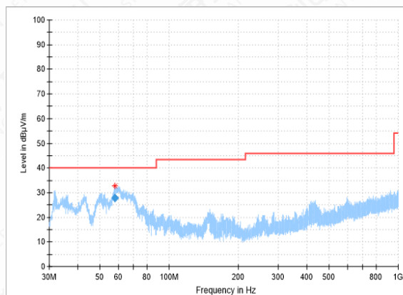
RSE-11AC(80M)-CH155-30MHz-1GHz
