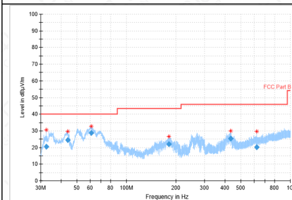
RSE-11B-CH1-30MHz-1GHz
