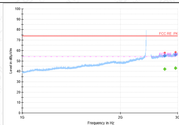
RSE-11B-CH1-1GHz-3GHz
