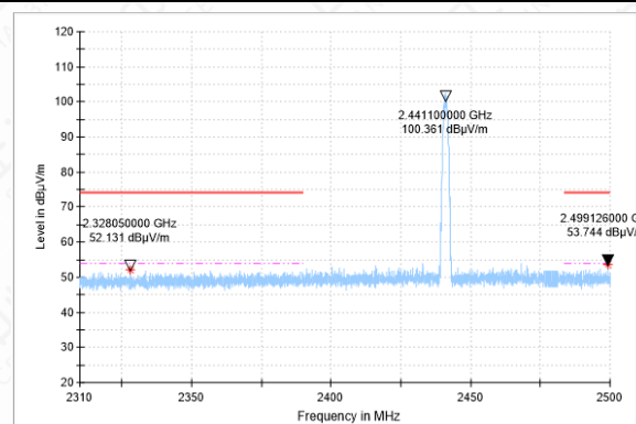
Bandedge-3DH5-CH39-PK
