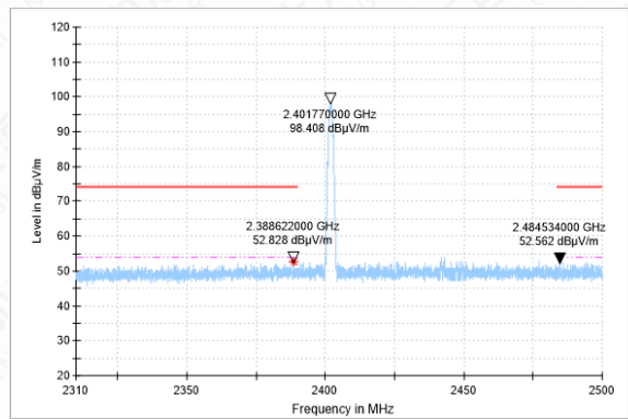
Bandedge-2DH5-CH0-PK
