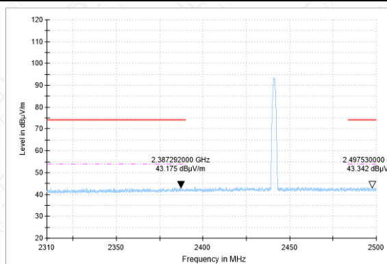
Bandedge-2DH5-CH39-AV
