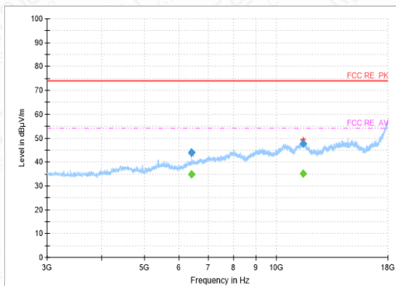
RSE-3DH5-CH0-3GHz-18GHz
