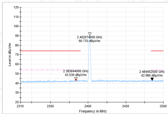
Bandedge-2DH5-CH0-AV
