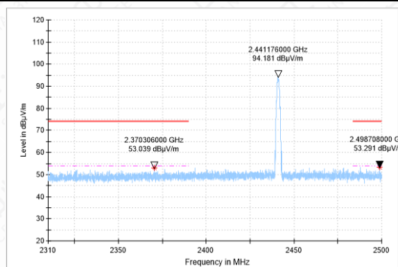
Bandedge-2DH5-CH39-PK
