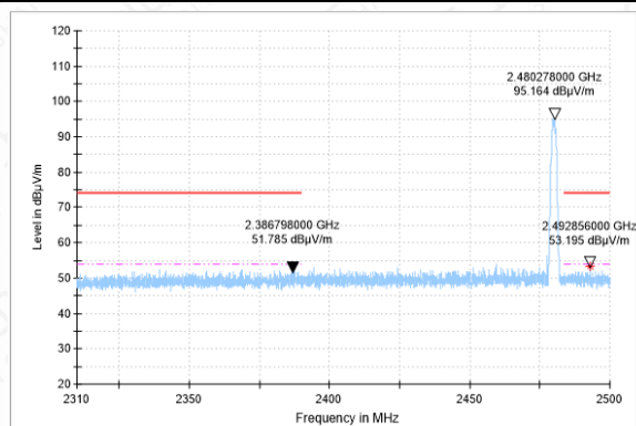
Bandedge-2DH5-CH78-PK
