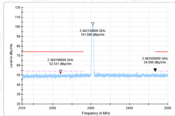
Bandedge-3DH5-CH0-PK
