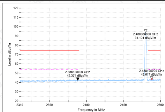
Bandedge-2DH5-CH78-AV
