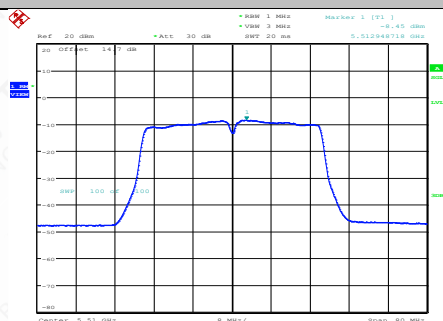
11AC40SISO-Ant1-5510-PASS
