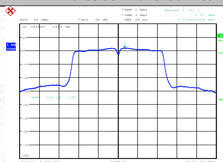
11AC40SISO-Ant1-5230-PASS
