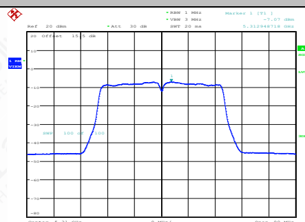
11AC40SISO-Ant1-5310-PASS
