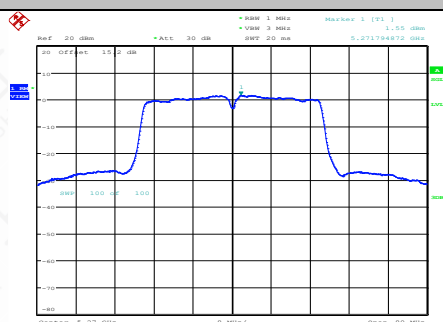
11AC40SISO-Ant1-5270-PASS
