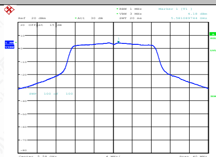
11AC20SISO-Ant1-5580-PASS
