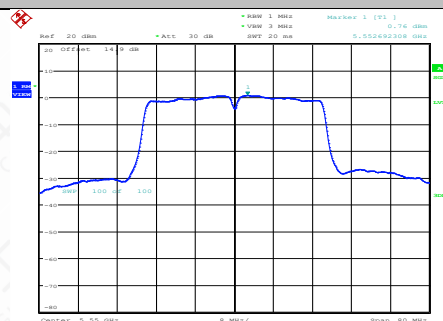
11AC40SISO-Ant1-5550-PASS
