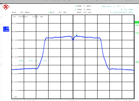
11AC40SISO-Ant1-5190-PASS
