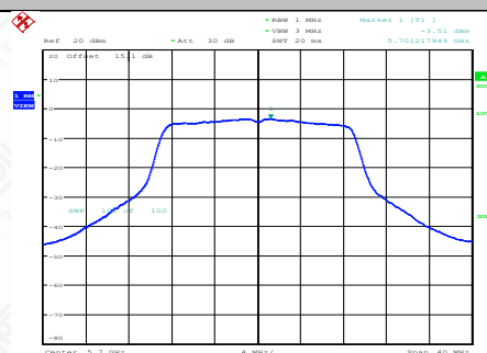
11AC20SISO-Ant1-5700-PASS
