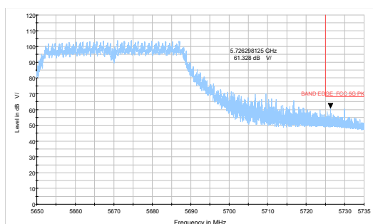
802.11ac VHT40-Channel 134: Peak
