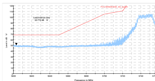
802.11a-Channel 149: Peak
