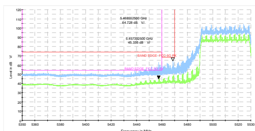
802.11n HT40-Channel 102: Peak + Average
