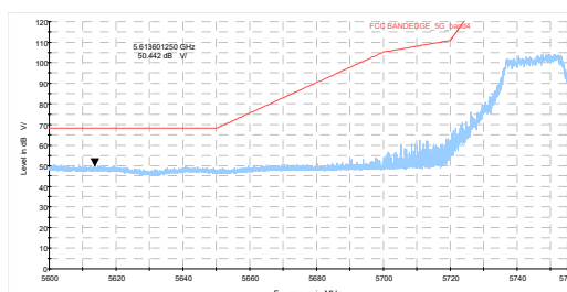
802.11ac VHT20-Channel 149: Peak
