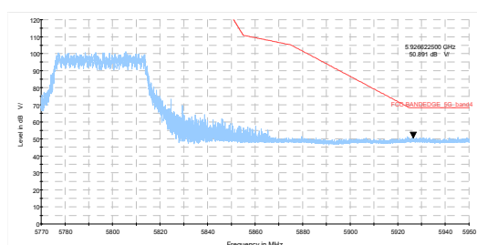
802.11n HT40-Channel 159: Peak
