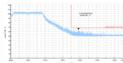
802.11ac VHT20-Channel 140: Peak
