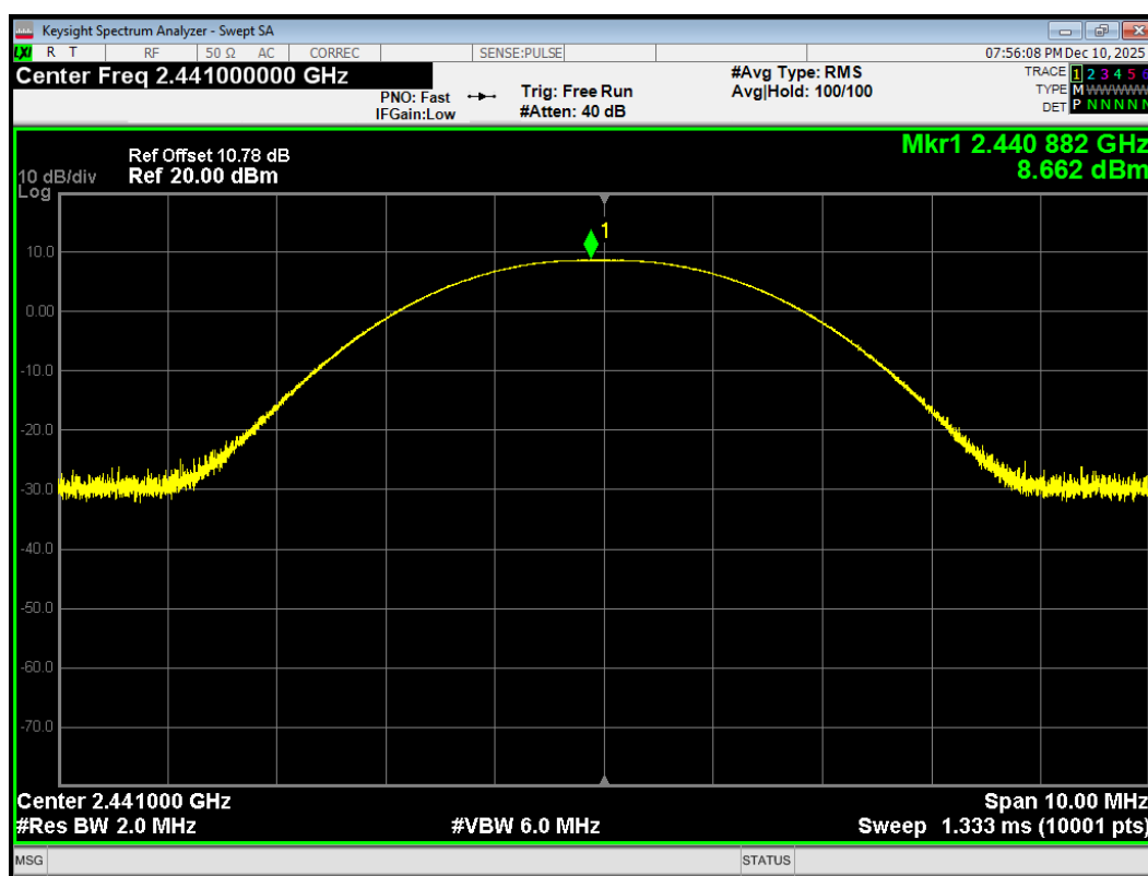
Power 1-DH5 2441MHz
