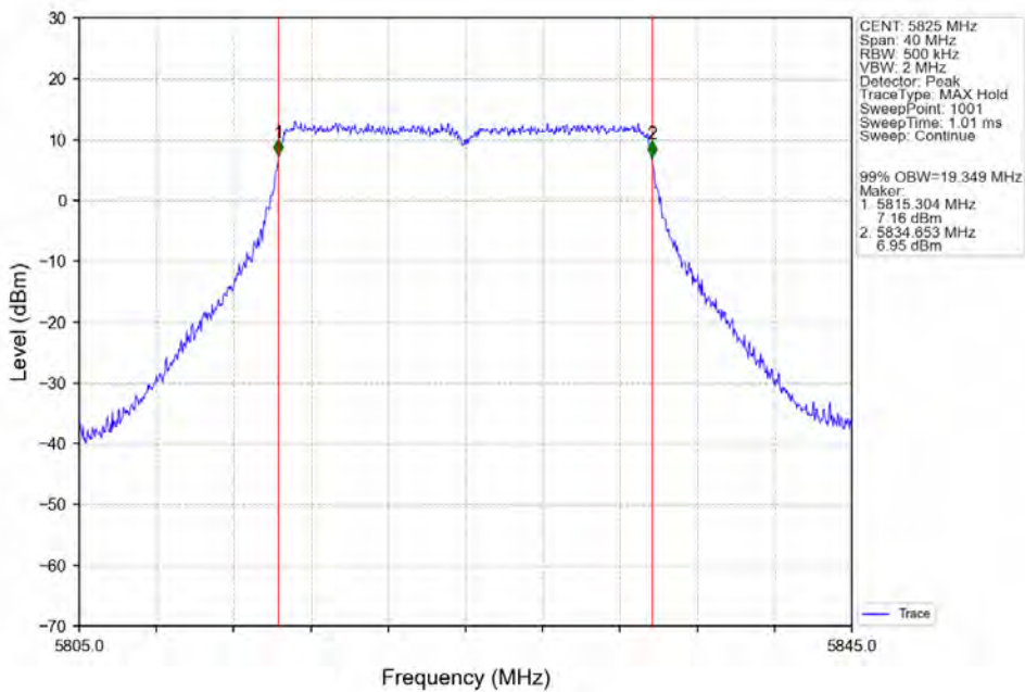
802.11ax(HEW20)_HCH_5825MHz_SU_/_Ant2_NTNV
