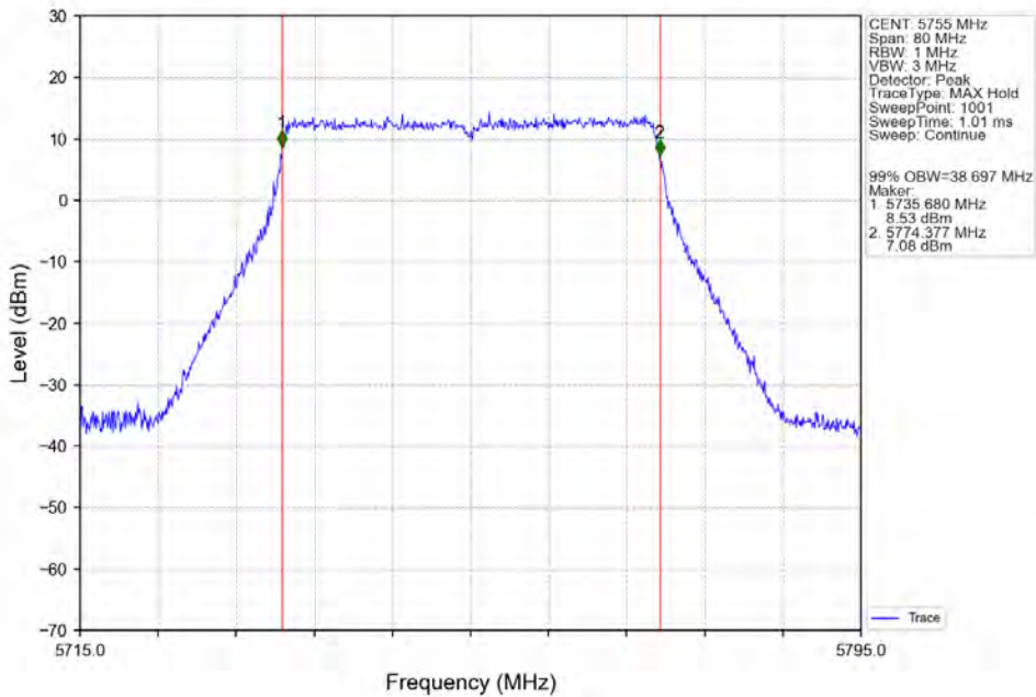
802.11ax(HEW40)_LCH_5755MHz_SU_/_Ant2_NTNV
