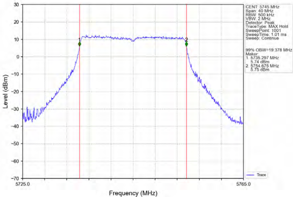
802.11ax(HEW20)_LCH_5745MHz_SU_/_Ant2_NTNV
