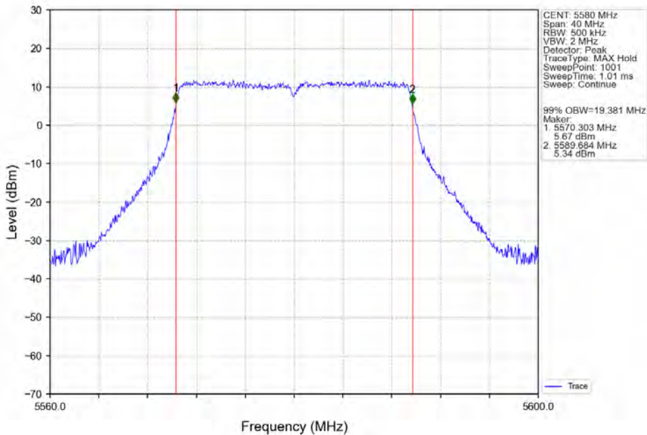
802.11ax(HEW20)_MCH_5580MHz_SU_/_Ant2_NTNV
