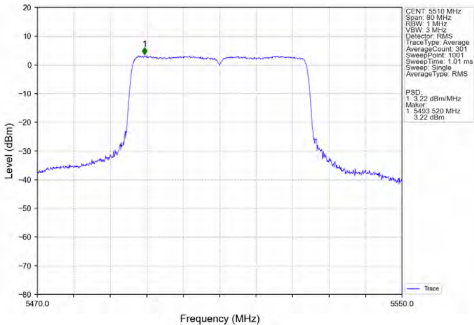
802.11ax(HEW40)_LCH_5510MHz_SU_/_Ant2_NTNV
