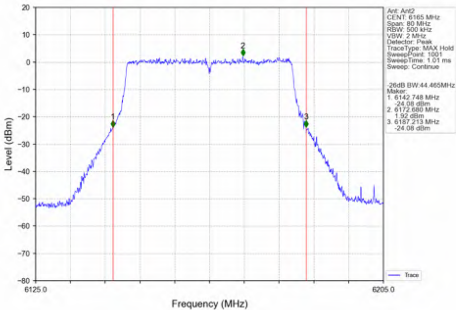
802.11ax(HEW40) MCH_6165MHz_SU / Ant2_NTNV
