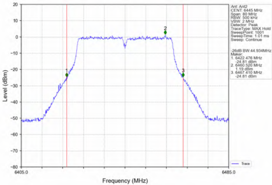
802.11n(HT40) LCH_6445MHz_Ant2_NTNV
