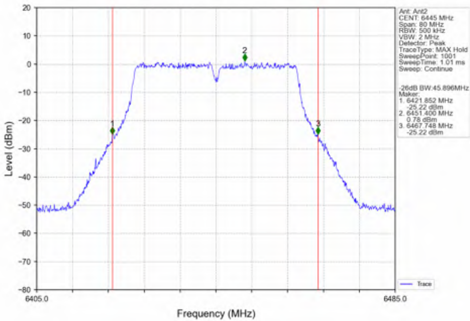
802.11ac(VHT40) LCH_6445MHz_Ant2_NTNV
