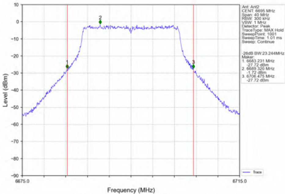
802.11ac(VHT20)_MCH_6695MHz_Ant2_NTNV
