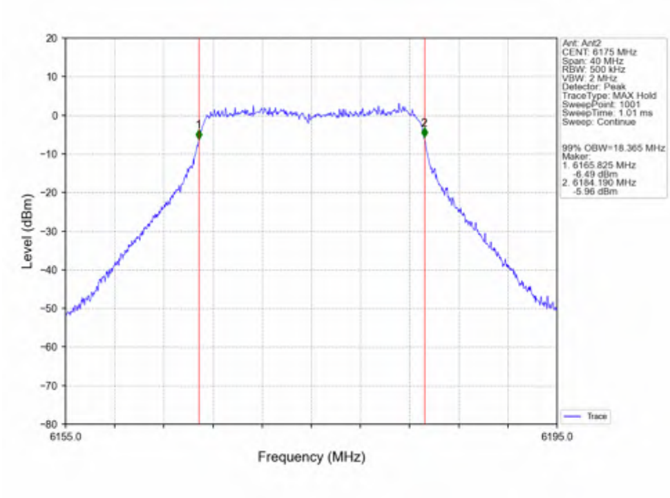
802.11ac(VHT20)_MCH_6175MHz_Ant2_NTNV
