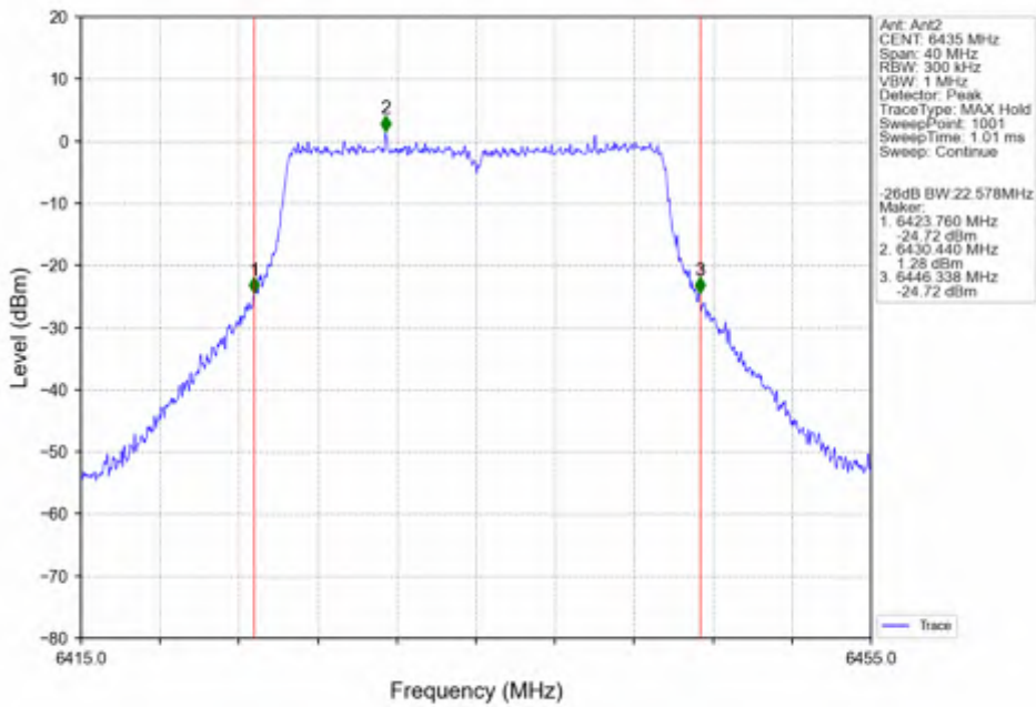
802.11ax(HEW20)_LCH_6435MHz_SU_ / Ant2_NTNV
