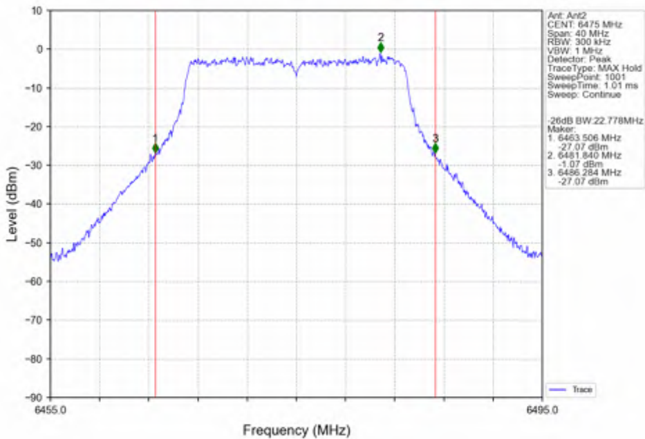
802.11ac(VHT20)_MCH_6475MHz_Ant2_NTNV
