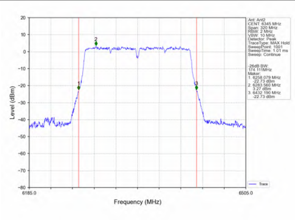
802.11ac(VHT160) HCH_6345MHz_Ant2_NTNV
