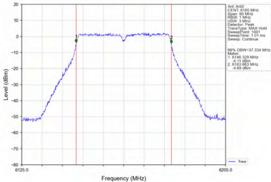
802.11ac(VHT40)_MCH_6165MHz_Ant2_NTNV
