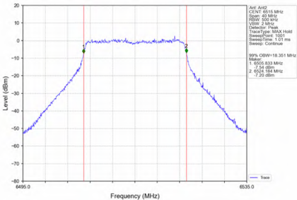
802.11ac(VHT20)_HCH_6515MHz_Ant2_NTNV
