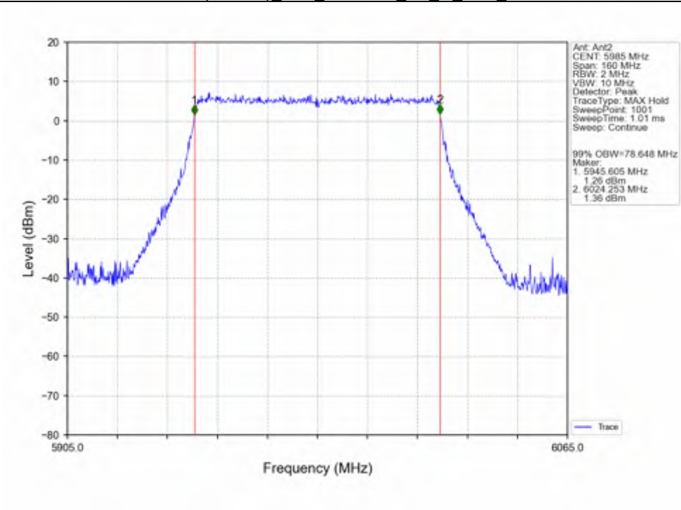
802.11ax(HEW80)_LCH_5985MHz_SU / Ant2_NTNV
