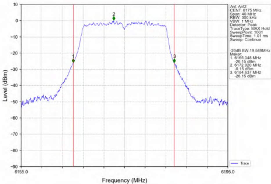
802.11a_MCH_6175MHz_Ant2_NTNV
