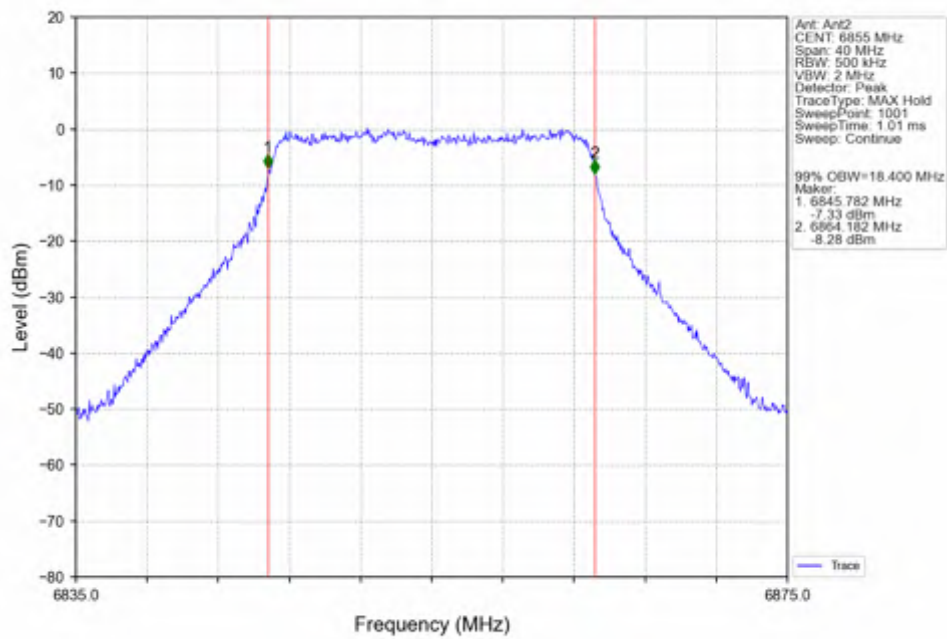
802.11ac(VHT20)_HCH_6855MHz_Ant2_NTNV
