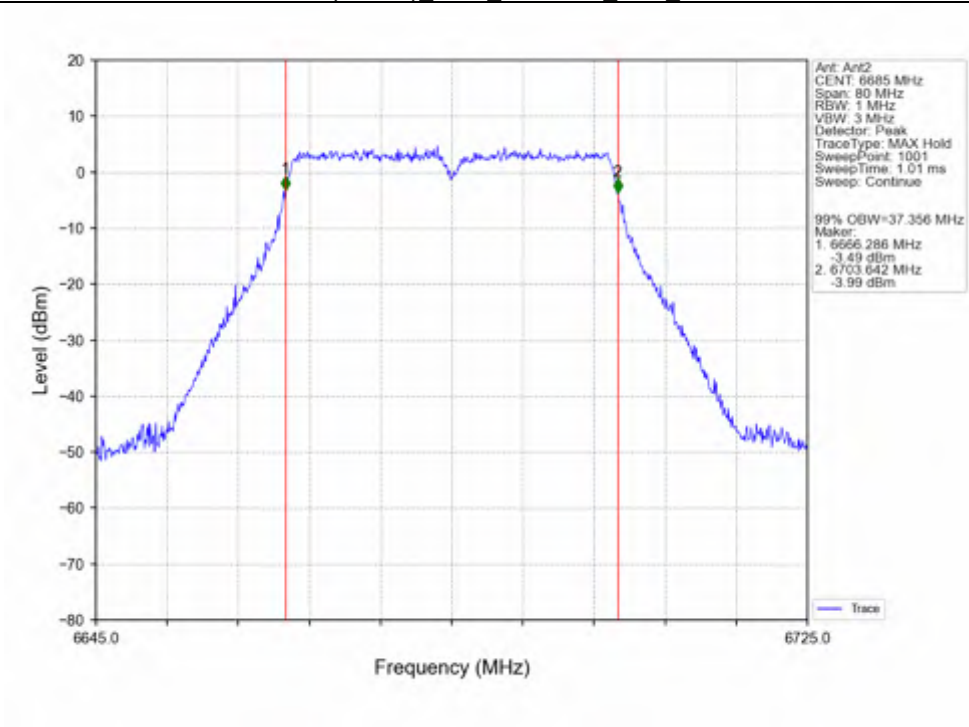
802.11ac(VHT40)_MCH_6685MHz_Ant2_NTNV
