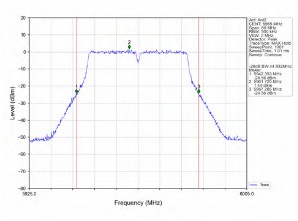
802.11n(HT40) LCH_5965MHz_Ant2_NTNV
