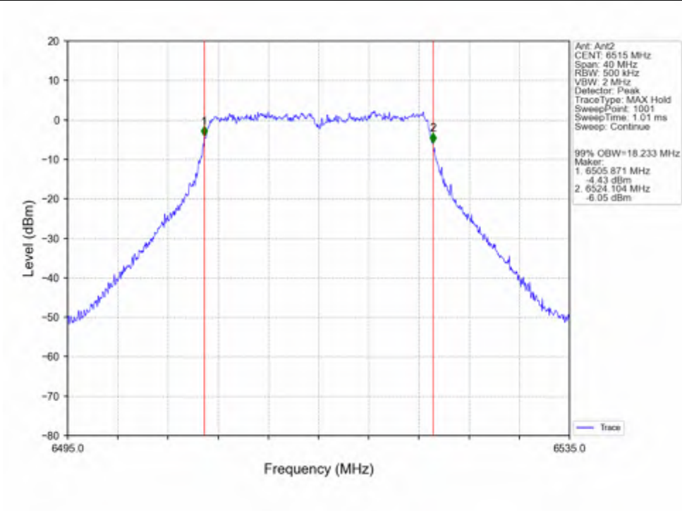
802.11n(HT20)_HCH_6515MHz_Ant2_NTNV
