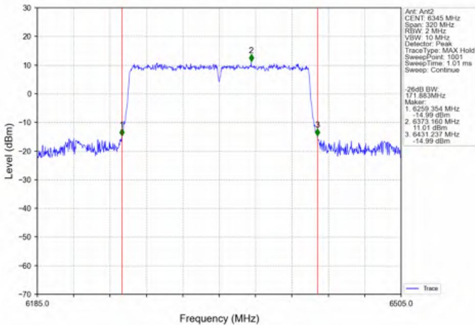
802.11ax(HEW160)_HCH_6345MHz_SU / Ant2_NTNV
