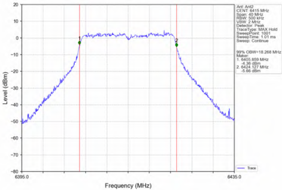
802.11n(HT20)_HCH_6415MHz_Ant2_NTNV
