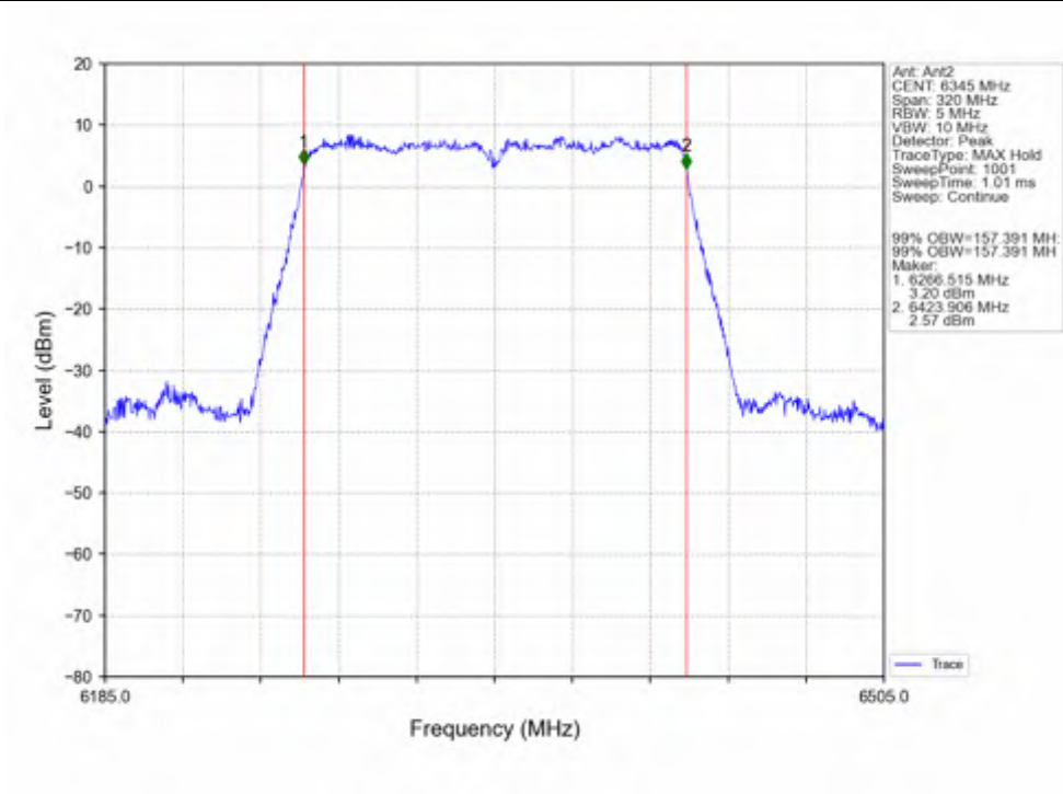
802.11ac(VHT160) HCH_6345MHz_Ant2_NTNV
