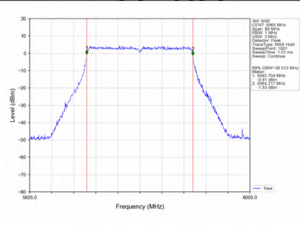
802.11ax(HEW40)_LCH_5965MHz_SU / Ant2_NTNV
