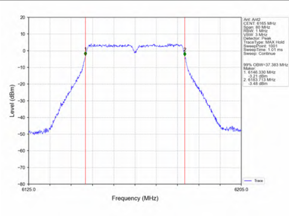
802.11n(HT40)_MCH_6165MHz_Ant2_NTNV
