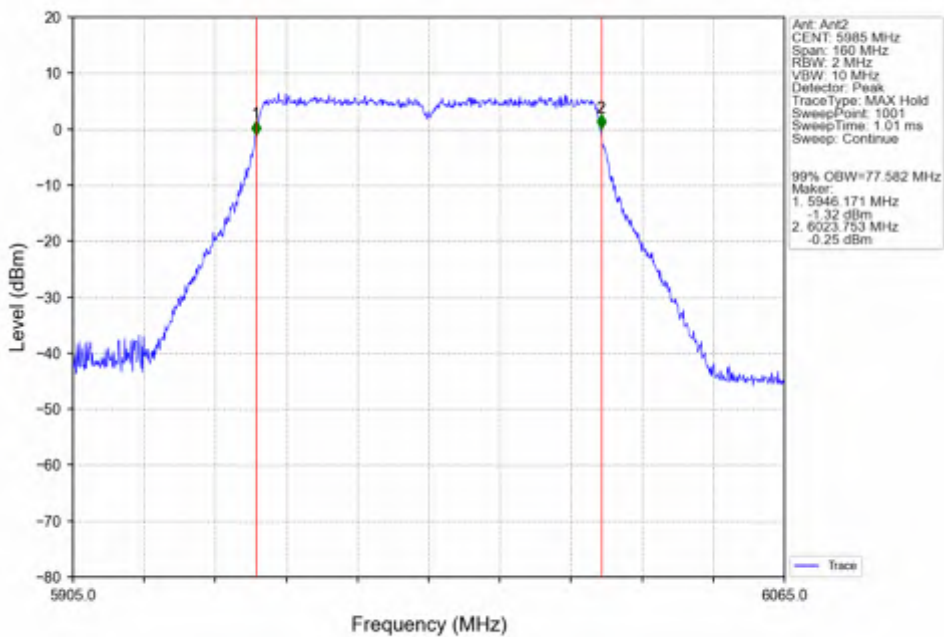
802.11ac(VHT80)_LCH_5985MHz_Ant2_NTNV
