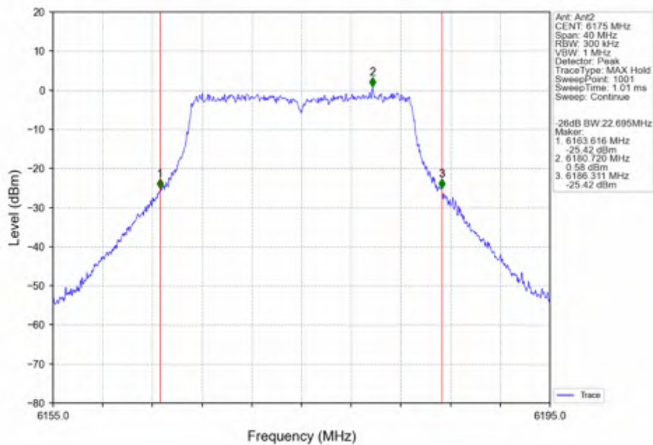
802.11ac(VHT20)_MCH_6175MHz_Ant2_NTNV
