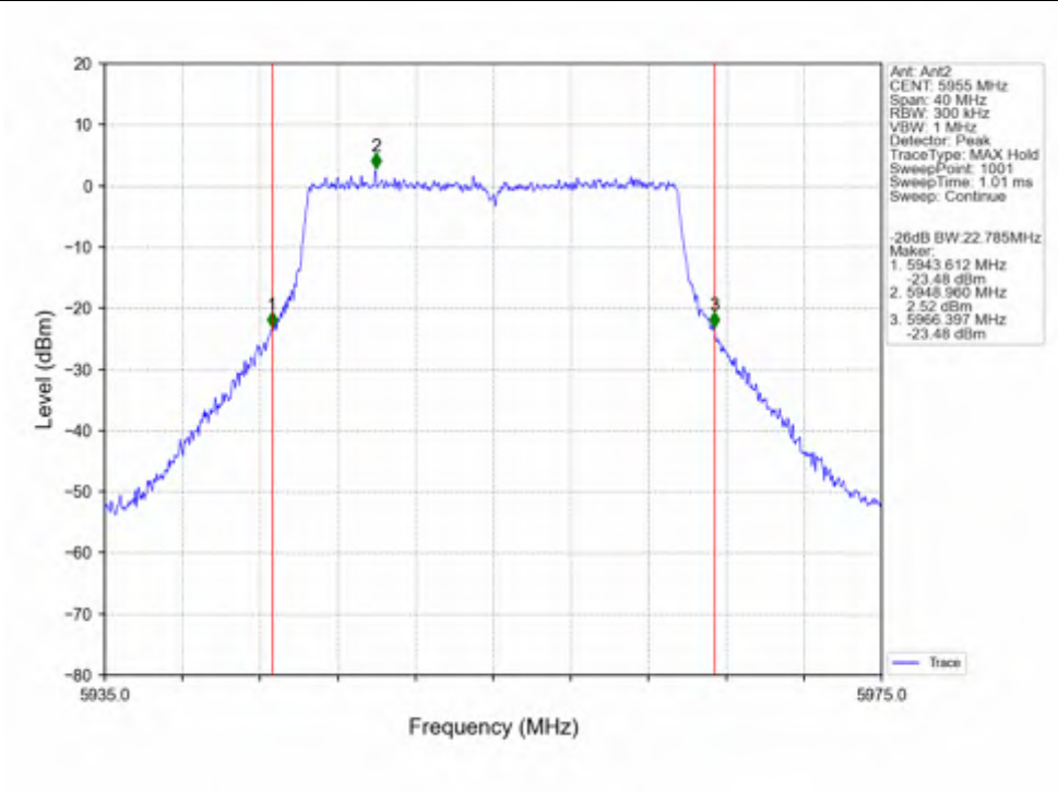
802.11ax(HEW20)_LCH_5955MHz_SU / Ant2_NTNV
