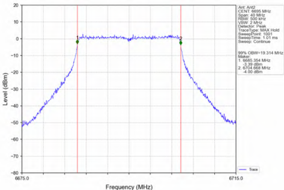
802.11ax(HEW20) MCH_6695MHz_SU / Ant2_NTNV
