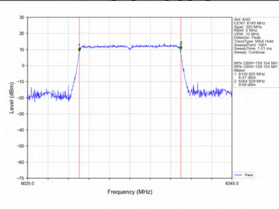
802.11ax(HEW160)_MCH_6185MHz_SU / Ant2_NTNV
