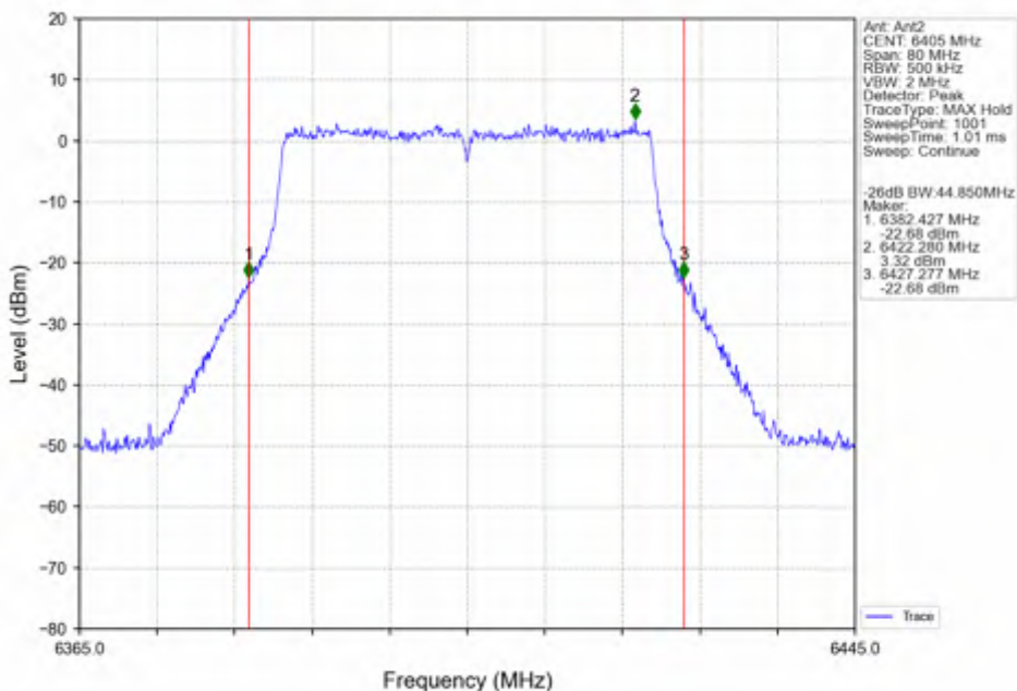
802.11ax(HEW40) HCH_6405MHz_SU / Ant2_NTNV
