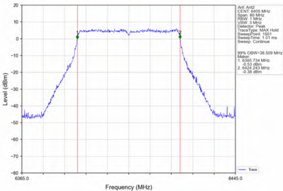
802.11ax(HEW40) HCH_6405MHz_SU / Ant2_NTNV
