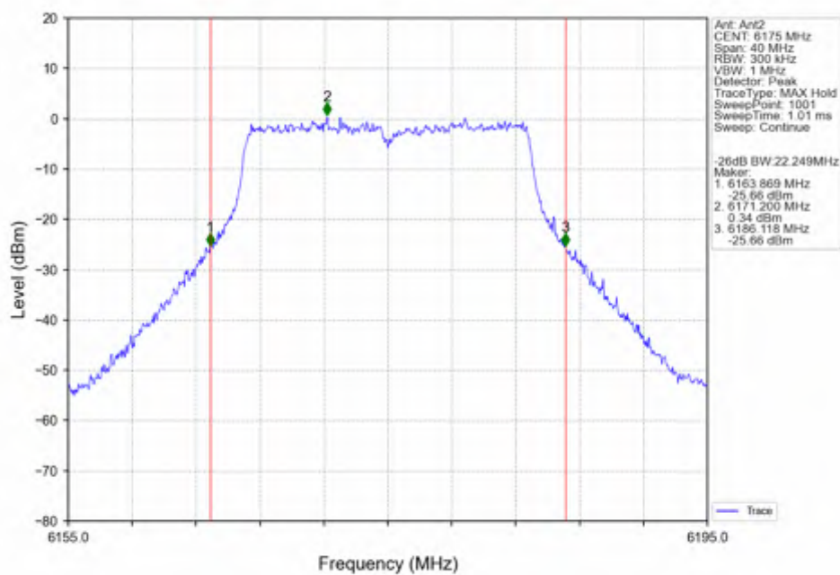
802.11n(HT20)_MCH_6175MHz_Ant2_NTNV
