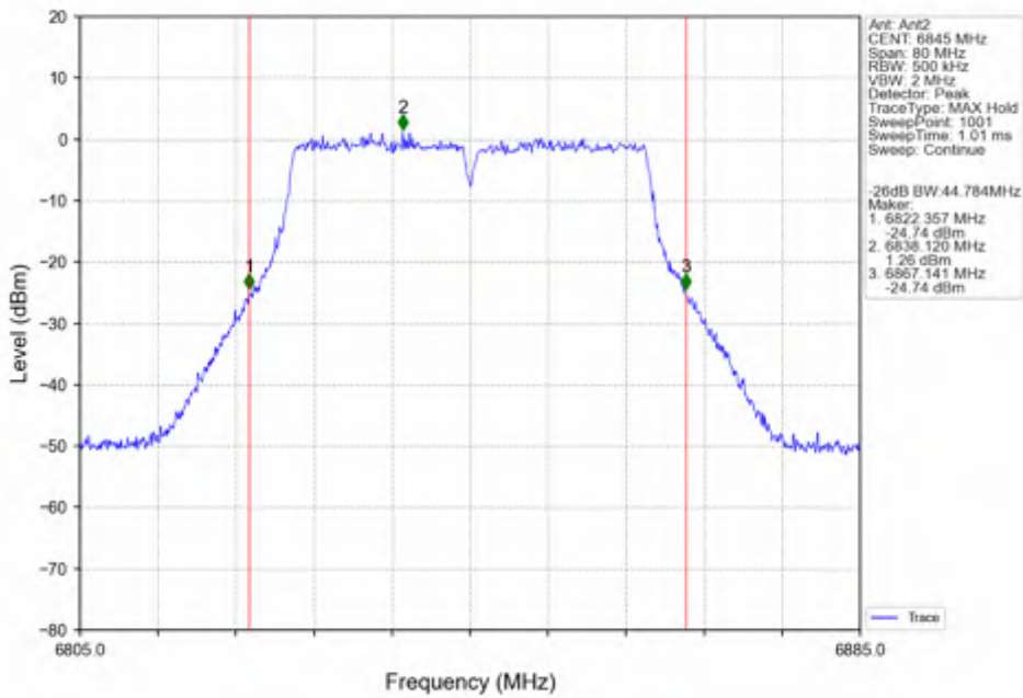
802.11n(HT40)_HCH_6845MHz_Ant2_NTNV
