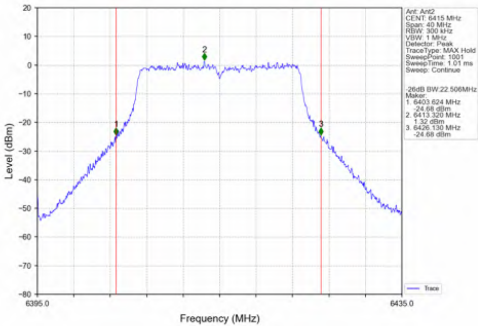
802.11n(HT20)_HCH_6415MHz_Ant2_NTNV
