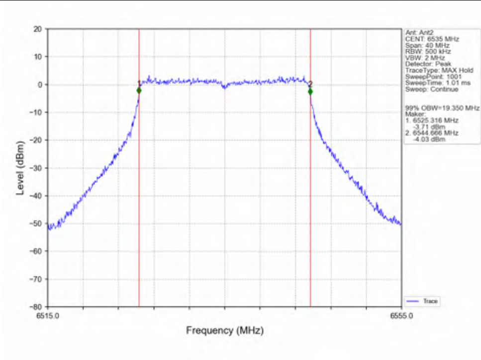
802.11ax(HEW20)_LCH_6535MHz_SU / Ant2_NTNV
