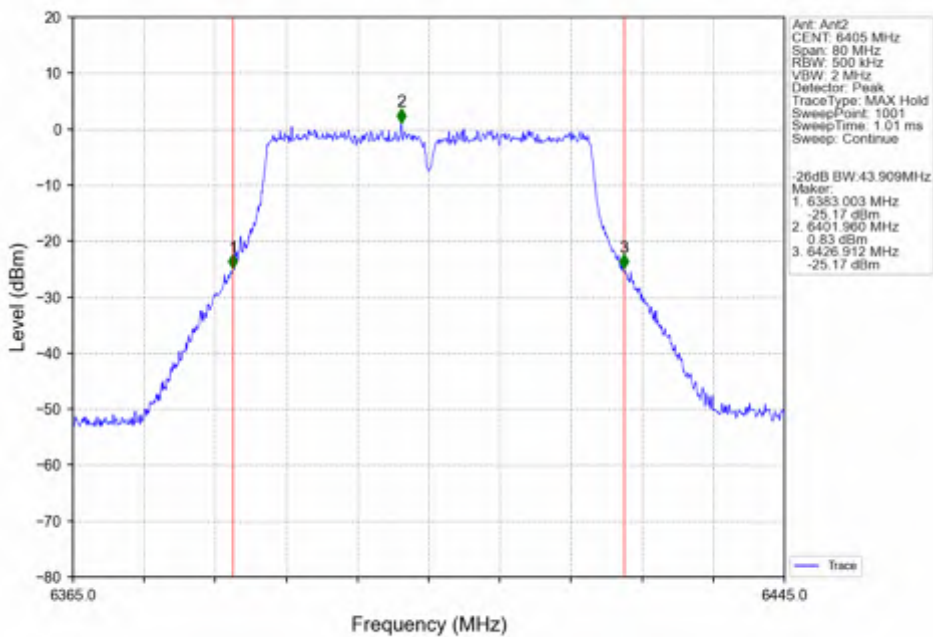
802.11ac(VHT40)_HCH_6405MHz_Ant2_NTNV
