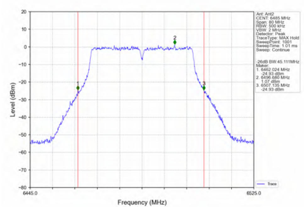
802.11ac(VHT40)_MCH_6485MHz_Ant2_NTNV
