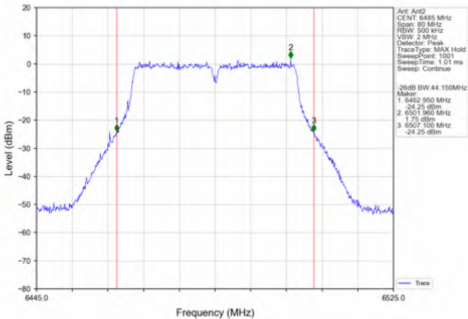
802.11n(HT40)_MCH_6485MHz_Ant2_NTNV
