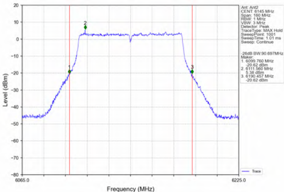
802.11ac(VHT80)_MCH_6145MHz_Ant2_NTNV
