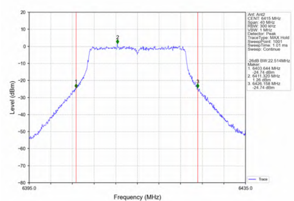
802.11ac(VHT20)_HCH_6415MHz_Ant2_NTNV
