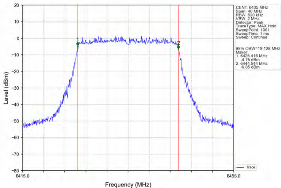
802.11ax(HEW20)_LCH_6435MHz_SU / Ant2_NTNV
