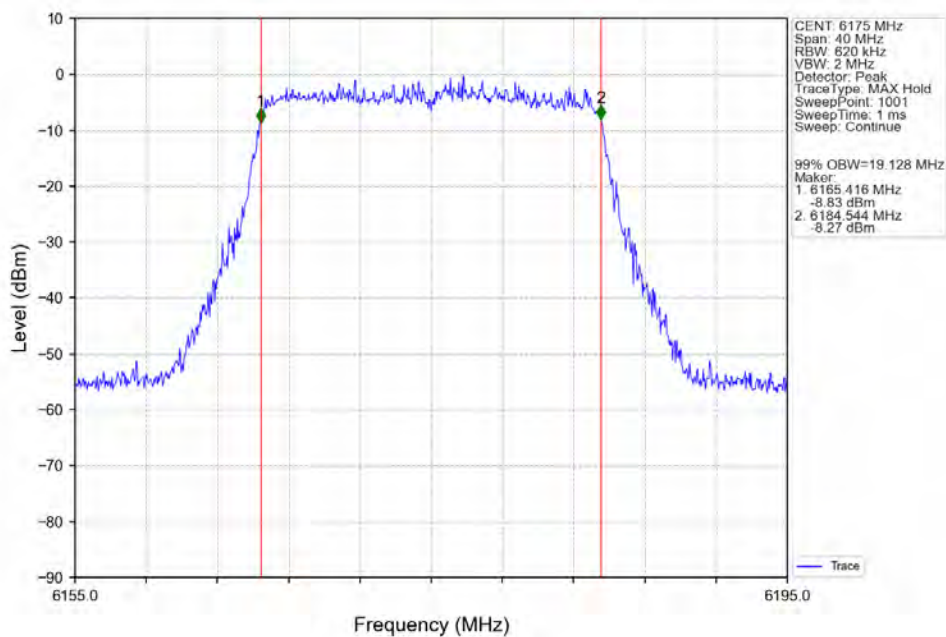
802.11ax(HEW20)_MCH_6175MHz_SU / Ant2_NTNV
