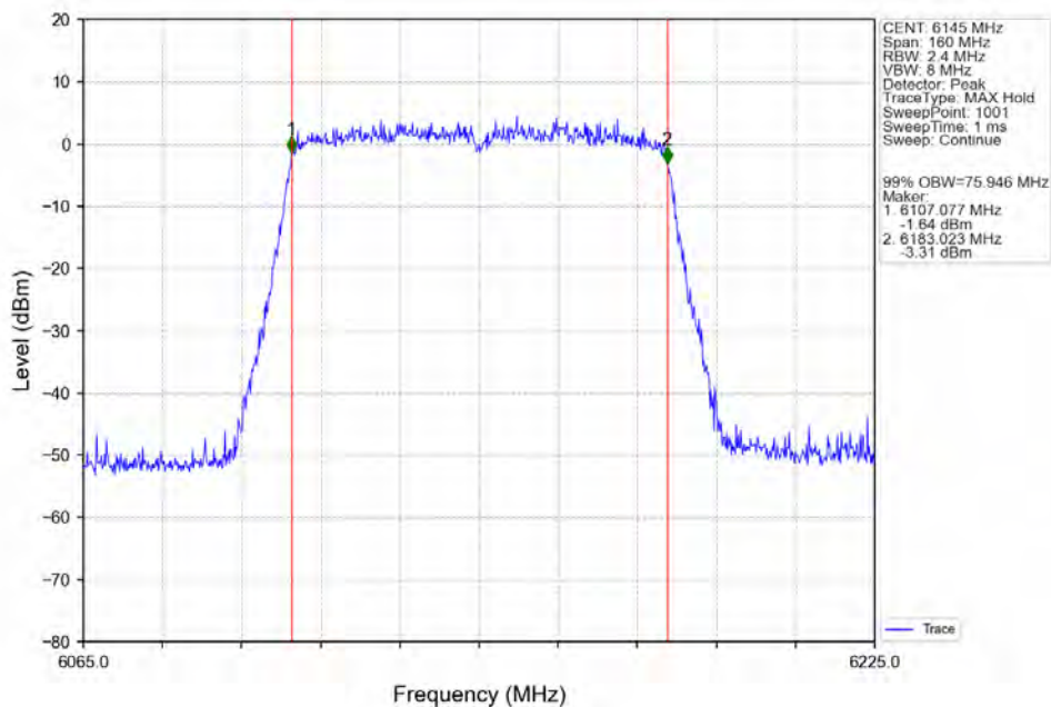
802.11ac(VHT80)_MCH_6145MHz_Ant2_NTNV
