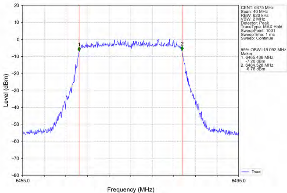
802.11ax(HEW20)_MCH_6475MHz_SU / Ant2_NTNV
