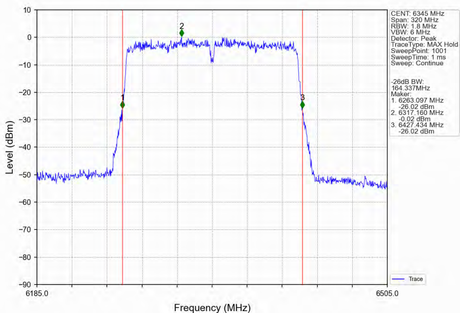
802.11ac(VHT160) HCH 6345MHz Ant2_NTNV
