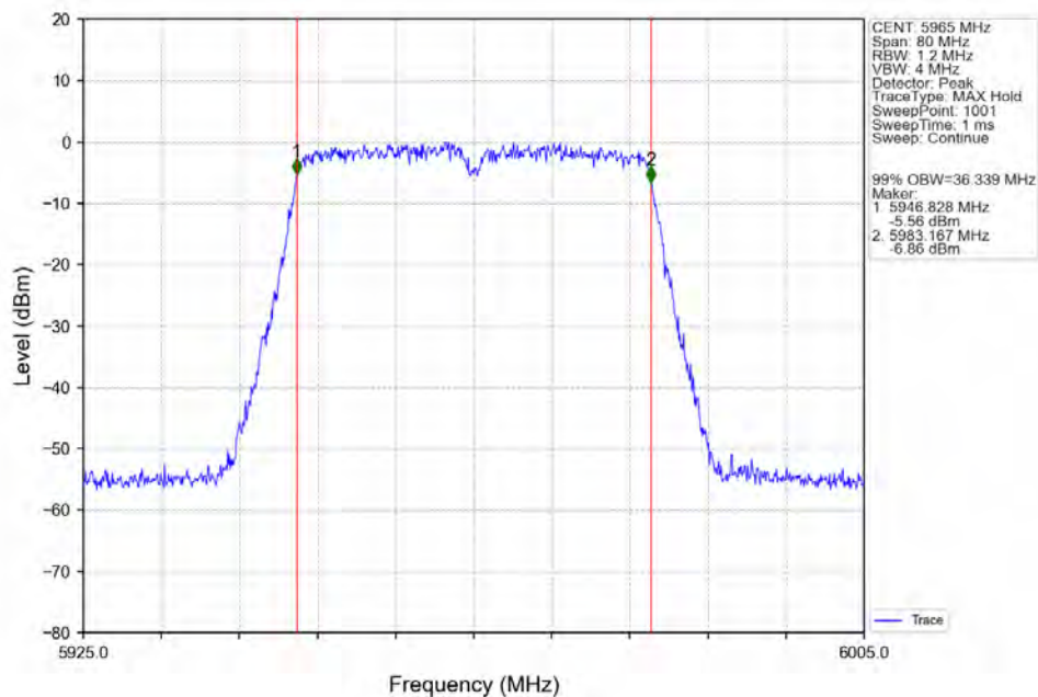
802.11n(HT40) LCH_5965MHz_Ant2_NTNV
