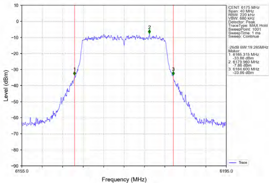
802.11a_MCH_6175MHz_Ant2_NTNV
