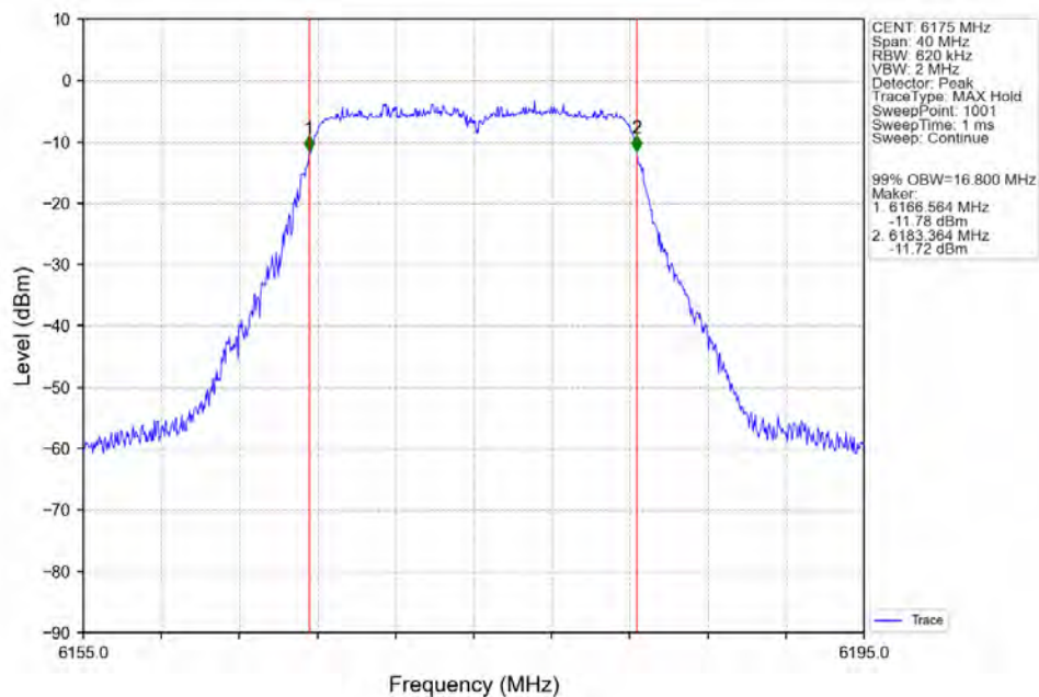
802.11a_MCH_6175MHz_Ant2_NTNV
