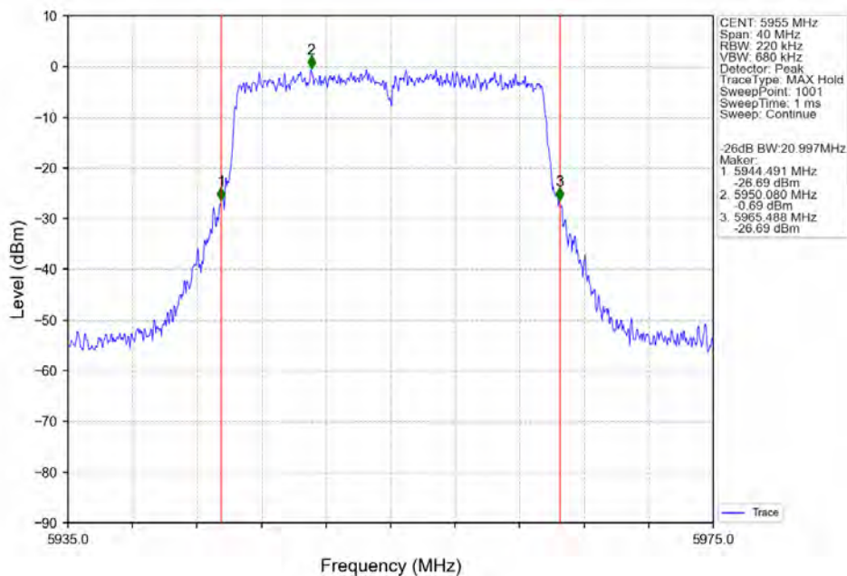
802.11ax(HEW20)_LCH_5955MHz_SU / Ant2_NTNV
