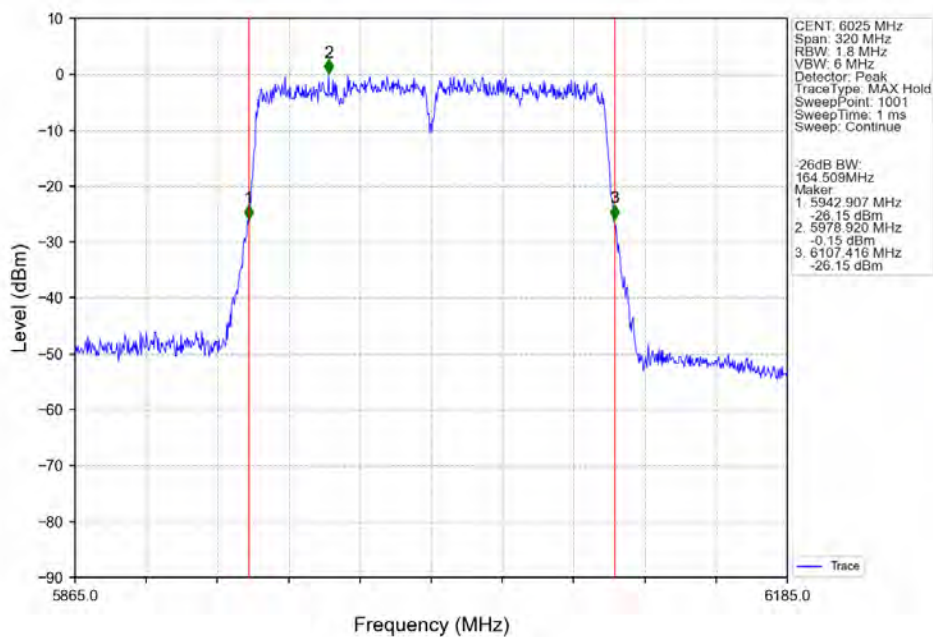
802.11ac(VHT160) LCH_6025MHz_Ant2_NTNV
