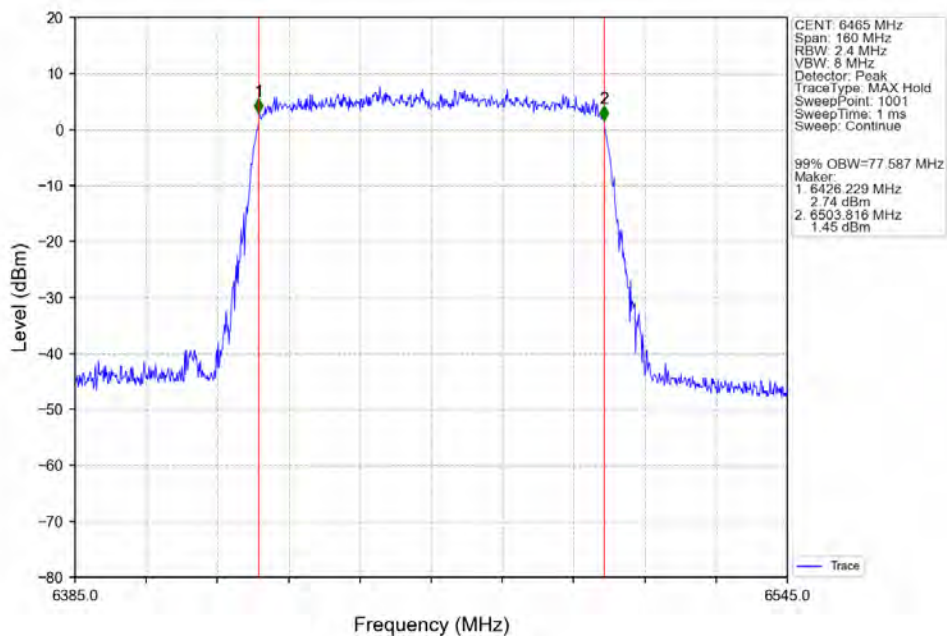
802.11ax(HEW80)_LCH_6465MHz_SU / Ant2_NTNV
