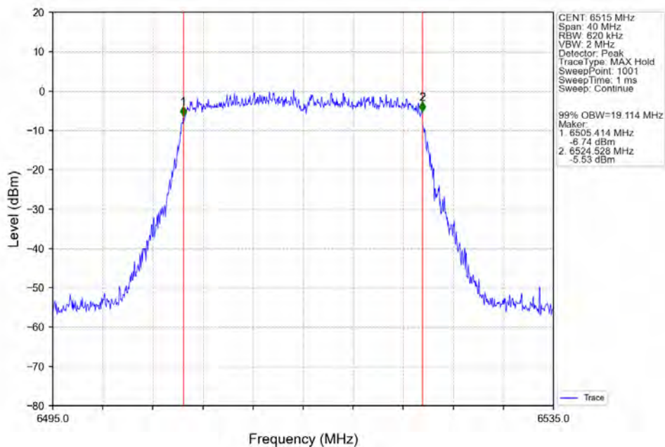
802.11ax(HEW20)_HCH_6515MHz_SU / Ant2_NTNV
