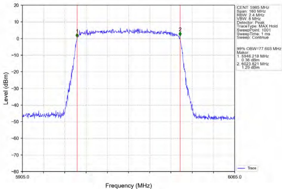
802.11ax(HEW80)_LCH_5985MHz_SU / Ant2_NTNV
