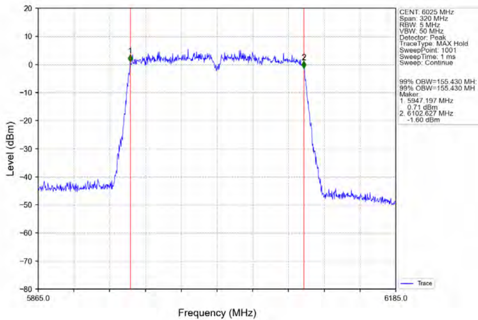
802.11ac(VHT160) LCH_6025MHz_Ant2_NTNV
