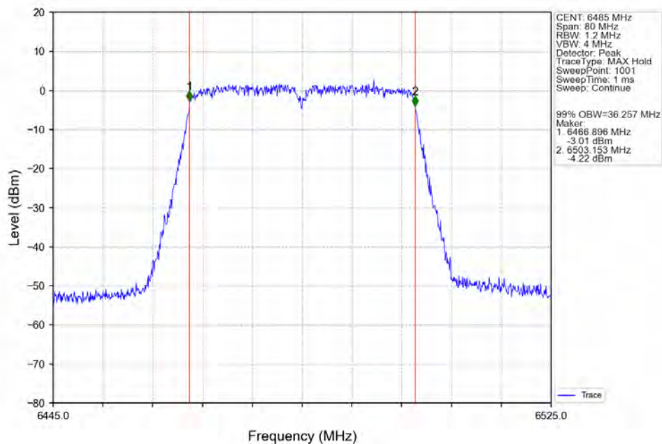
802.11ac(VHT40)_MCH_6485MHz_Ant2_NTNV
