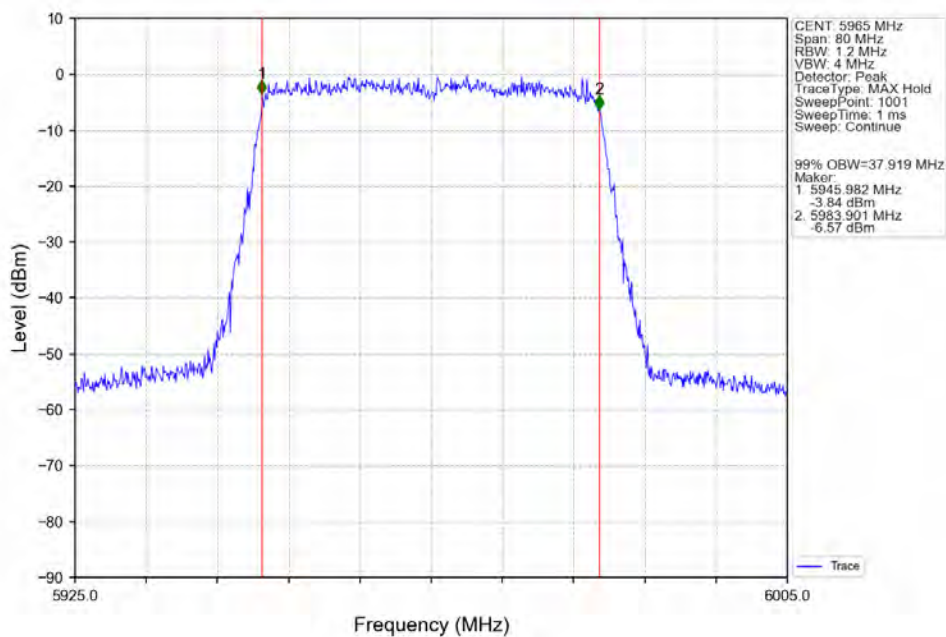
802.11ax(HEW40)_LCH_5965MHz_SU / Ant2_NTNV
