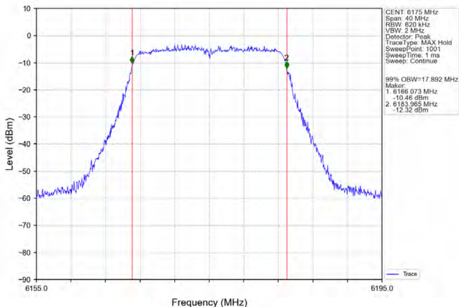
802.11n(HT20)_MCH_6175MHz_Ant2_NTNV
