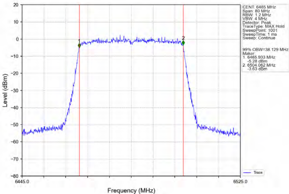
802.11ax(HEW40) MCH_6485MHz_SU / Ant2_NTNV
