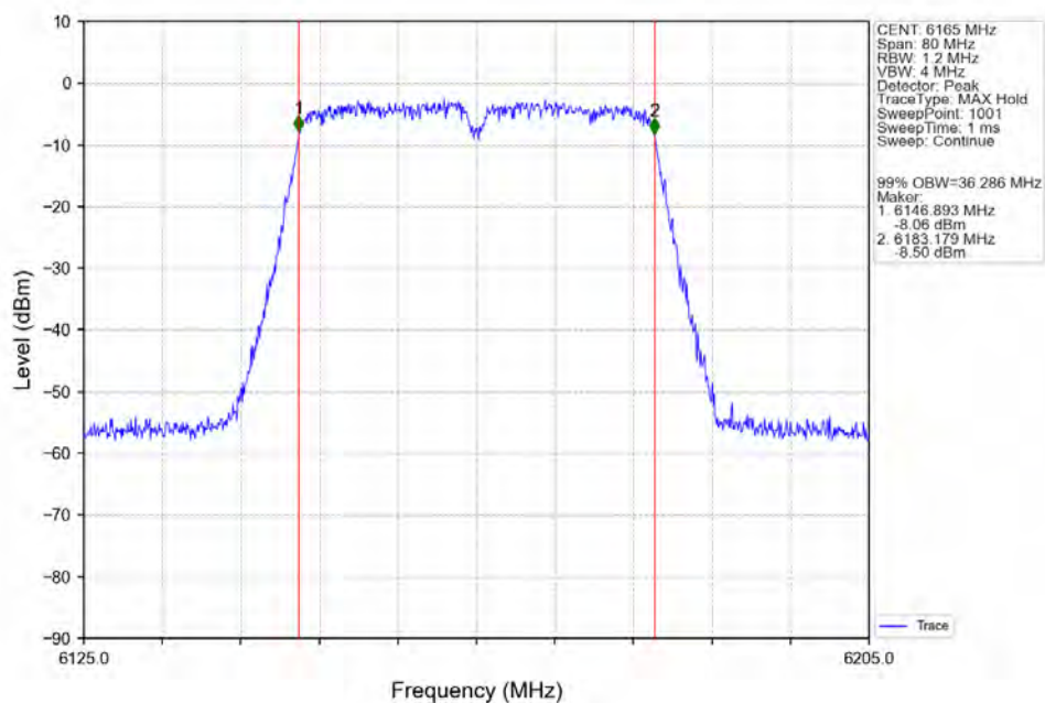
802.11ac(VHT40)_MCH_6165MHz_Ant2_NTNV
